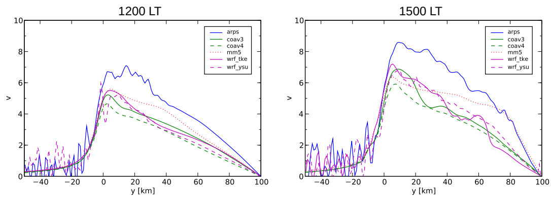
Figure 10: As in Figure 9, but for the uncoupled simulations.
