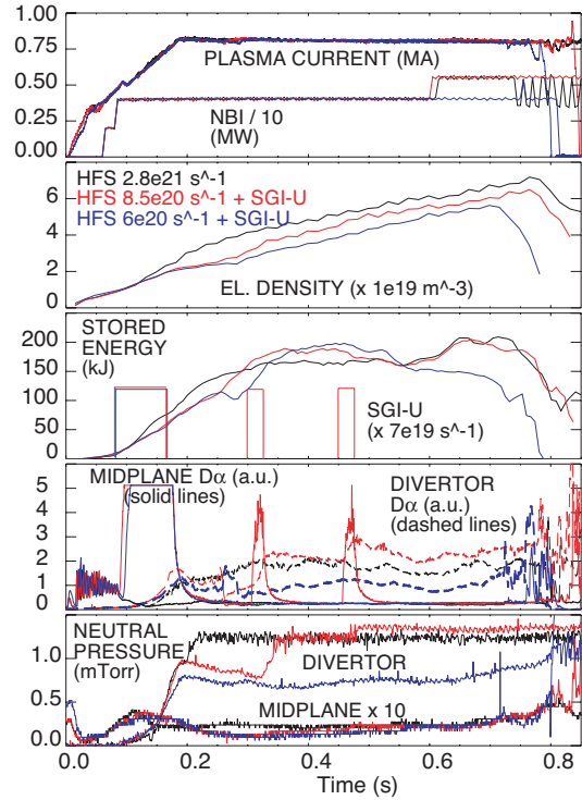
Figure 3: Waveforms of three H-mode discharges fueled by 1/ HFS injector only, 2/ reduced HFS injector rate and three SGI-U pulses, 3/ reduced HFS injector rate and one SGI-U pulse.
