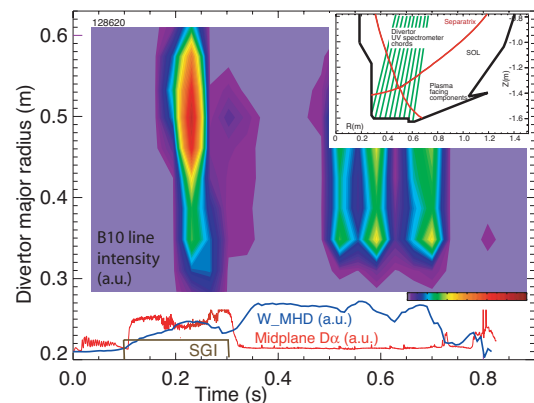
Figure 4: Spectroscopic evidence of X-point MARFE formation during SGI-U gas pulse.
