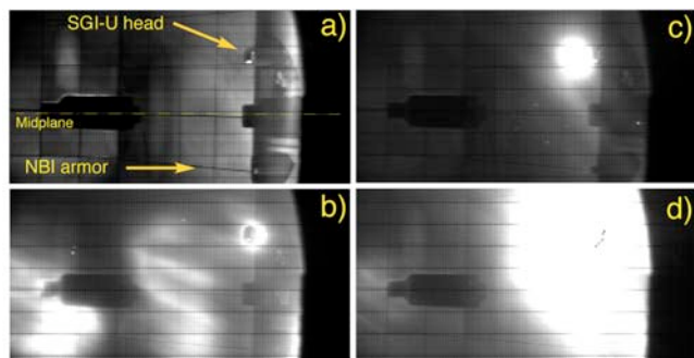
Figure 1: Fast camera images of jet-plasma interaction: (a) SGI-U head in the vacuum vessel at R = 1.57 \text{ m} , (b) Plasma interaction with SGI-U head during an MHD event, (c) D_\alpha emission from jet in the initial phase of high-pressure injection, (d) D_\alpha emission during high-pressure injection.
