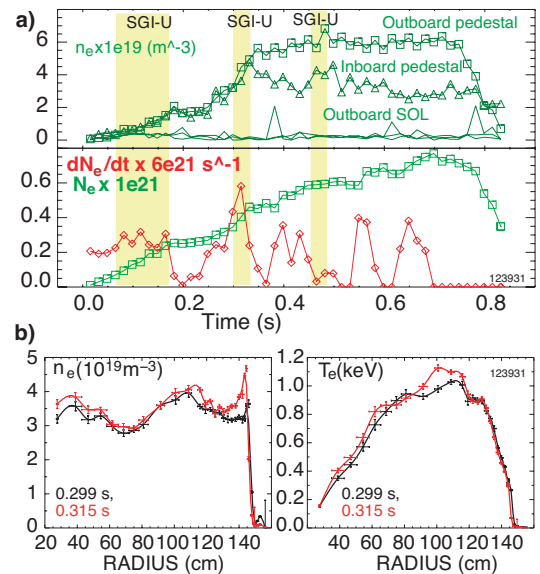
Figure 2: (a) Density waveforms of an H-mode discharge, with SGI-U injection shown by yellow bars; (b) n_e, T_e profiles just before and during the SGI-U pulse at 0.3 s.
