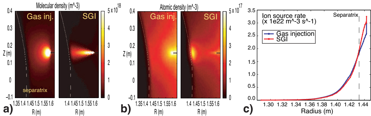
Figure 5: DEGAS 2 simulations of the conventional and supersonic gas injections in the H-mode plasmas: (a) molecular, (b) atomic densities, (c) flux surface averaged ionization rates. An artificial elongation 2:1 was given to panels (a) and (b) for clarity.
