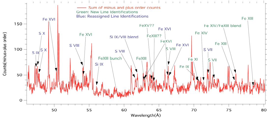
FIGURE 1: Co-added LETG spectra of Procyon (in red) between 48 -80 Å with previously unidentified lines (green) and reassigned lines (blue). We have reassigned some of the lines previously identified by Raassen, et al (2002). Two observations of Procyon were summed and the plus and minus orders were co-added and binned by 2 to get better signal to noise. Several new tentative identifications of Fe IX-XIV have been made for the first time and many lines have been reassigned to other ions. Laboratory measurements were carried out at densities relevant to stellar coronae and at voltages necessary to produce the L and M shell spectra of these astrophysically abundant elements. Note that some of these identifications are preliminary, as the laboratory data are not published yet.
