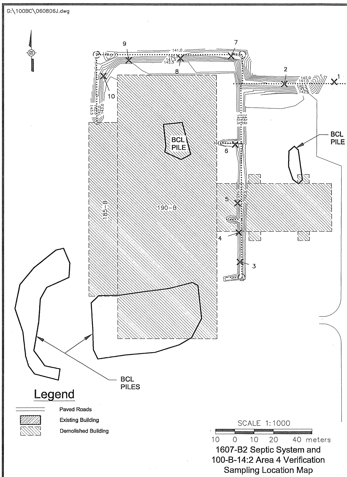
Figure 11. Statistical Verification Sampling Locations at the 100-B-14:2 (Area 4) Subsite.
