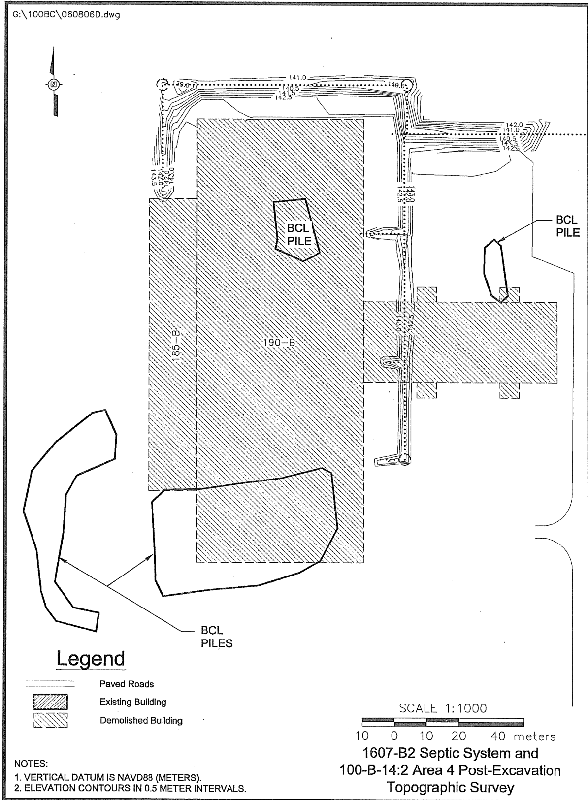
Figure 5. Post-Excavation Civil Survey of the 100-B-14:2 (Area 4) Subsite.
