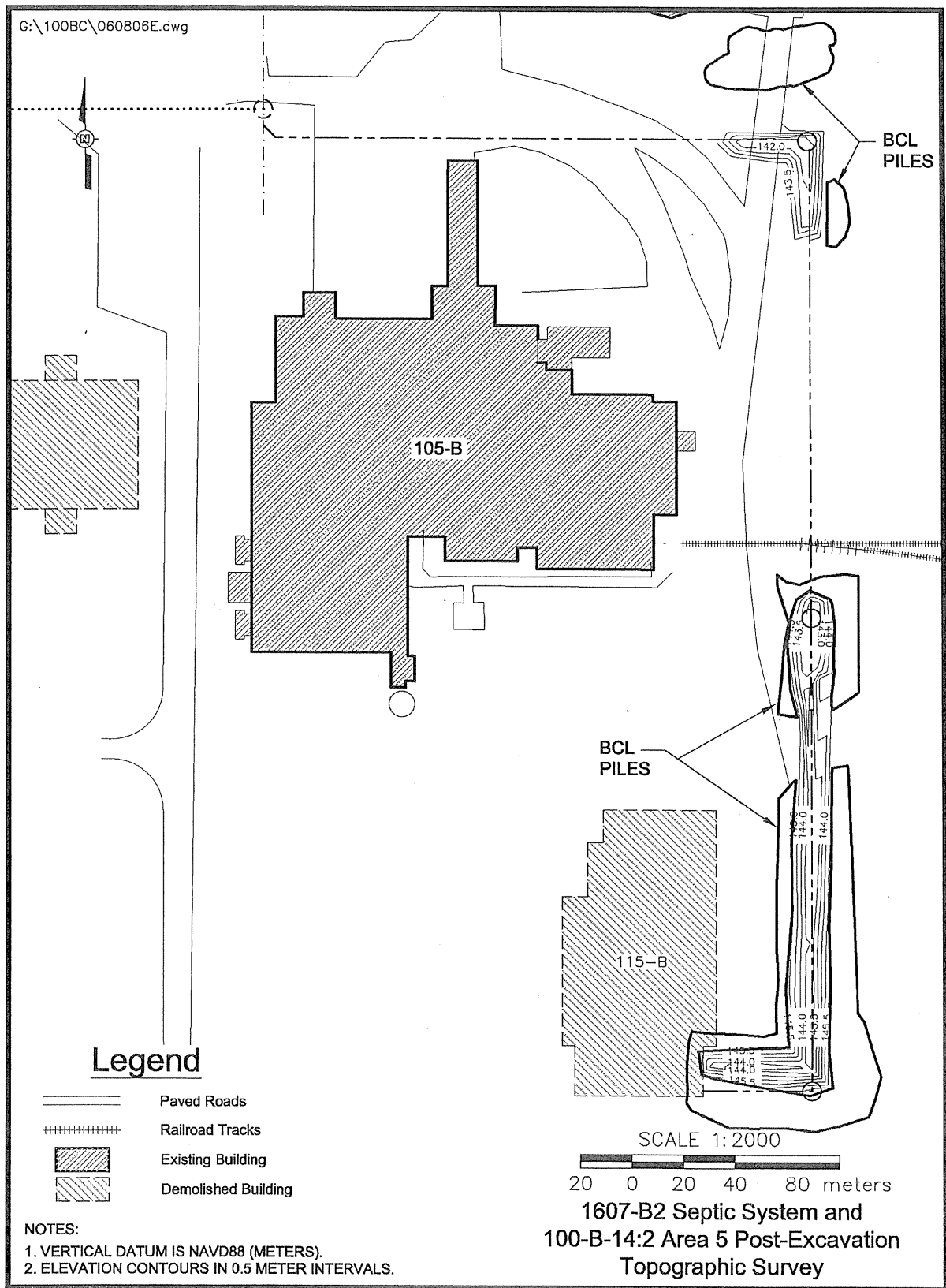
Figure 6. Post-Excavation Civil Survey of the 100-B-14:2 (Area 5) Subsite.
