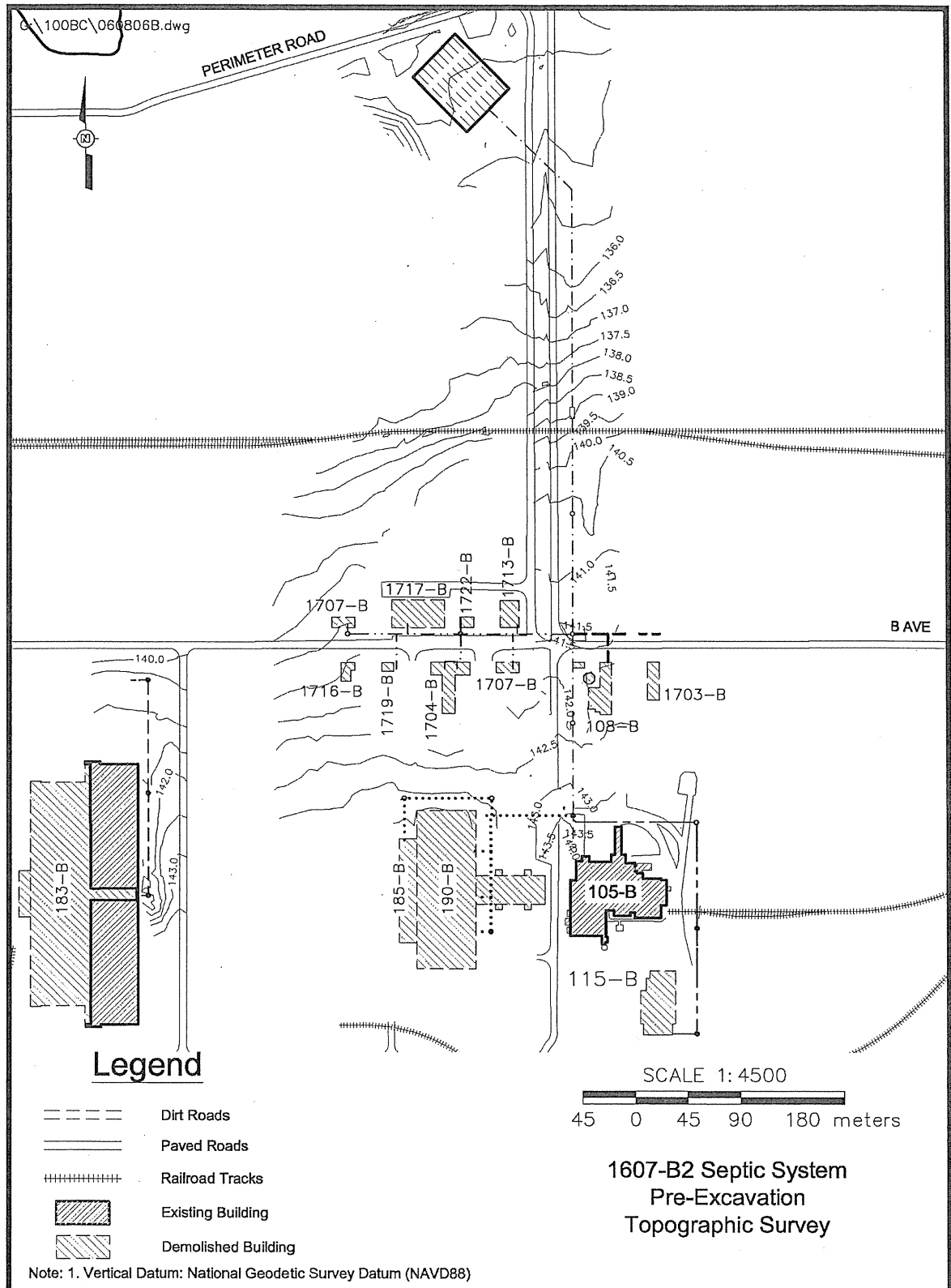
Figure 3. Pre-Excavation Topographic Survey of the 100-B-14:2 and 1607-B2 Waste Site Vicinity.
