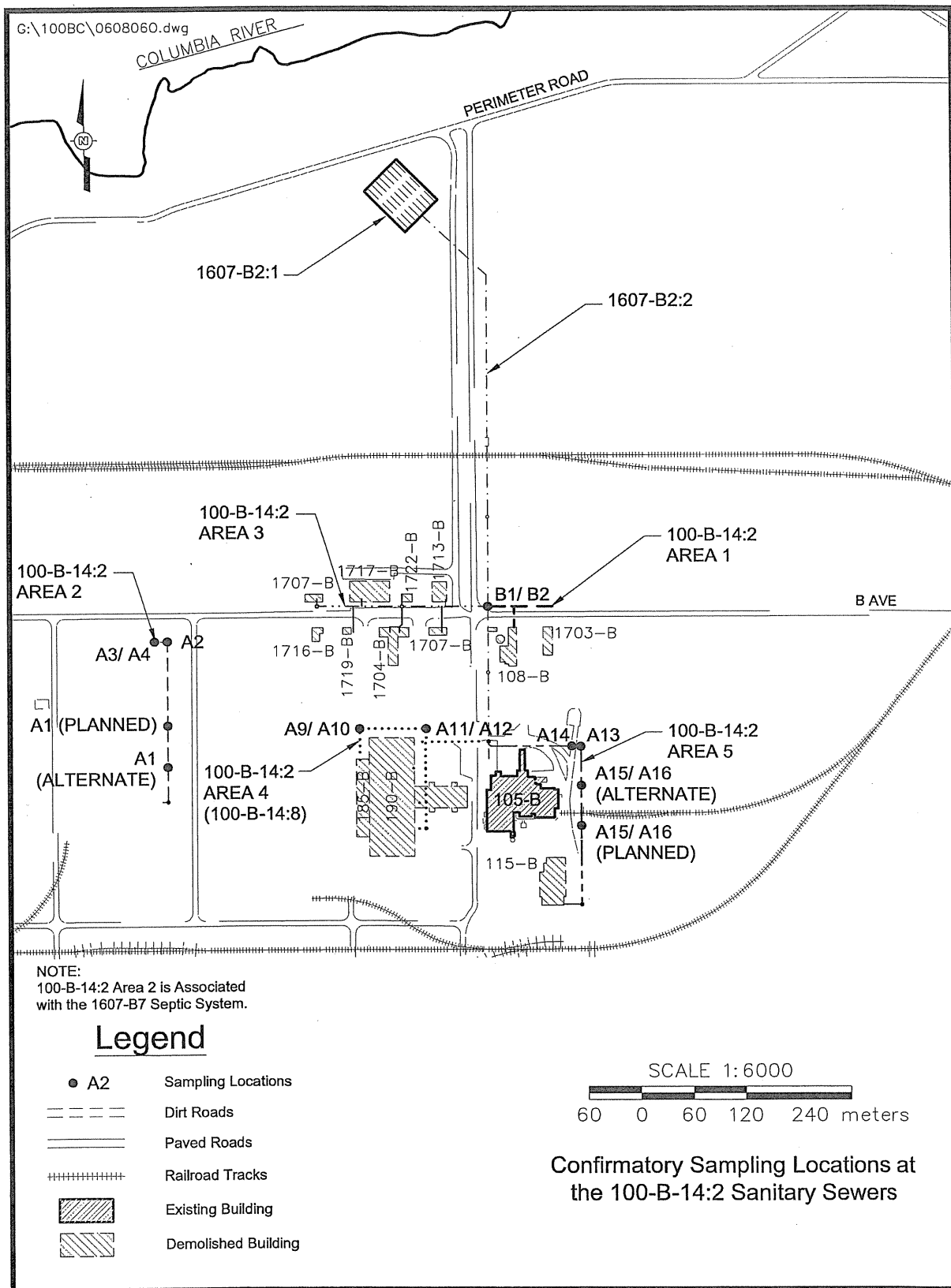
Figure 2. Confirmatory Sampling Locations at the 100-B-14:2 Subsite.
