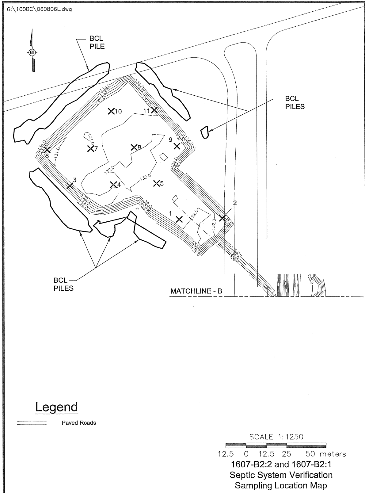
Figure 15. Statistical Verification Sampling Locations at the 1607-B2:1 Subsite.
