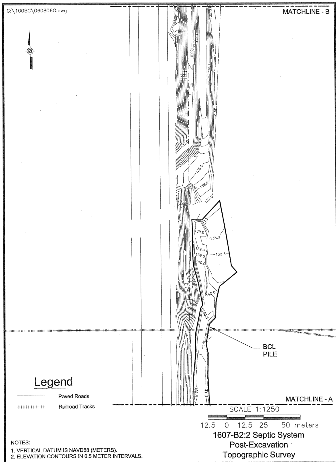
Figure 8. Post-Excavation Civil Survey of the Northern 1607-B2:2 Subsite.
