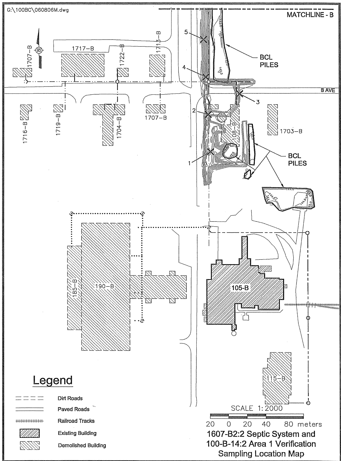
Figure 13. Statistical Verification Sampling Locations at the Southern 1607-B2:2 Subsite and 100-B-14:2 (Area 1) Subsite.
