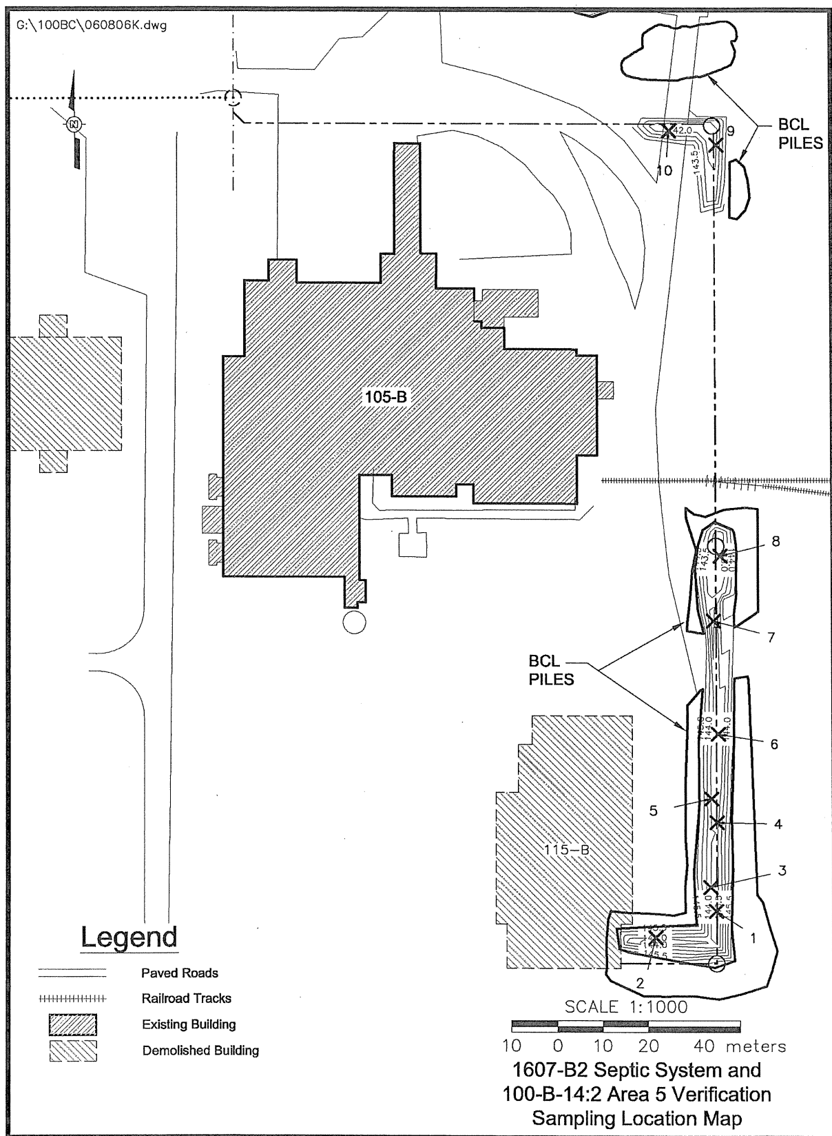
Figure 12. Statistical Verification Sampling Locations at the 100-B-14:2 (Area 5) Subsite.
