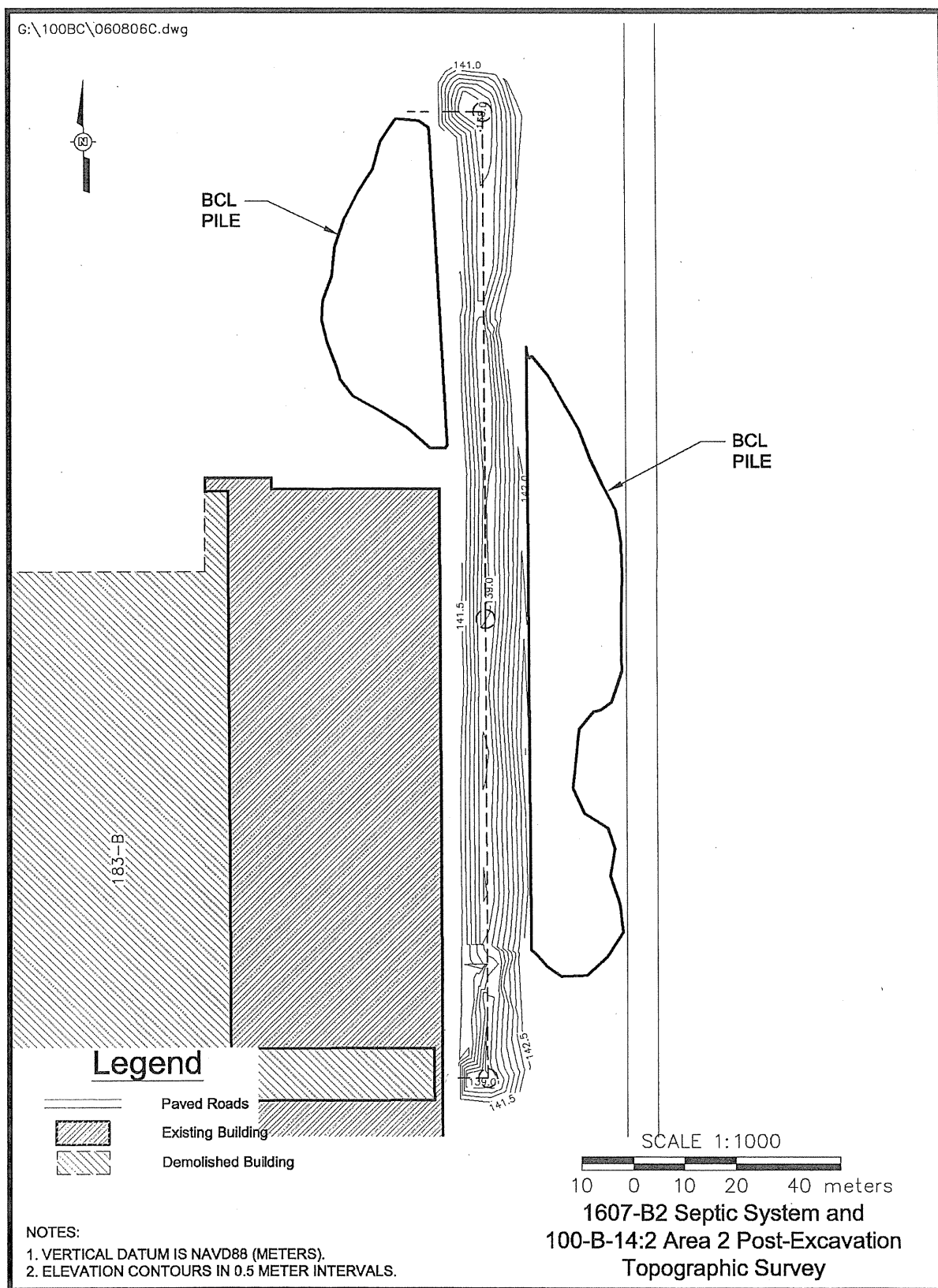
Figure 4. Post-Excavation Civil Survey of the 100-B-14:2 (Area 2) Subsite.
