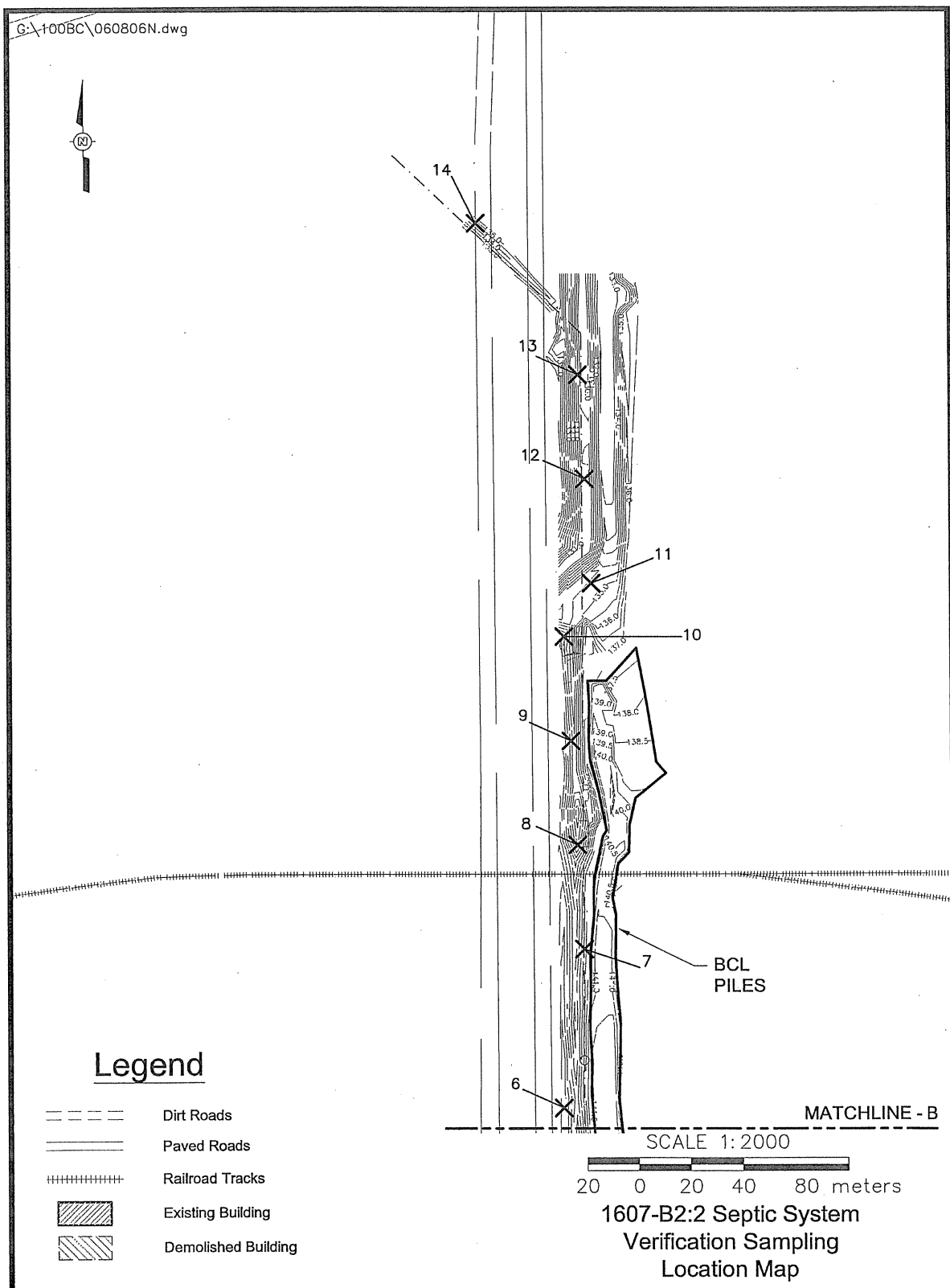
Figure 14. Statistical Verification Sampling Locations at the Northern 1607-B2:2 Subsite.
