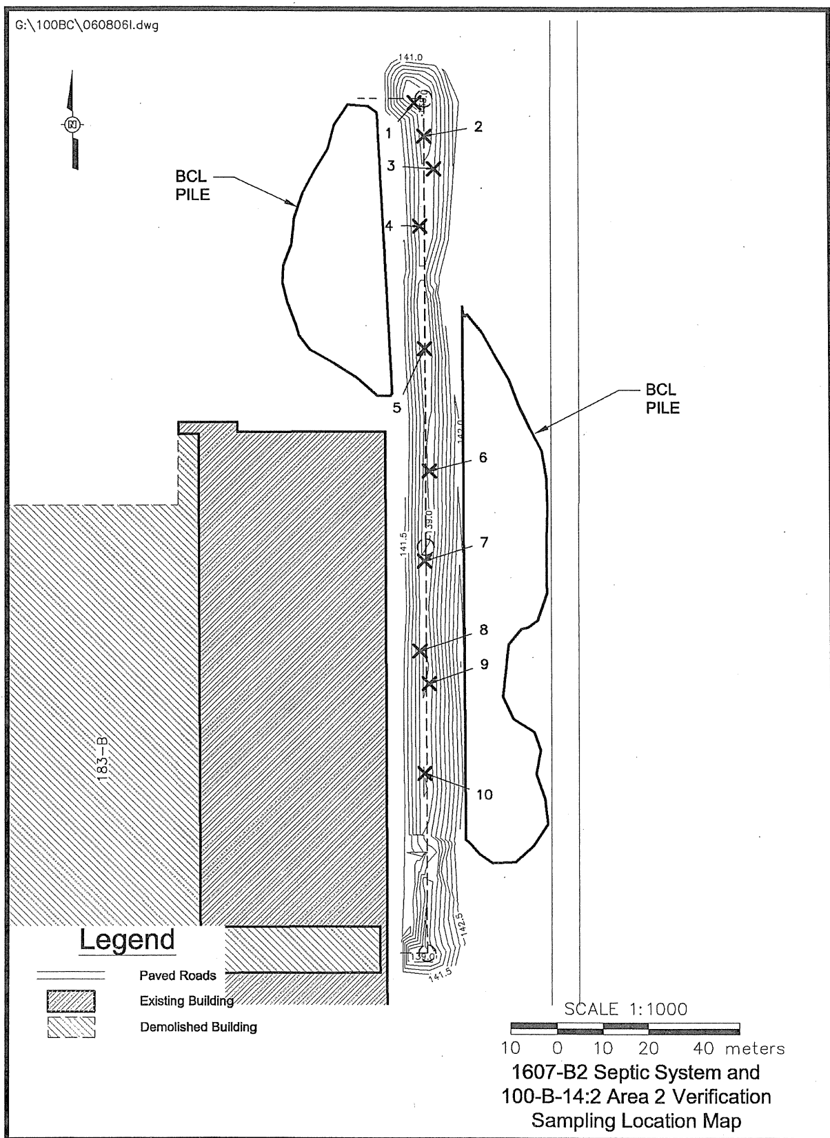
Figure 10. Statistical Verification Sampling Locations at the 100-B-14:2 (Area 2) Subsite.
