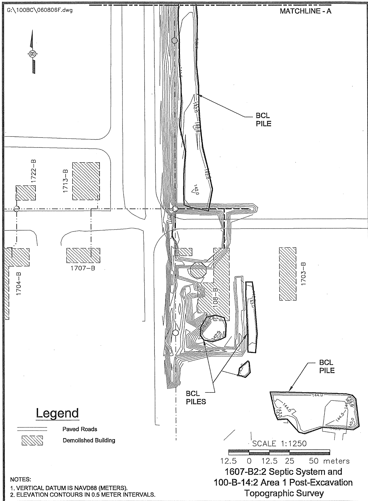
Figure 7. Post-Excavation Civil Survey of the Southern 1607-B2:2 Subsite and 100-B-14:2 (Area 1) Subsite.
