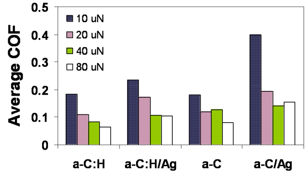
Fig. 3 The average COF of the four samples with different normal loads.
