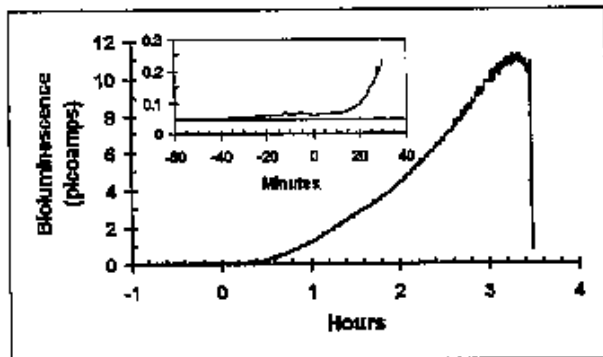
Fig. 3. Bioluminescence from a growing culture of P. fluorescens 5RL as measured by the microluminometer. At time = 0, salicylate (1 ppm) was used to fully induce the lux genes. The bioluminescence level increased for ~ 3.5 hours until the bioluminescent reaction became oxygen limited at a cell population of 1.53 \times 10^8 .
