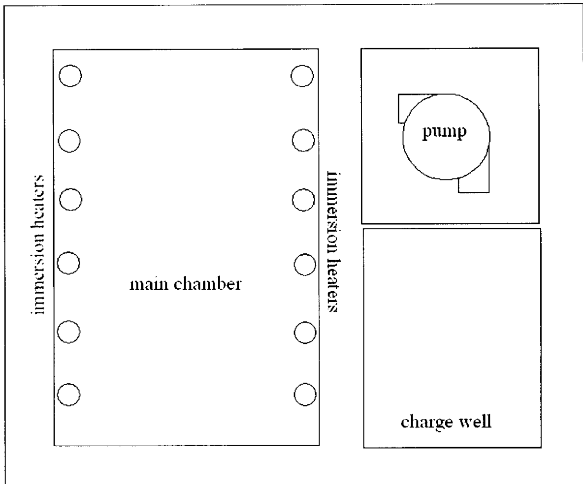
Figure 2: Concept of possible conversion of the generic sidewell aluminum melter in figure 1 to an immersed tube melter. All dimensions remain the same as in figure 1.
