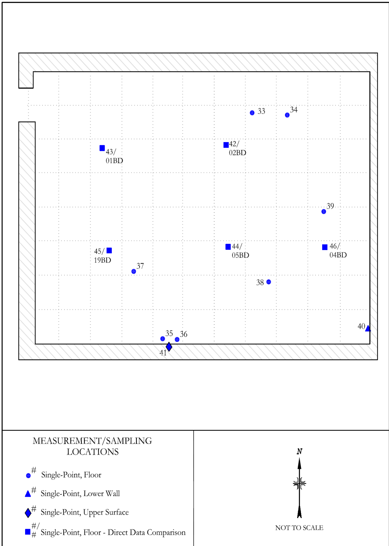
FIGURE 5: Auxiliary Building, Room 25 - Direct Measurement Locations
