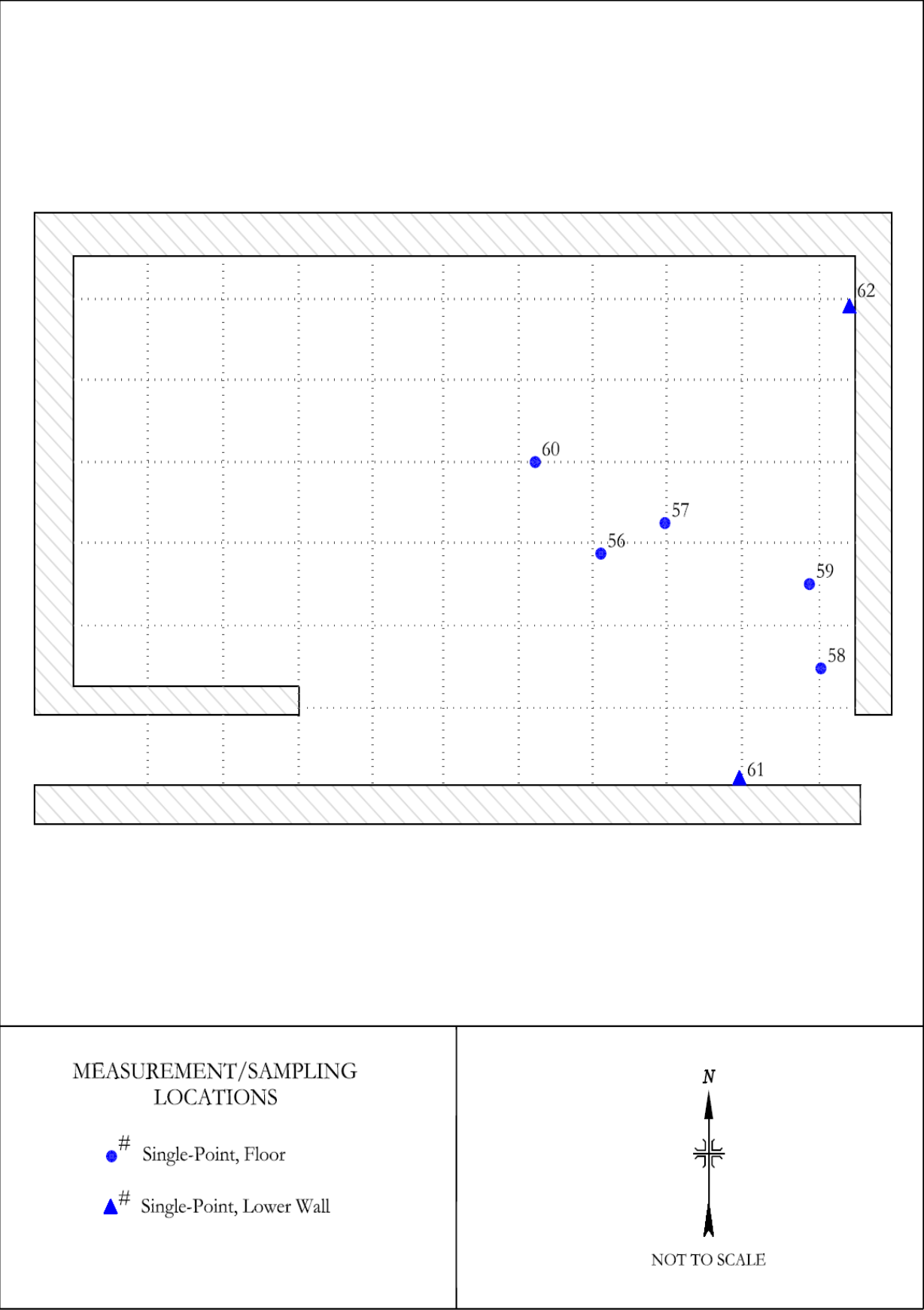
FIGURE 3: Auxiliary Building, Room 23 - Direct Measurement Locations
