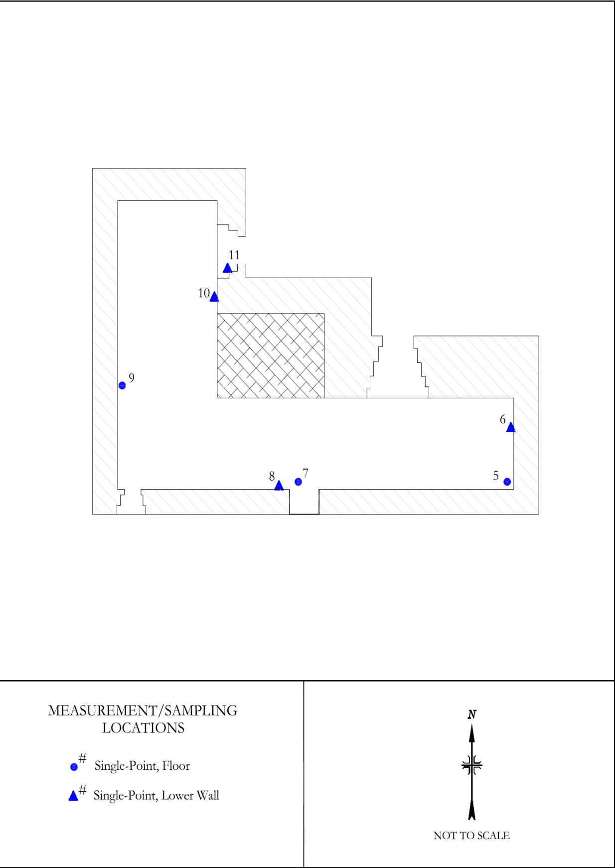
FIGURE 9: Auxiliary Building, Room 46 - Direct Measurement Locations
