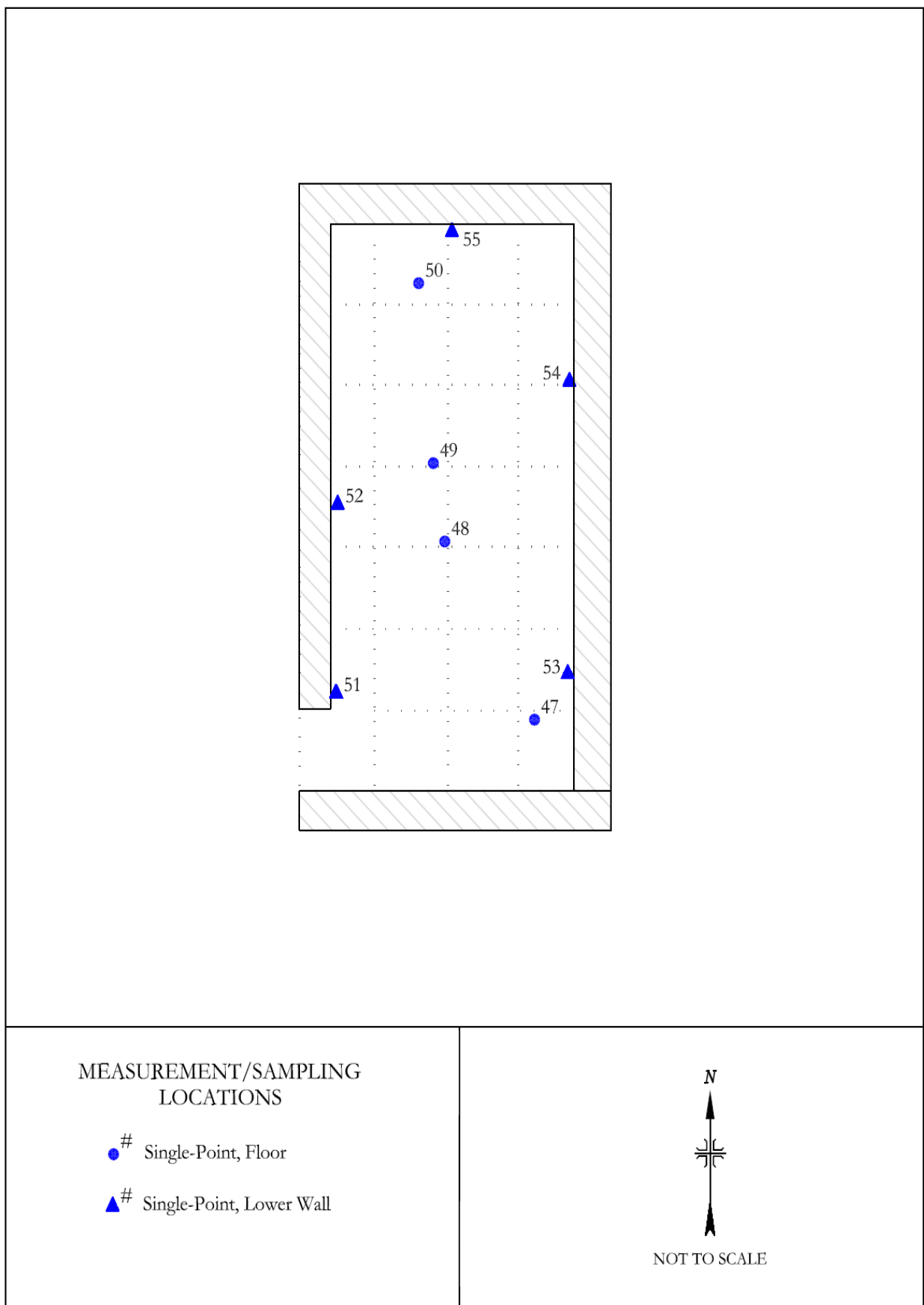
FIGURE 4: Auxiliary Building, Room 24 - Direct Measurement Locations
