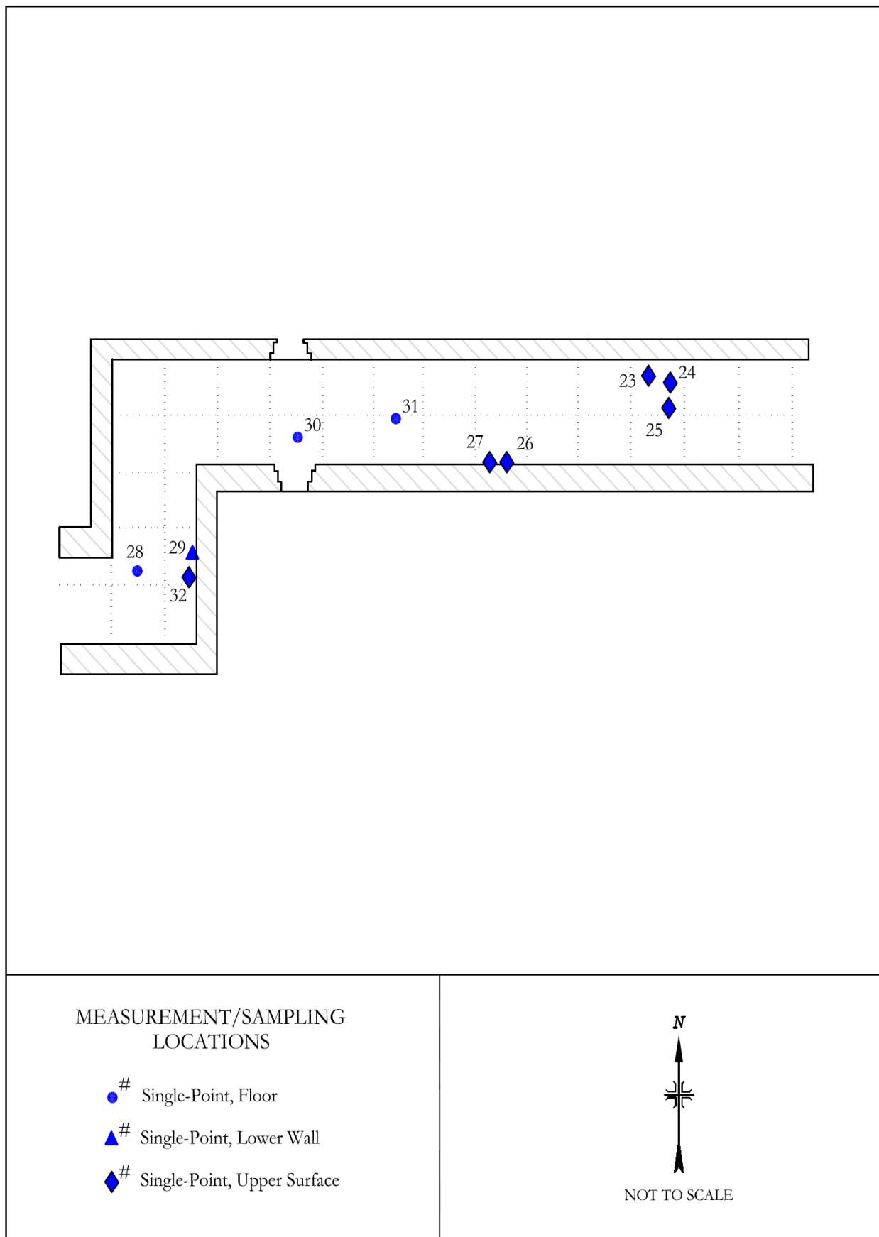
FIGURE 8: Auxiliary Building, Room 45 - Direct Measurement Locations
