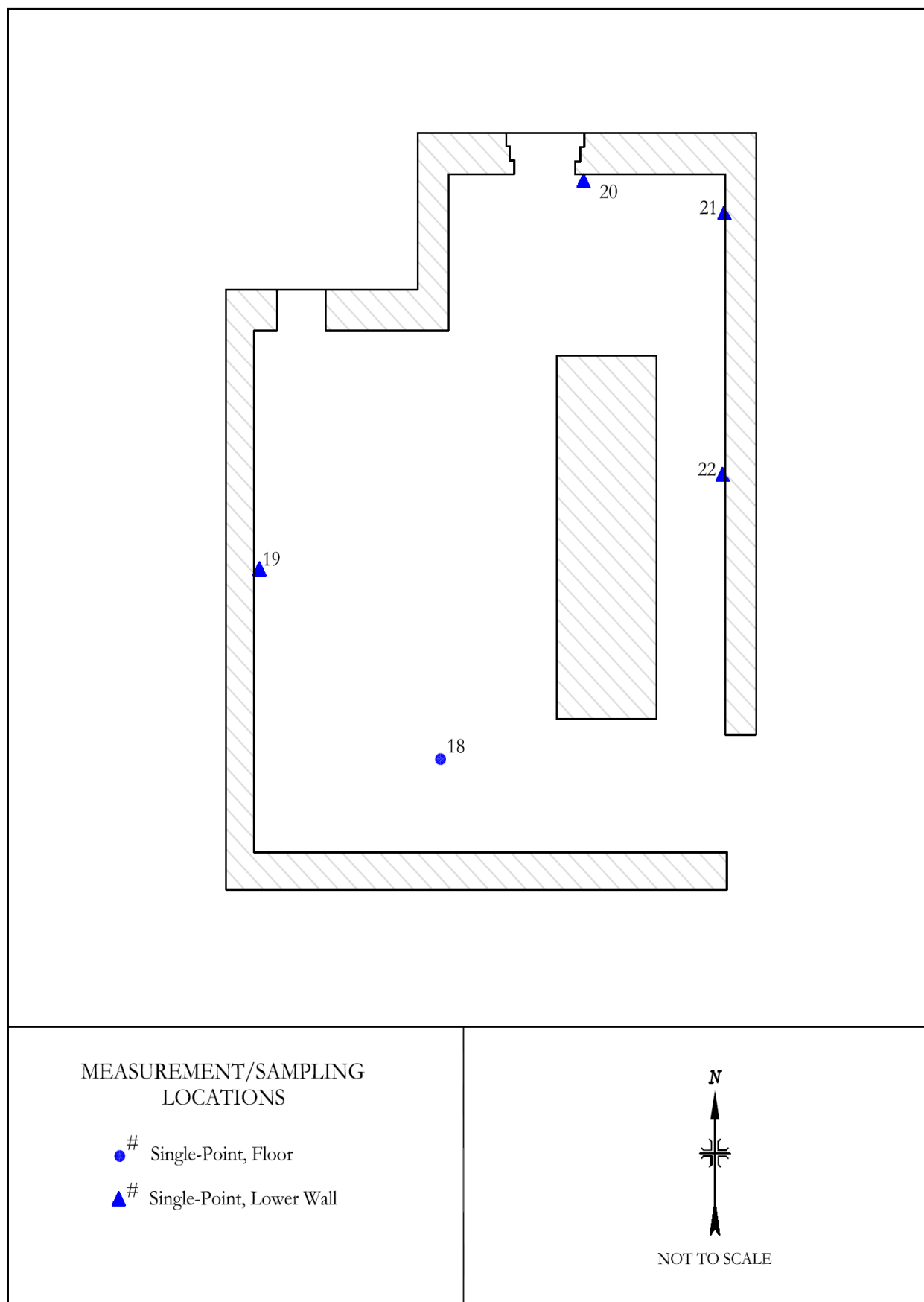
FIGURE 7: Auxiliary Building, Room 44 - Direct Measurement Locations
