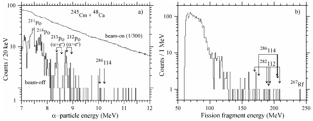
FIG. 1. a) Total beam-on and beam-off \alpha -particle energy spectra of events registered by the focal-plane detector and by both the focal-plane and side detectors in the ^{245}\text{Cm} + ^{48}\text{Ca} reaction. In the beam-off \alpha -particle spectrum we observe the peaks originating from isotopes of Po, the decay products of long-lived isotopes of Ra-Th produced in transfer reactions, and ^{211}\text{Po} , the descendant nucleus of ^{219}\text{Th} produced in the calibrations with a ^{nat}\text{Yb} target. The energies of events observed during beam-off periods in the correlated decay chains are shown by arrows (see Table II). b) Total fission-fragment energy spectrum in the ^{245}\text{Cm} + ^{48}\text{Ca} reaction; the arrows show the energies of events observed in the correlated decay chains.
