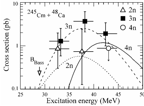
FIG. 2. Excitation functions for the 2n , 3n , and 4n evaporation channels from the complete-fusion reaction ^{245}\text{Cm} + ^{48}\text{Ca} . The Bass barrier [19] is shown by an open arrow. Lines show the results of theoretical predictions [23]. Error bars correspond to statistical uncertainties.
