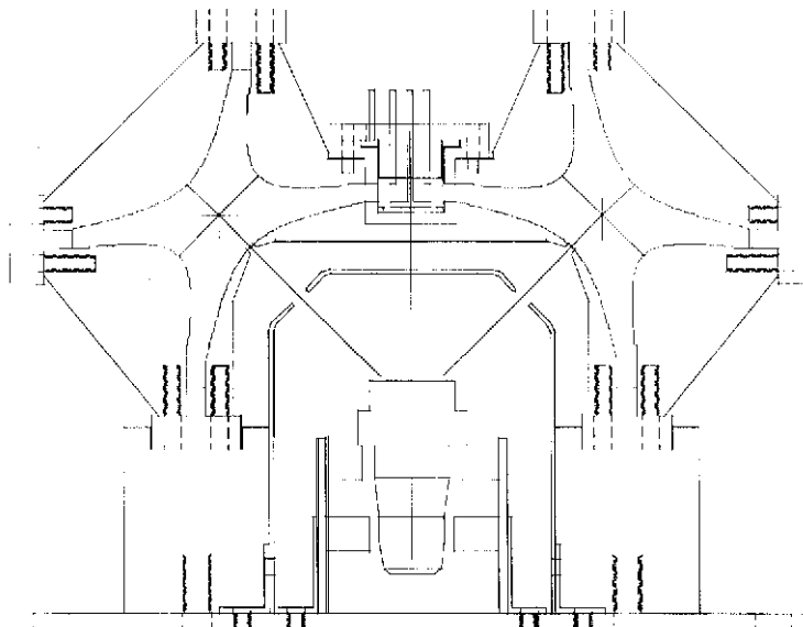
FIGURE 2: Schematic of new toroid analyzer geometry that allows use of standard electron multiplier in place of multichannel plate detector
