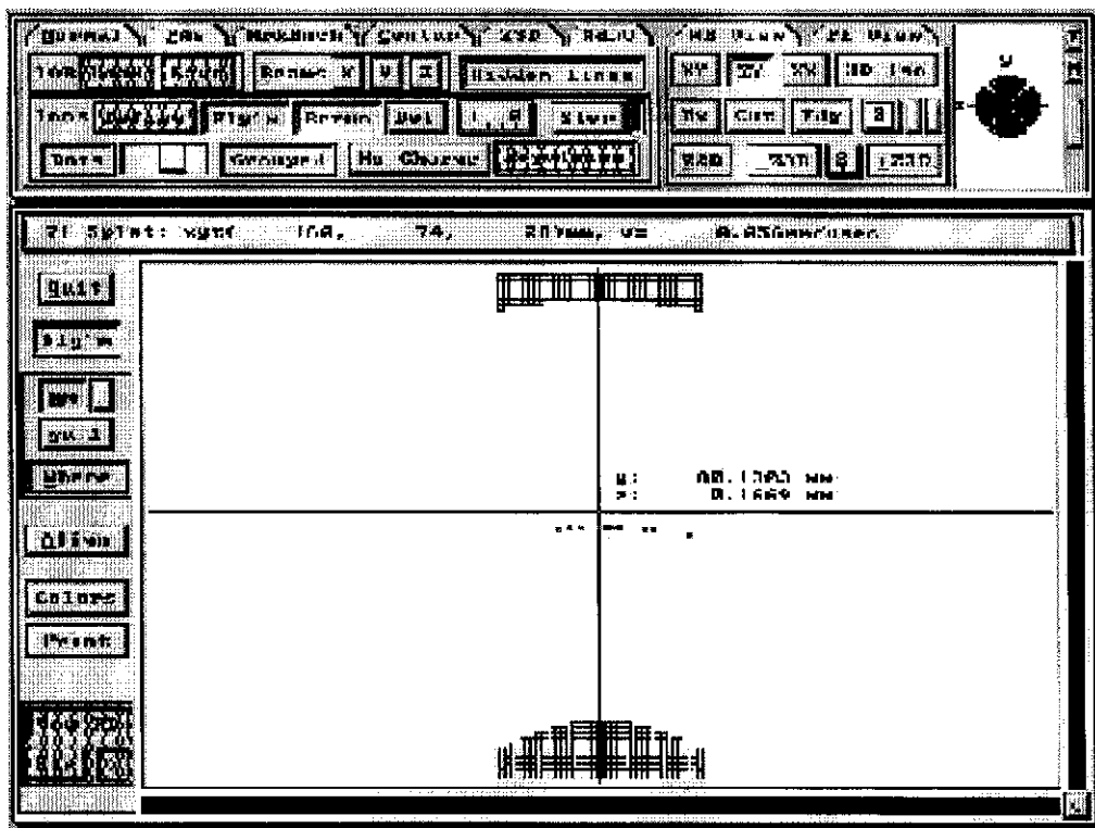
FIGURE 1: Toroid ion trap simulation showing final ion position at a point away (towards inner ring electrode) from the physical center of the toroid electrode structure (crosshair position)
