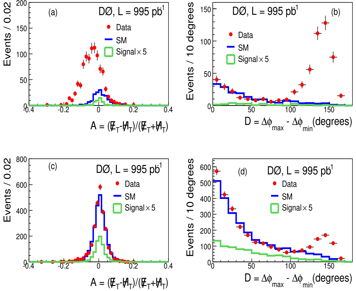
Figure 8.1: Distributions of the asymmetry A = \cancel{E}_T - \cancel{H}_T / \cancel{E}_T + \cancel{H}_T with the cut on \Delta\phi_{\text{max}} - \Delta\phi_{\text{min}} inverted (a) and applied (c). Distributions of \Delta\phi_{\text{max}} - \Delta\phi_{\text{min}} with the cut on A inverted (b) and applied (d) for data (points with error bars), for SM backgrounds (histogram), and for a signal with m_{\tilde{t}} = 150 \text{ GeV} and m_{\tilde{\chi}_1^0} = 70 \text{ GeV} (hatched histogram). In all plots the signal contribution has been scaled by five and \cancel{E}_T > 60 \text{ GeV} is required. The excess in data at A = 0 is consistent with the systematic uncertainties on the predicted background.
