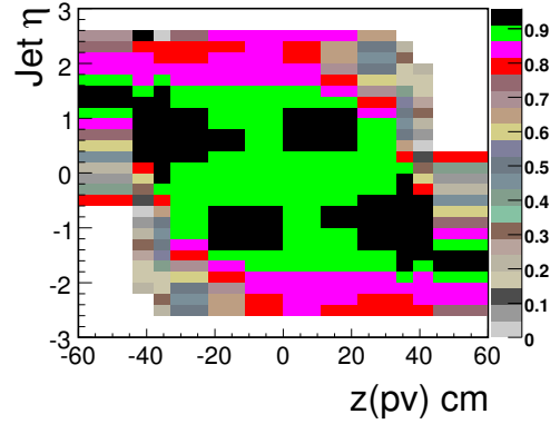
Figure 8.11: Taggability parametrization obtained by interpolating between six fit functions shown in Fig. 8.10.
