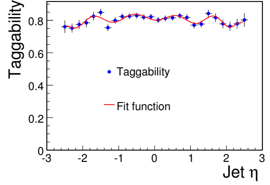
Figure 8.9: Taggability as a function of the detector \eta of the jet observed in data. The fit function used to parametrize the distribution is also shown.
