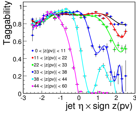
Figure 8.10: Taggability as a function of the product of the detector \eta of the jet and sign z(pv) divided into six regions according to the z position of the primary vertex. The fit function are also shown.
