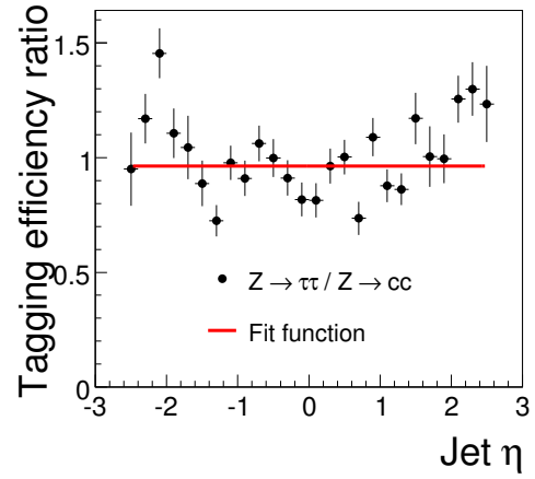
Figure 8.17: Top: Distributions for tagging efficiencies as a function of the \eta_{\text{det}} of the jet for Z(\rightarrow b\bar{b}) , Z(\rightarrow c\bar{c}) , Z(\rightarrow q\bar{q}) and Z(\rightarrow \tau^+\tau^-) MC samples. Bottom: The distribution of the ratio of the tagging efficiency for \tau jets to that for c jets along with the parametrization.
