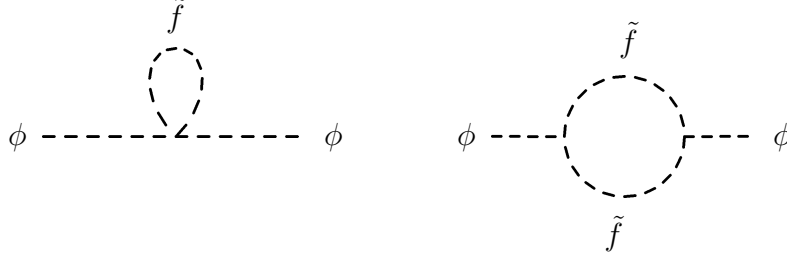
Figure 2.2: Scalar fermion loop corrections to Higgs mass.
