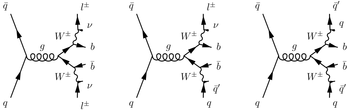
Figure 6.3: Feynman diagrams for top pair production along with the all leptonic, lepton+jets and all hadronic decay modes of W bosons.
