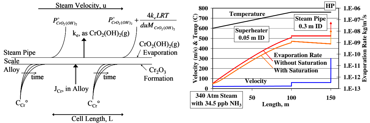
Figure 2. The combination of gas evaporation of \text{CrO}_2(\text{OH})_2 , gas saturation of \text{CrO}_2(\text{OH})_2 , and Cr depletion in the alloy is illustrated. This represents one section of superheater tubing or steam pipe of cell length L . Figure 3. The effects of gas saturation is shown for a hypothetical arrangement of a 100m long SH that leads into a 50m steam pipe that leads to a high pressure (HP) turbine. Saturation results in an 80% reduction in the evaporation rate at the HP turbine.
