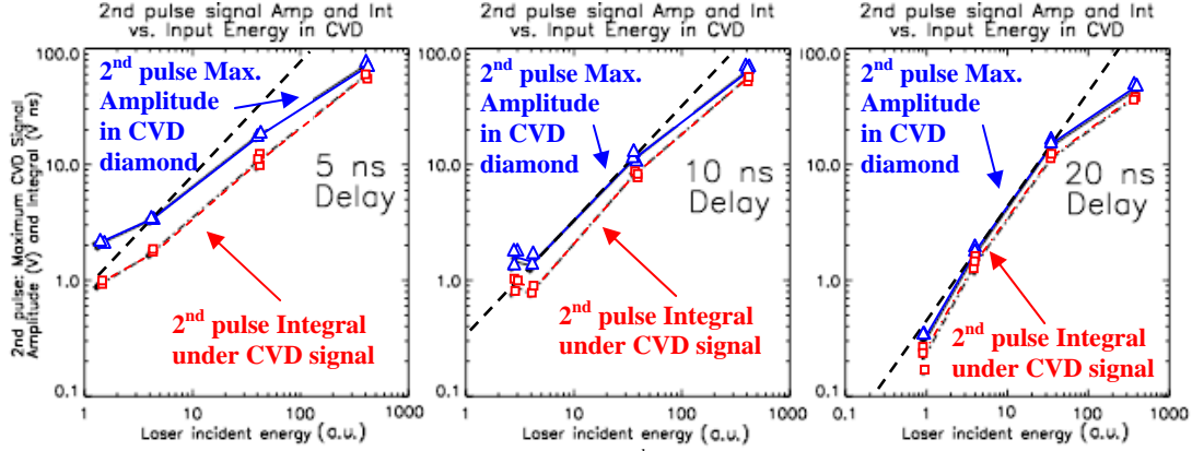
Figure 2. Maximum signal amplitude, V_{\max} (V), of the 2 nd pulse and integral under the pulse, S (V ns), in the CVD diamond wafer versus incident energy for the 2 nd pulse (in arbitrary but consistent units). The straight-dashed lines are the linearity lines. Results are shown for the 3 delay times, 5, 10, and 20 ns in between both pulses.
