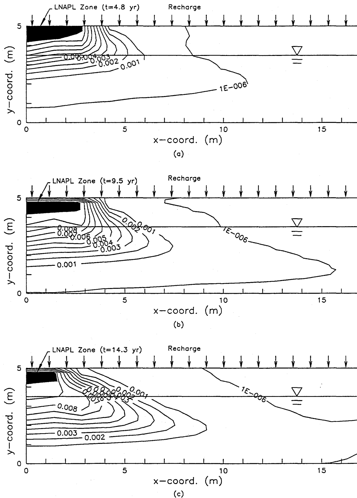
Figure 4.39. Model predictions of the shrinking LNAPL zone and aqueous-phase concentrations at three typical time values, (a) t = 4.8 yr, (b) t = 9.5 yr., and (c) t = 14.3 yr.
