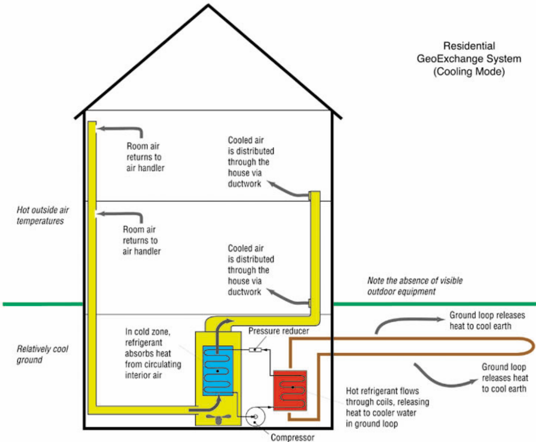
Figure 6-12: GHP Operation – Cooling Mode
