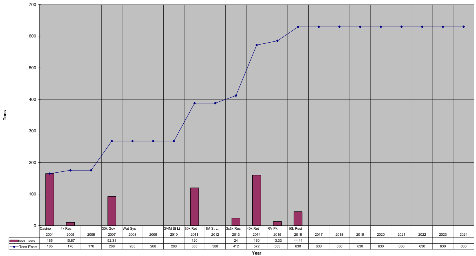
Figure 5-3: Cooling Demand Forecast
