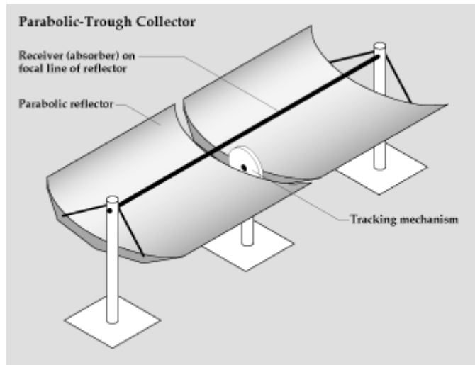
Figure 6-7: Parabolic Trough Collectors
