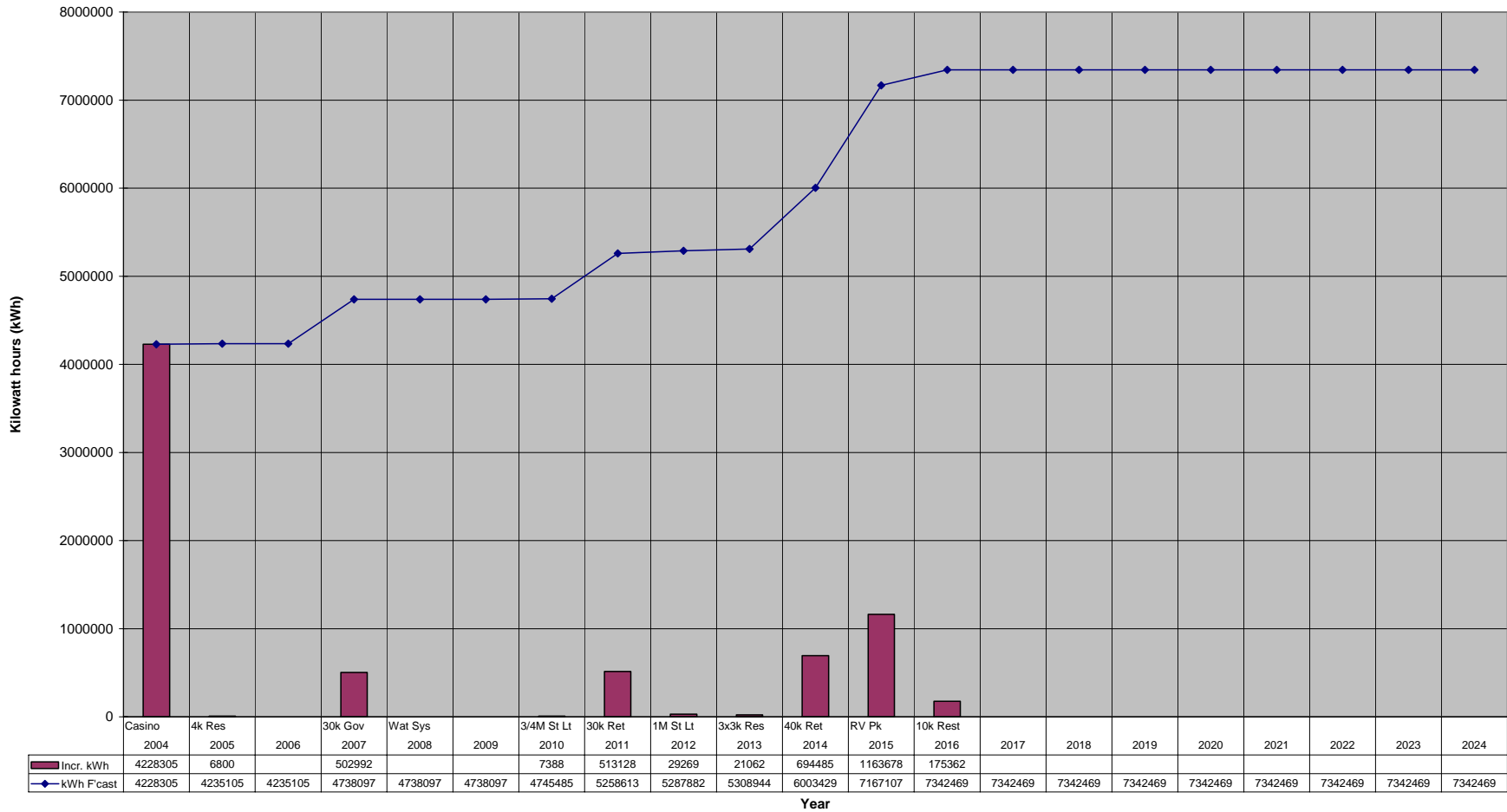
Figure 5-2: Electric Consumption Forecast
