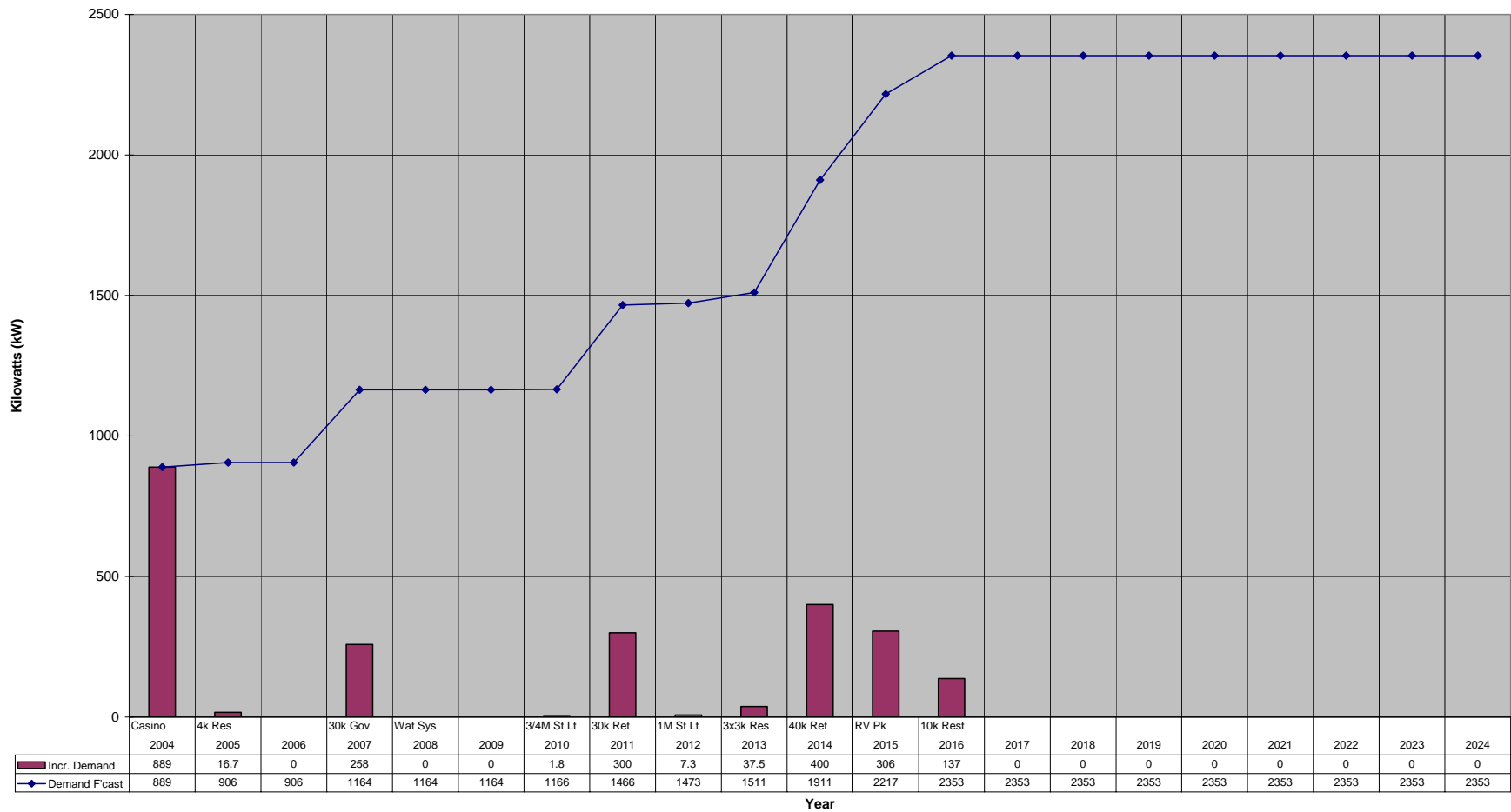
Figure 5-1: Electric Demand Forecast
