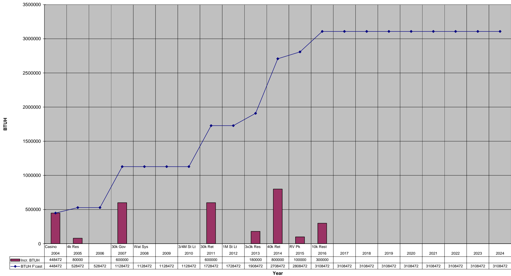
Figure 5-4: Heating Demand Forecast
