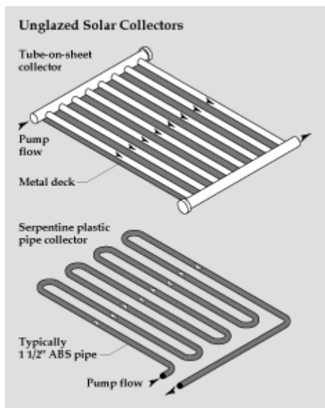
Figure 6-4: Unglazed Solar Collectors
