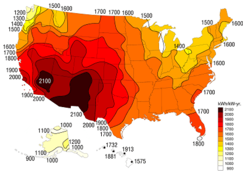
Energy produced each year, in kilowatt-hours, for a one-kilowatt photovoltaic solar electric system
