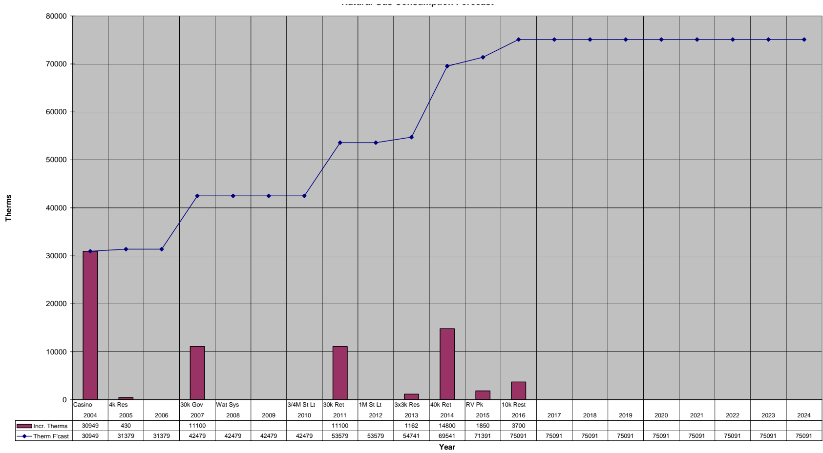
Figure 5-5: Natural Gas Consumption Forecast
