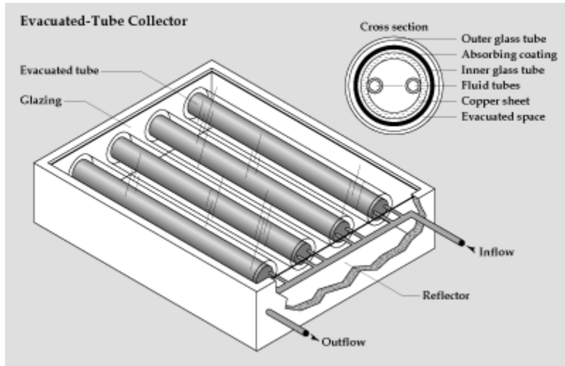
Figure 6-6: Evacuated Tube Collectors
