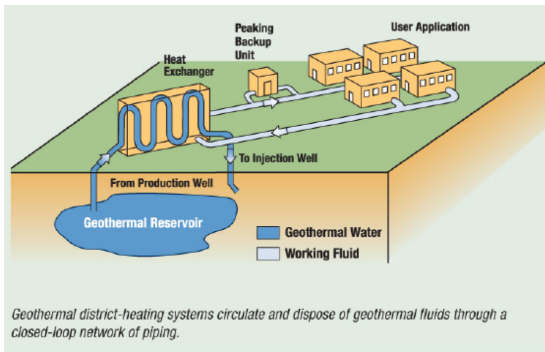
Figure 6-11: Direct Use District Heating System
