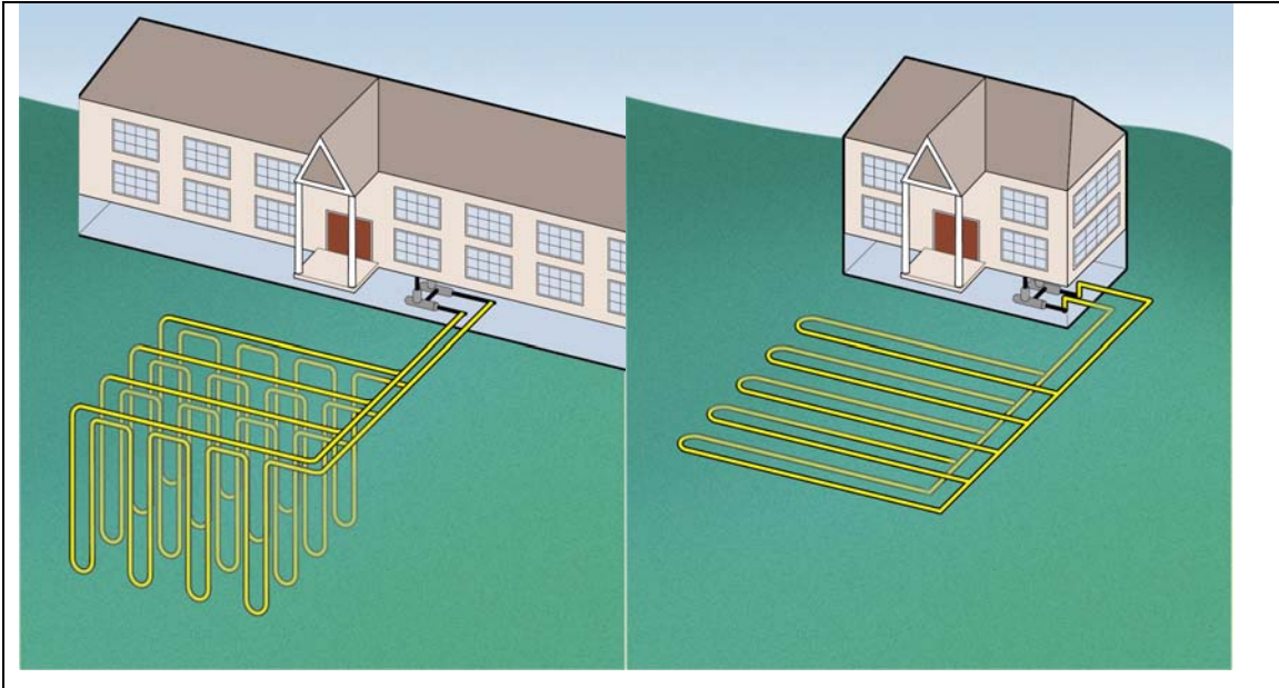
Figure 6-13: Typical Commercial Vertical and Horizontal Loop Fields
