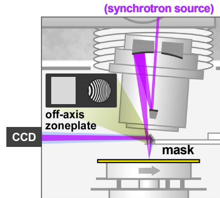
Figure 2. SEMATECH Berkeley Actinic Imaging tool
