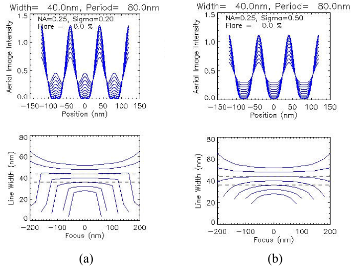
Figure 5. CD change vs focus as a function of threshold (a) sigma 0.2 (b) sigma 0.5
