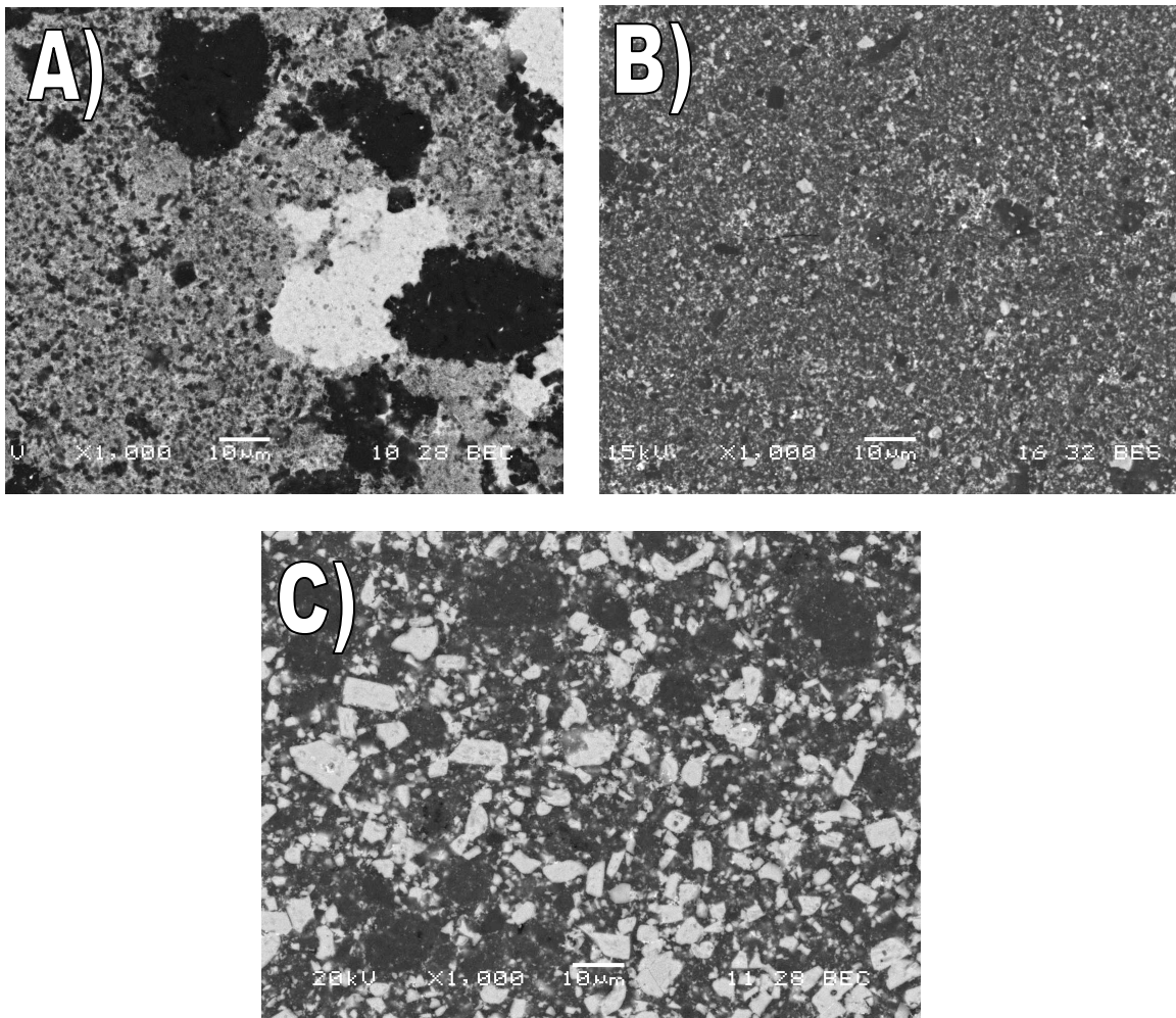
Figure 4.2: Backscattered electron images showing range of microstructural variations in \text{AlMgB}_{14} - 30 wt% \text{TiB}_2 composites prepared by mechanical alloying. Dark regions are \text{AlMgB}_{14} , white corresponds to \text{TiB}_2 , and the grey regions are a nanoscale mixture of the two phases. A) vibratory-milled, prepared from chunk boron, B) vibratory-milled, prepared from elemental powders, C) attritor-milled, prepared from elemental powders. Note the difference in phase distribution and size resulting from the various types of milling equipment (all micrographs were obtained at a magnification of 1000x)
