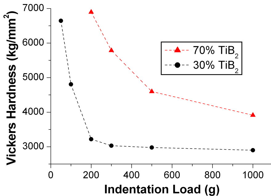
Figure 7.6: Indentation size effect on hardness of an \text{AlMgB}_{14} - 70 wt% \text{TiB}_2 composite compared to an older 30 wt% \text{TiB}_2 composite (Lewis) [14].
