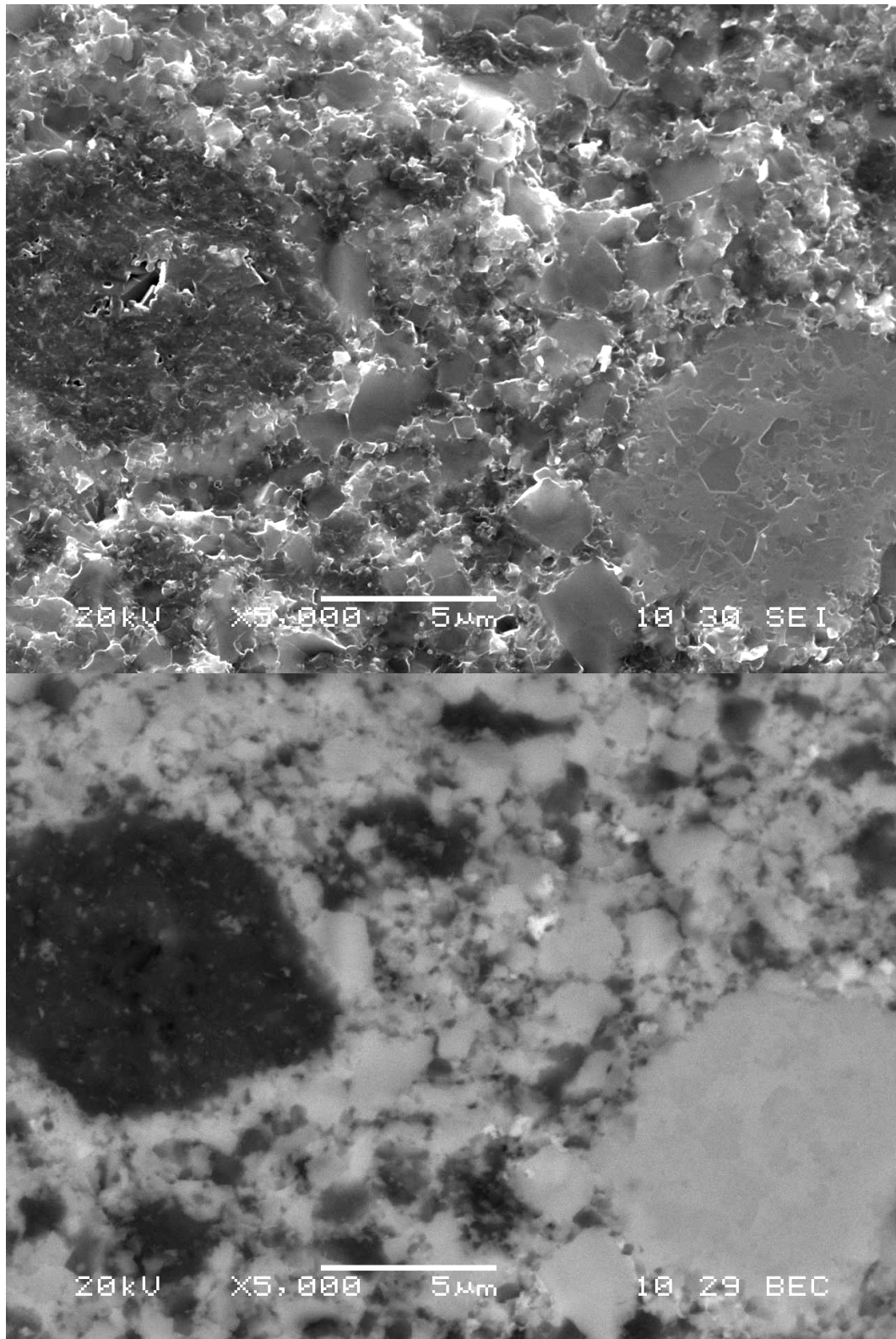
Figure 7.10: Fracture surface of AlMgB 14 - 70 wt% MM TiB 2 composite, same area by SE (top) and BSE (bottom) imaging. AlMgB 14 agglomerate (dark) and TiB 2 agglomerate (light) surrounded by typical composite microstructure. Hot-pressed at 1400°C and 106 MPa pressure.
