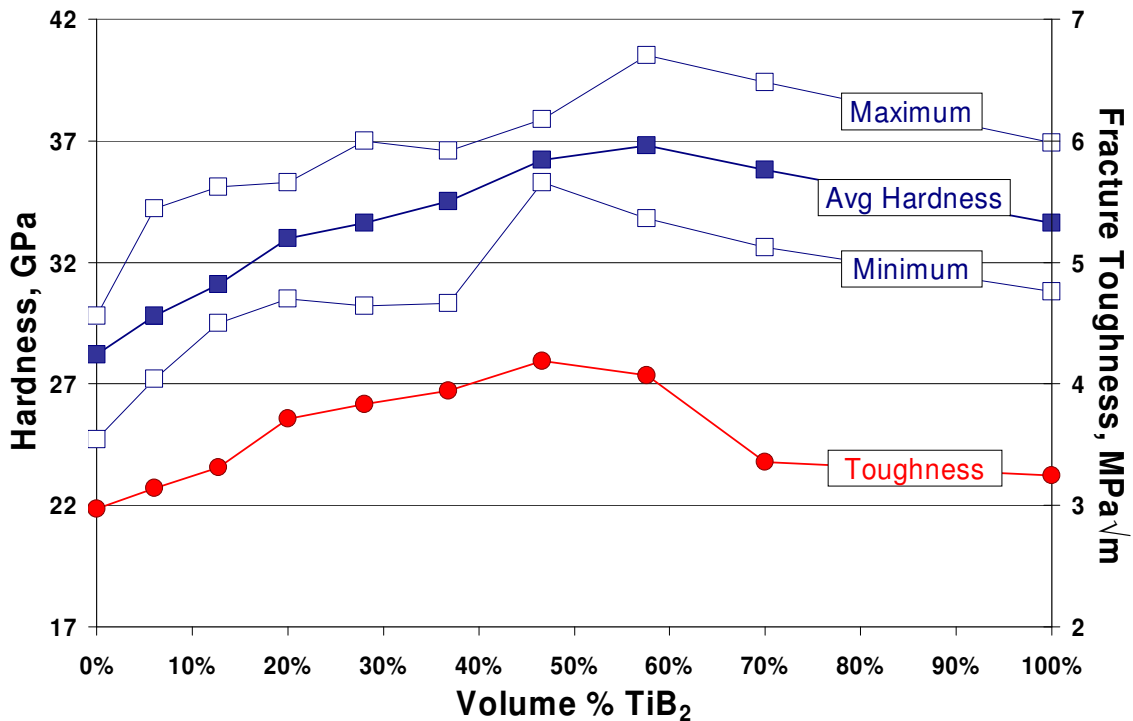
Figure 5.1: Vickers hardness and Palmqvist fracture toughness for AlMgB 14 -TiB 2 composites [69].
