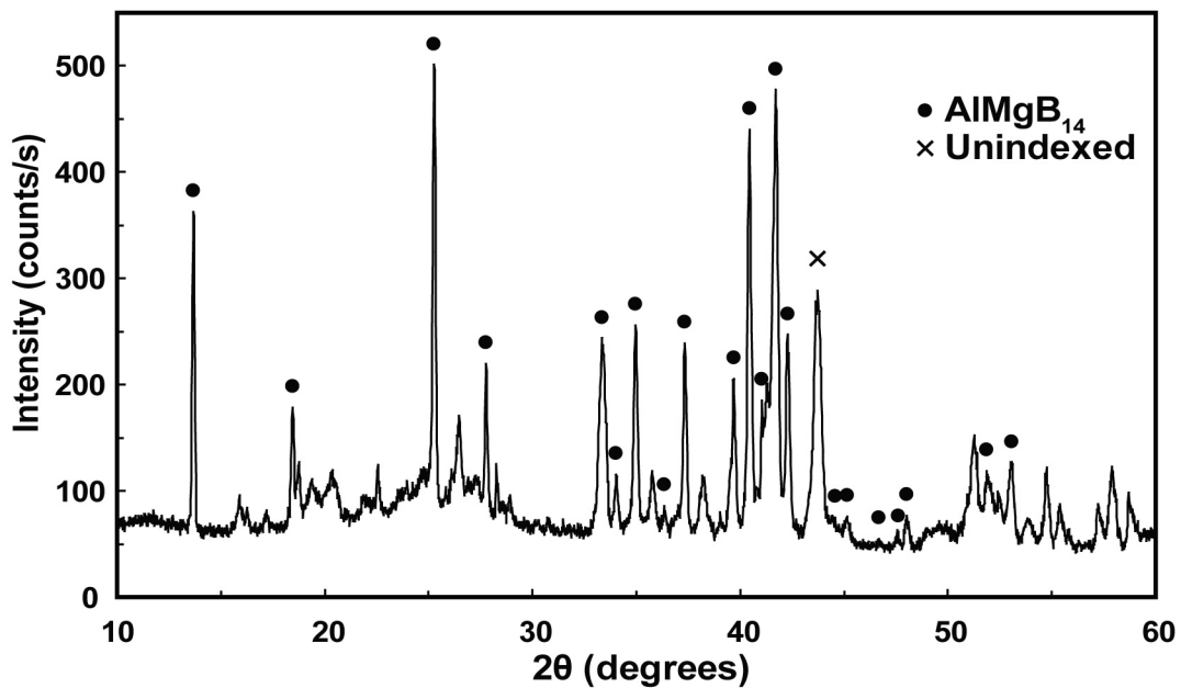
Figure 3.3: X-ray diffraction pattern of \text{AlMgB}_{14} reacted for 6 hours at 1300^\circ\text{C} . Unindexed peak marked with “X” matches unidentified peak seen in \text{Mg}_2\text{B}_{14} samples.
