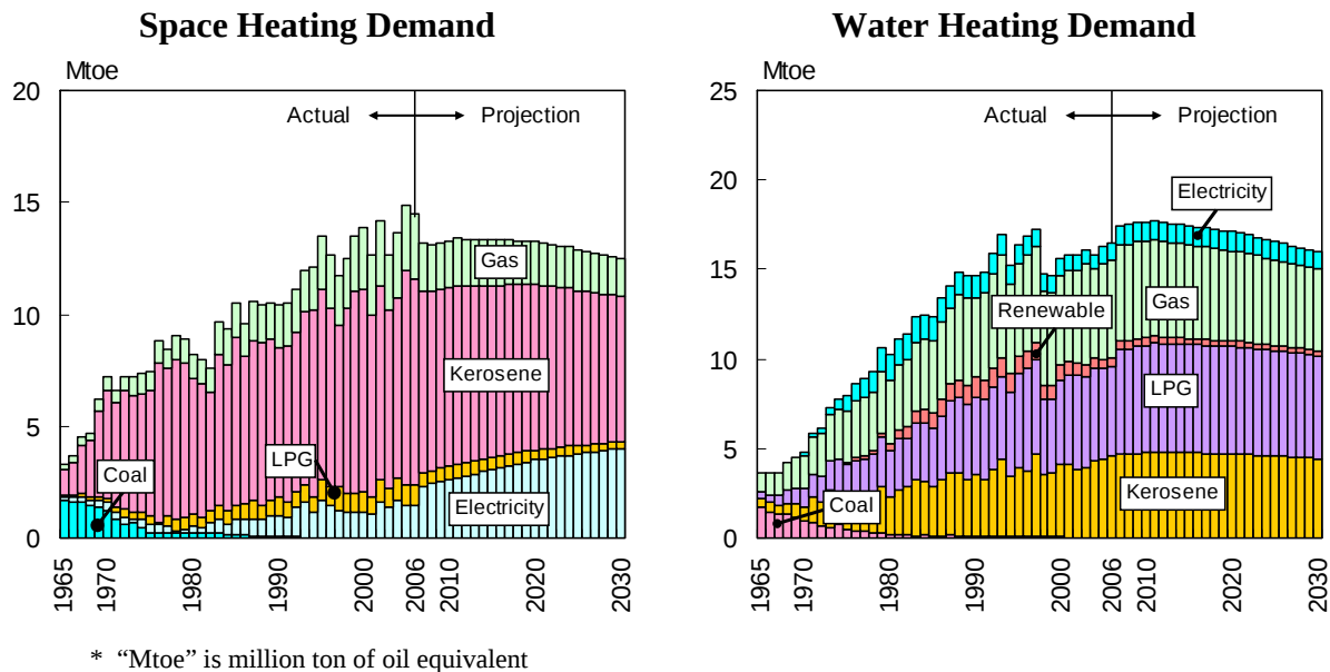
Figure 10. Space Heating and Water Heating Demand in Japanese Residential Sector by Energy Source to 2030 in (300 Trial Runs, Average Value)
