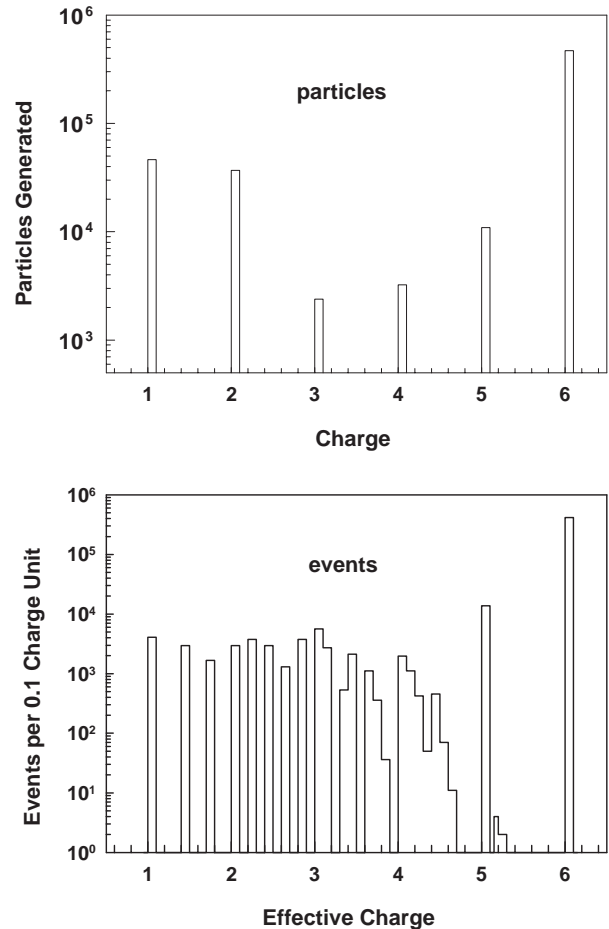
FIG. 11: Above, Figure 11a shows a histogram of particle charges produced by PHITS for a 290 MeV/nucleon carbon beam incident on an aluminum target. Below, Figure 11b shows the charge distribution after combining the fragment charges, as in the measurements. These are referred to as "track" and "event" analyses, respectively.
