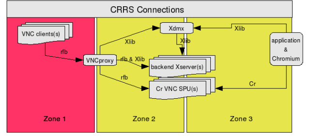
Fig. 3. CRRS Security Zones. Zone 1 traffic consists exclusively of RFB protocol messages, and typically occurs over the open internet. A commonly accepted practice to “secure” this connection is to force all such traffic through SSH tunnels, where site-wide policy can enforce authentication and the connection is armored. Inside the center, Zone 2 traffic consists of a mixture of RFB and Xlib messages between the Proxy and the VNC servers. Zone 3 traffic consists of application-generated OpenGL and Xlib command streams, and is typically where services like MPI are provided for parallel application operation.
