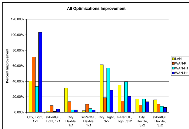
Fig. 8. Relative performance improvement from enabling all optimizations.
