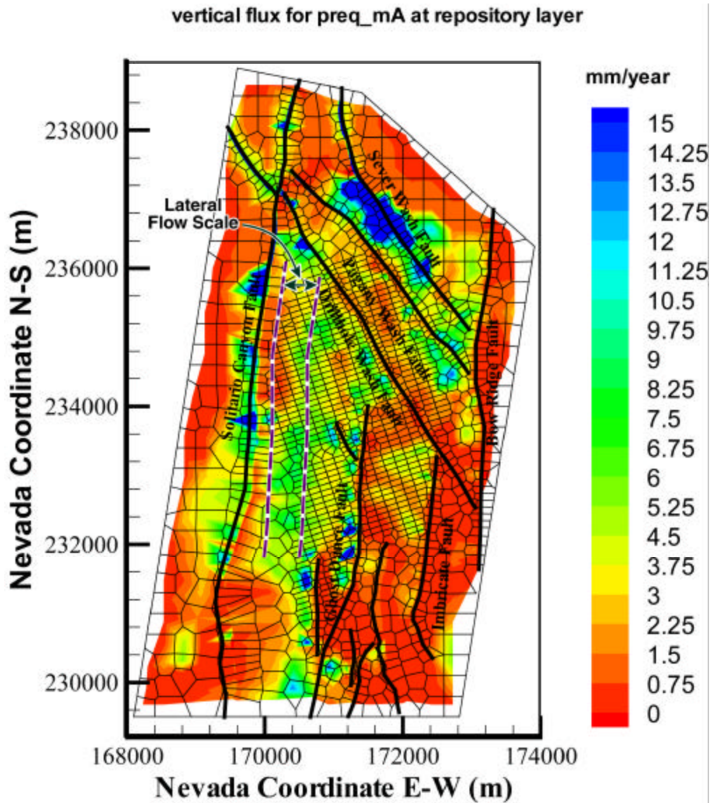
Figure 8. Simulated percolation fluxes at the repository horizon, using the present-day, mean infiltration scenario, base-case model results (peq_mA) (modified from Wu et al. , 2004)
