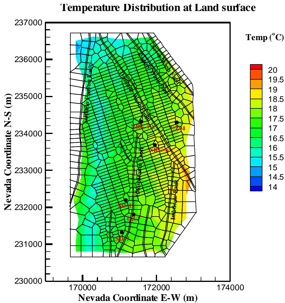
Figure 14b. Temperature distributions estimated at the Yucca Mountain surface
