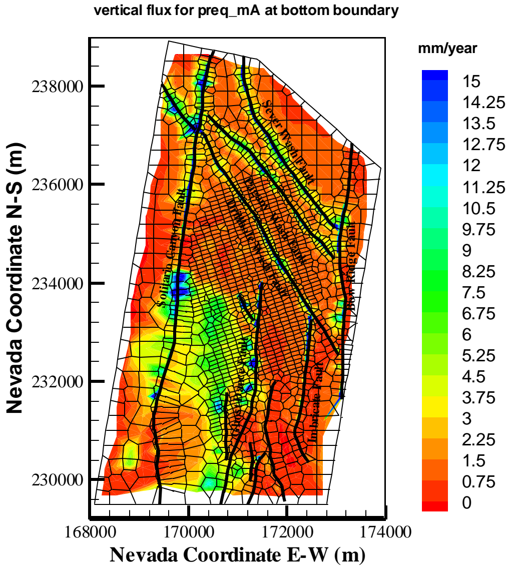
Figure 11. Simulated percolation fluxes at the water table, using the present-day, mean infiltration scenario, base-case model results (peq_mA)
