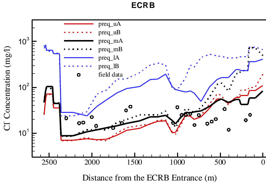
Figure 16. Comparison between measured and simulated chloride concentration (mg/L) profiles along the ECRB for present infiltration with mean, upper, and lower bounds
