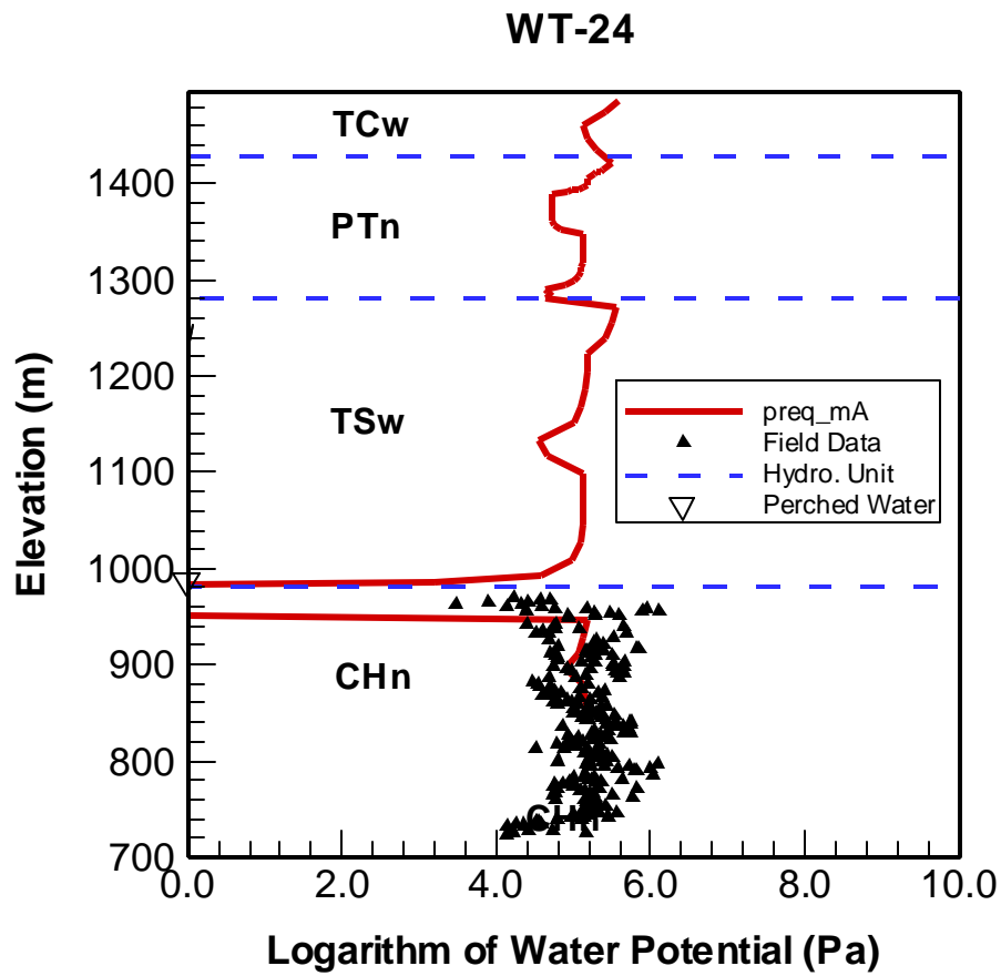
Figure 6. Comparison of simulated and measured matrix water potentials and perched-water elevations at borehole WT-24, using the present-day mean infiltration rate (req_mA)
