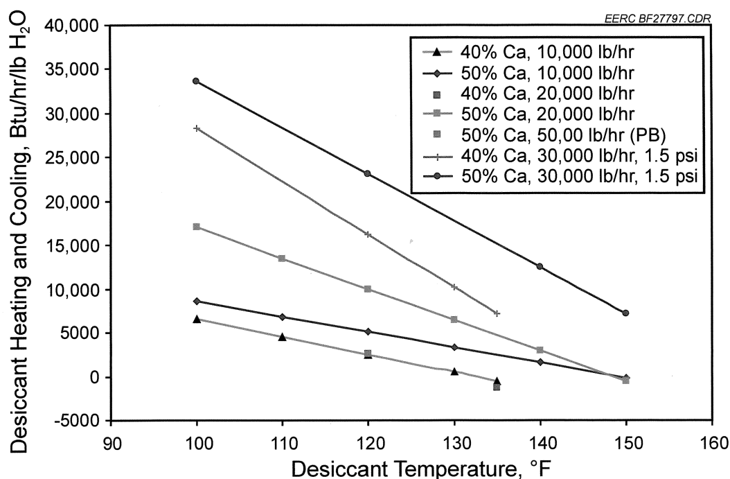
Figure 42. Energy required to regenerate desiccant as a function of design parameters.
