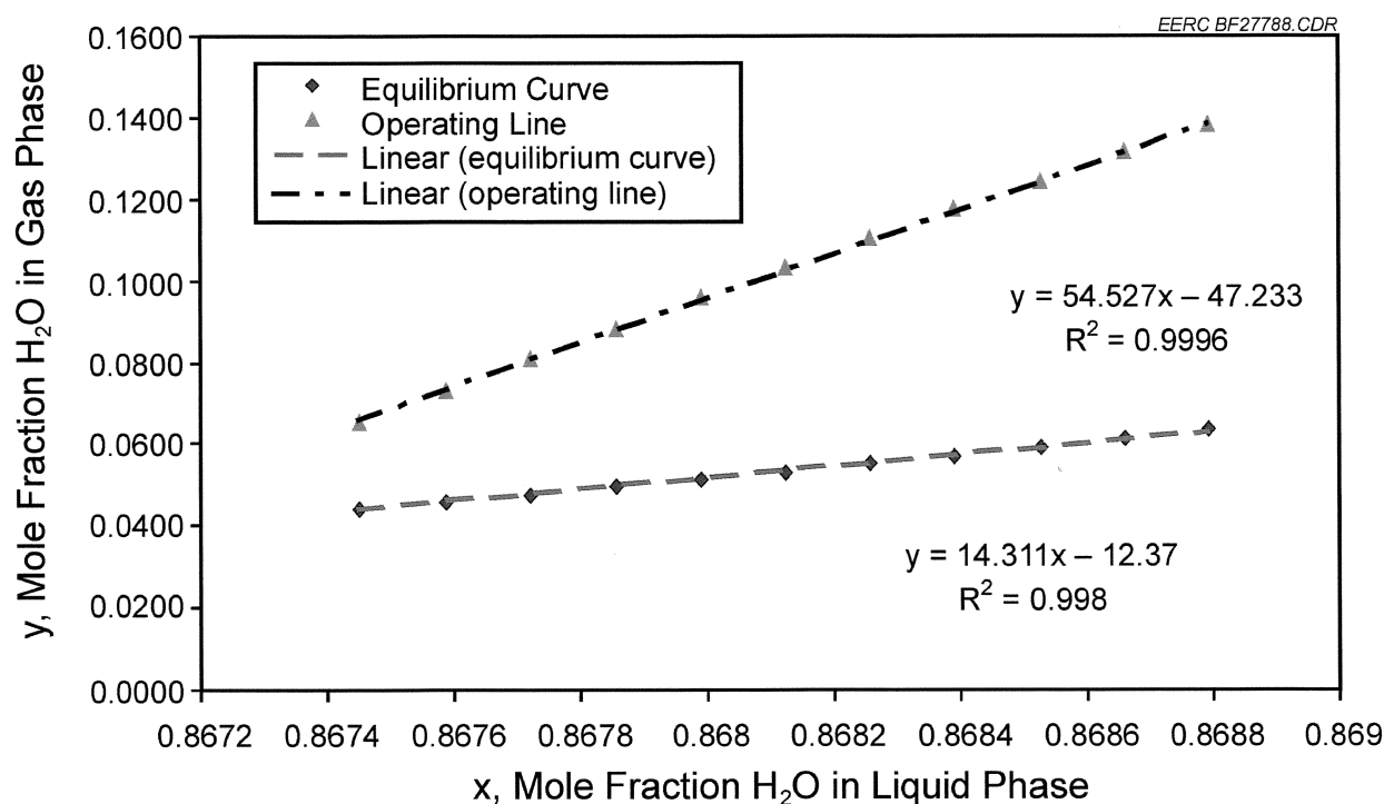
Figure 33. Operating and equilibrium lines for the flue gas \text{CaCl}_2 desiccant system.
