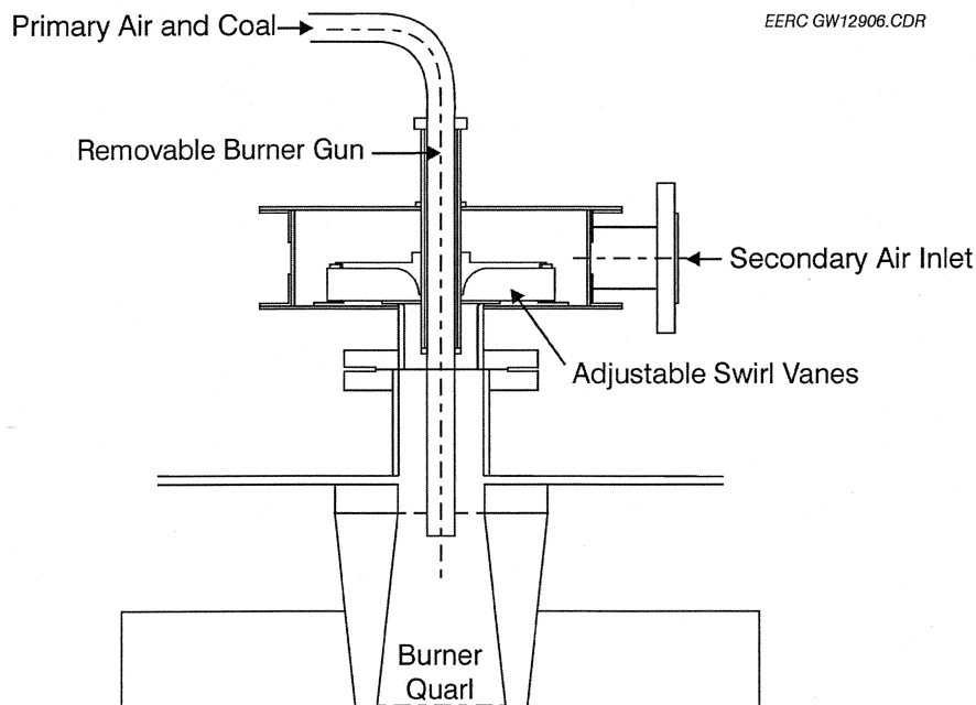
Figure 5. Schematic of the SFS basic burner design, an IFRF-type adjustable secondary air swirl generator.
