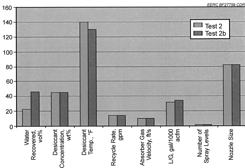
Figure ES-5. Average product water recovery rate varying desiccant temperature and L/G, Test Series II.
