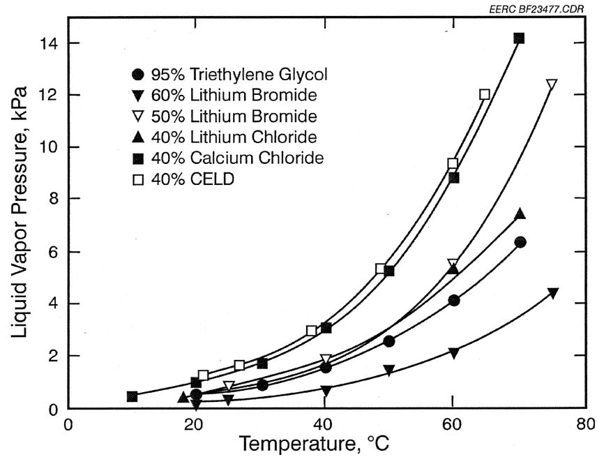
Figure 14. Vapor pressure of liquid desiccants (Oberg and Goswami, 1998) as a function of temperature for various concentrations of desiccant (CEL D: cost-effective liquid desiccant, a mixture of calcium and lithium chloride).
