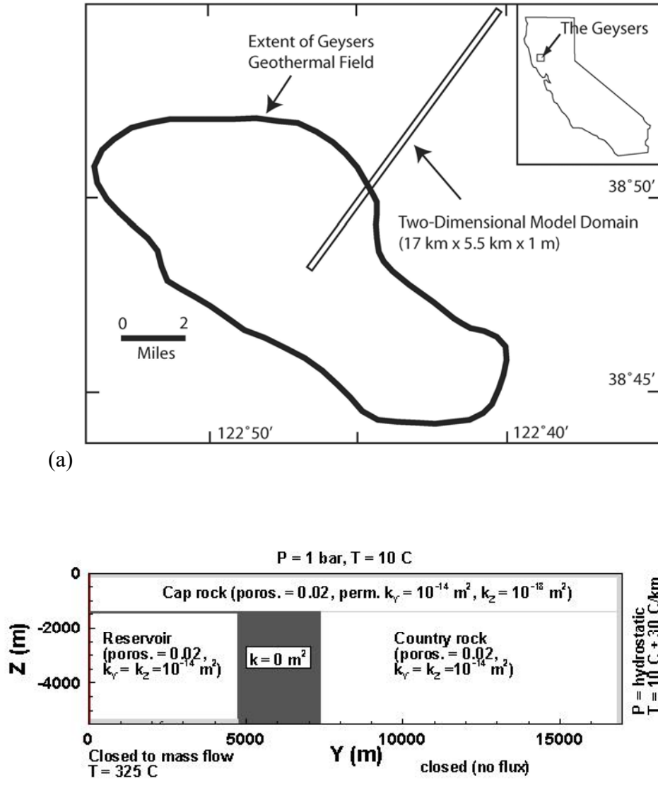
Figure 1. Two-dimensional model for coupled THM analysis of induced seismicity at The Geysers. (a) Location map of The Geysers showing approximate boundary of the geothermal reservoir and orientation of the two-dimensional model domain and (b) model geometry with hydraulic properties of different rock units and boundary conditions.
