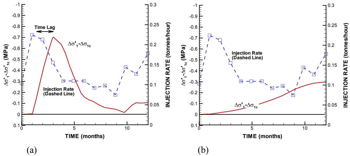
Figure 7. Comparison of injection rate and evolution of failure margin ( \Delta\sigma'_1 - \Delta\sigma'_{lc} ) at (a) the bottom of the injection well ( x = 217.5 m, z = -3325 m), and at (b) about 1700 m below the injection well ( x = 217.5 m, z = -5000 m).
