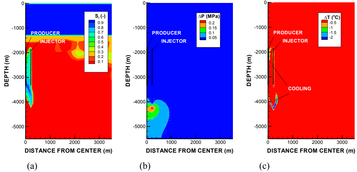
Figure 5. Calculated basic thermal-hydrological responses after 6 months of the 2005 seasonal injection analysis. (a) liquid saturation, (b) changes in fluid pressure, and (c) changes in temperature.
