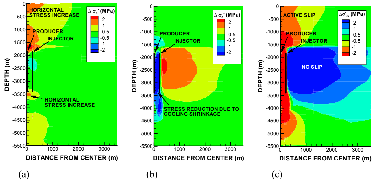
Figure 4. Calculated geomechanical responses after 44 years of production/injection. Changes in (a) horizontal effective stress (b) vertical effective stress and (c) potential for failure, \Delta\sigma'_{lm} = \Delta\sigma'_{l1} - \Delta\sigma'_{lc} .
