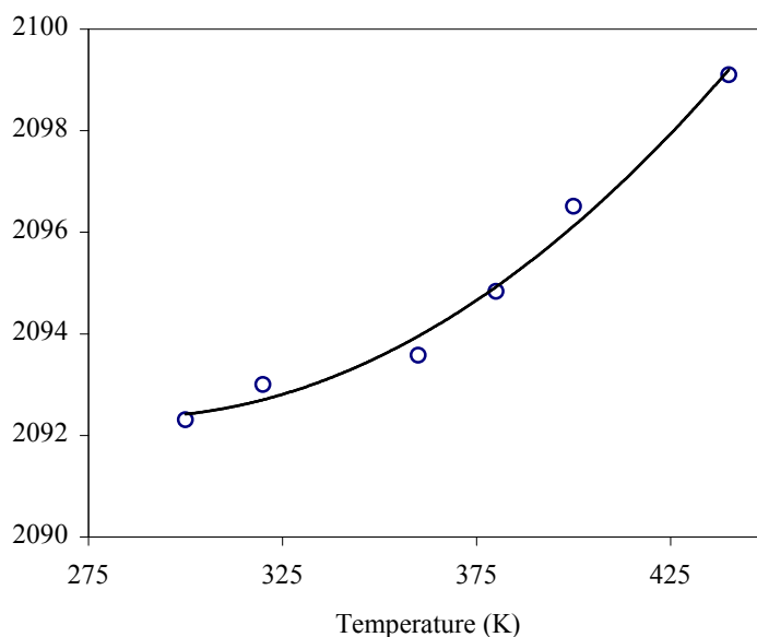
Figure 6.8. CO vibrational resonance frequency, \omega_{\text{CO}} , plotted against the metal surface temperature. Solid line drawn as a visual aide.
