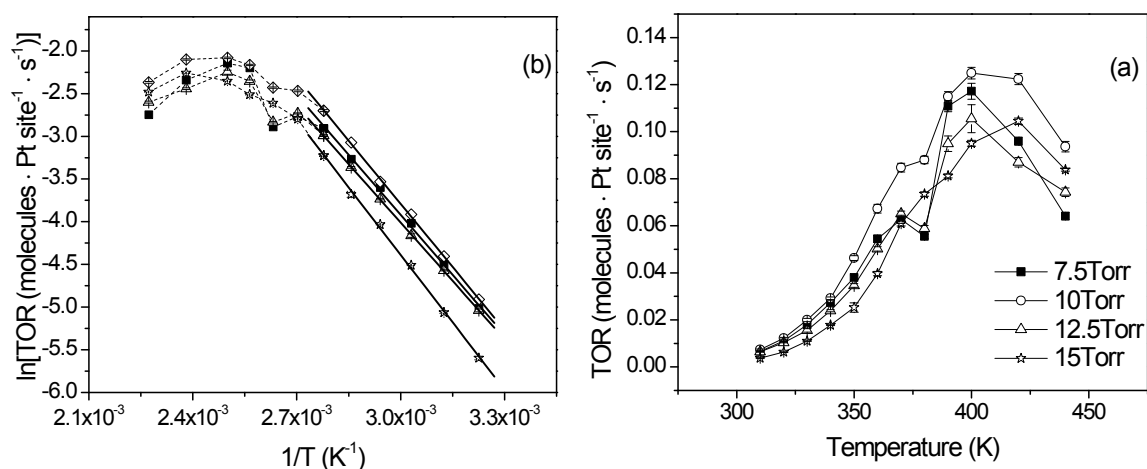
Figure 5.1. (a) Turnover rates (TORs), in molecules per Pt atom per second, for benzene (at 7.5, 10, 12.5, and 15 Torr) hydrogenation to cyclohexane in the presence of \text{H}_2 (100 Torr), and (b) Arrhenius plots of the TORs. Apparent activation energies and pre-exponentials are listed in table 5.1. The decrease in TOR at 380 K followed by a sharp increase at 390 K is attributed to the onset of cyclohexene production (See figure 5.2(a)). Cyclohexene has a higher sticking probability on platinum resulting in further hydrogenation to cyclohexane. The non-Arrhenius behavior above 370 K is explained in terms of changes in the surface coverage of the adsorbates. Dotted lines were drawn for visual aides.
