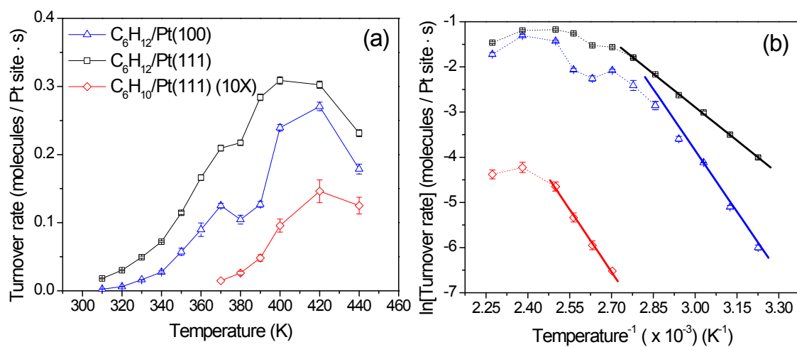
Figure 10.5. (a) Turnover rates of cyclohexane ( C_6H_{12} ) and cyclohexene ( C_6H_{10} ) formation on Pt(100) and Pt(111) single-crystals for 10 Torr C_6H_6 , 100 Torr H_2 , and 650 Torr Ar and (b) corresponding Arrhenius plots. The dotted lines are drawn as visual aides.
