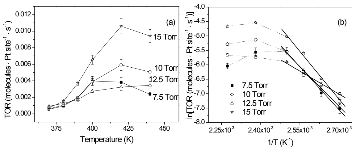
Figure 5.2. (a) Turnover rates (TORs), in molecules per Pt atom per second, for benzene (7.5, 10, 12.5, and 15 Torr) hydrogenation to cyclohexene in the presence of H_2 (100 Torr), and (b) Arrhenius plots of the TORs. Apparent activation energies and pre-exponentials are listed in table 5.2. The non-Arrhenius behavior above 420 K is explained in terms of changes in the surface coverage of the adsorbates. Dotted lines were drawn for visual aides.
