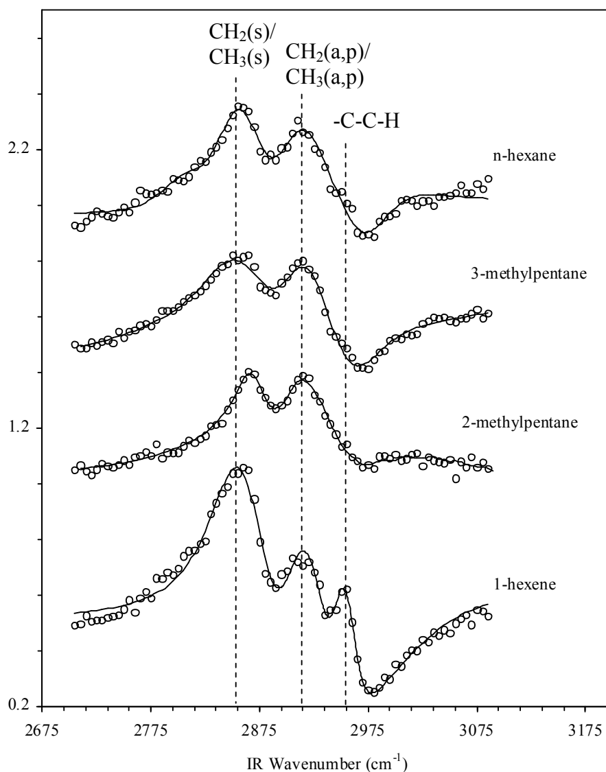
Figure 9.1. SFG spectra of surface species on Pt(100) at 300K in 1.5 Torr C 6 hydrocarbon and 15 Torr H 2 . In order from the top are n -hexane, 3-methylpentane, 2-methylpentane, and 1-hexene, respectively. Markers represent experimental data and solid lines represent the curve fits using equation 9.1.
