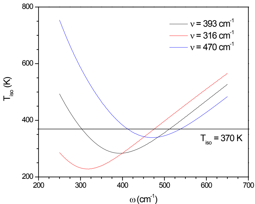
Figure 8.4. Isokinetic temperature, T_{\text{iso}} , calculated for \nu = 393 \pm 77 \text{cm}^{-1} using the full resonance formula. A line at T_{\text{iso}} = 370 K is drawn to obtain the vibration of the heat bath, \omega .
