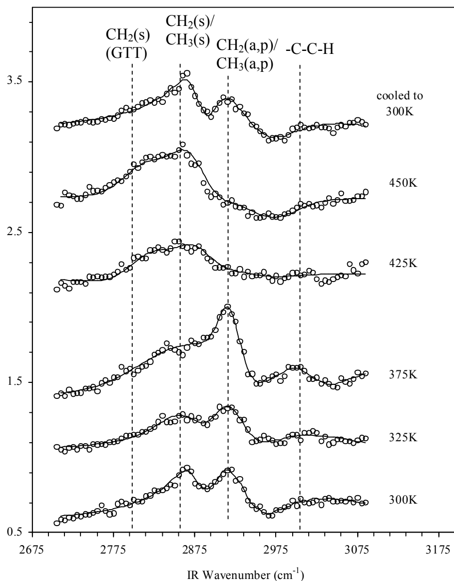
Figure 9.4. Temperature dependent SFG spectra of surface species on Pt(100) under 1.5 Torr 2-methylpentane and 15 Torr \text{H}_2 in the temperature range of 300-450K. The top SFG spectrum was taken after the metal surface was cooled from 450 K to 300 K. Symmetric \text{CH}_2 and \text{CH}_3 ; perturbed asymmetric \text{CH}_2 and \text{CH}_3 ; and vinylic CH bands are identified. Markers represent experimental data and solid lines represent the curve fits using equation 9.1.
