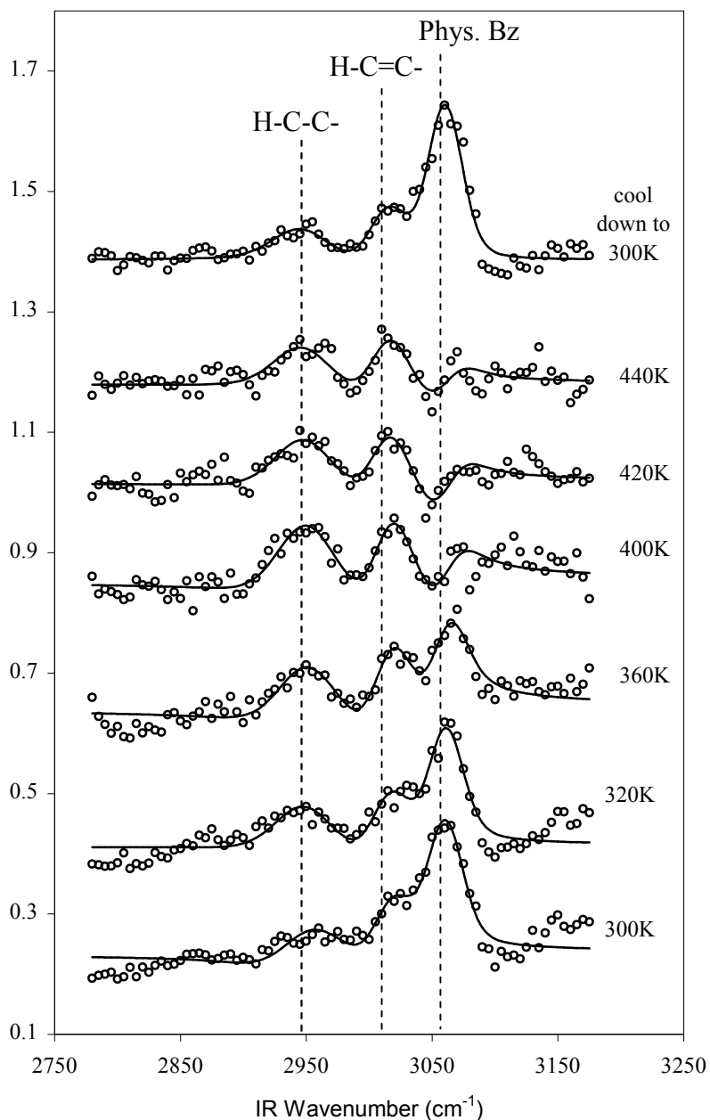
Figure 5.5. Temperature dependent SFG spectra of surface species on Pt(111) under 15 Torr benzene and 100 Torr \text{H}_2 in the range of 300-440 K. The top SFG spectrum was taken after the metal surface was cooled from 440 K to 300 K. H-C-C-, vinylic (H-C=C-), and physisorbed benzene (phys. Bz) bands are identified. Markers represent experimental data and solid lines represent the curve fits to equation 5.1.
