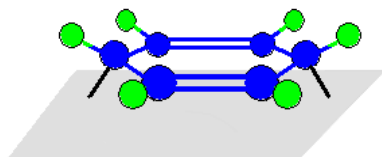
Scheme 5.1. Schematic diagram of dienyl chemisorbed benzene ( C_6H_6 ) intermediate.
