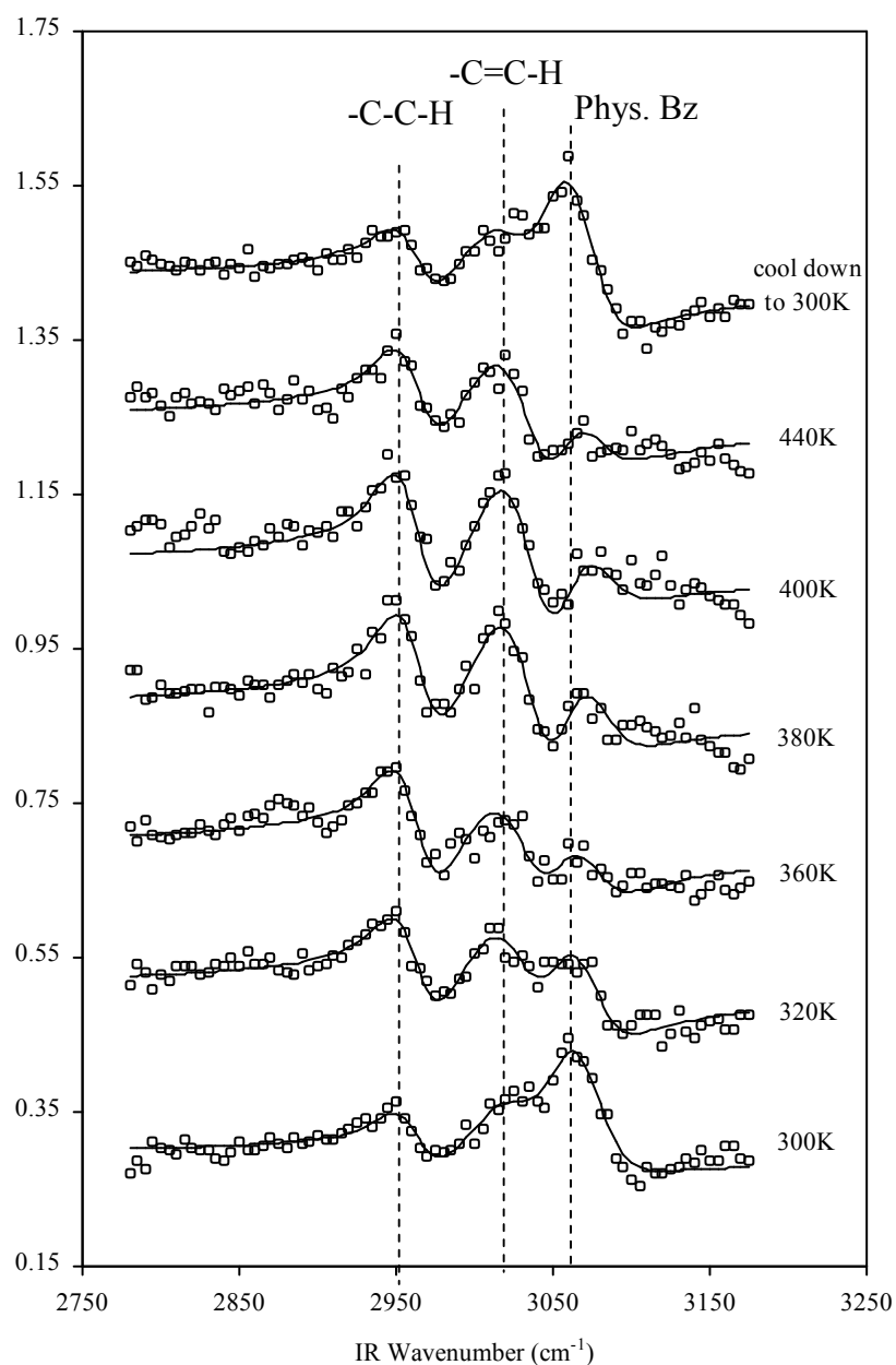
Figure 7.4. Temperature dependent SFG spectra of surface species on Pt(111) under 10 Torr benzene and 10 Torr H 2 in the range of 300-440 K. The top SFG spectrum was taken after the metal surface was cooled from 440 K to 300 K. H-C-C-, vinylic (H-C=C-), and physisorbed benzene (phys. Bz) bands are identified. Markers represent experimental data and solid lines represent the curve fits to equation 7.1.
