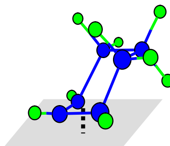
(b) \pi -allyl c-C 6 H 9
