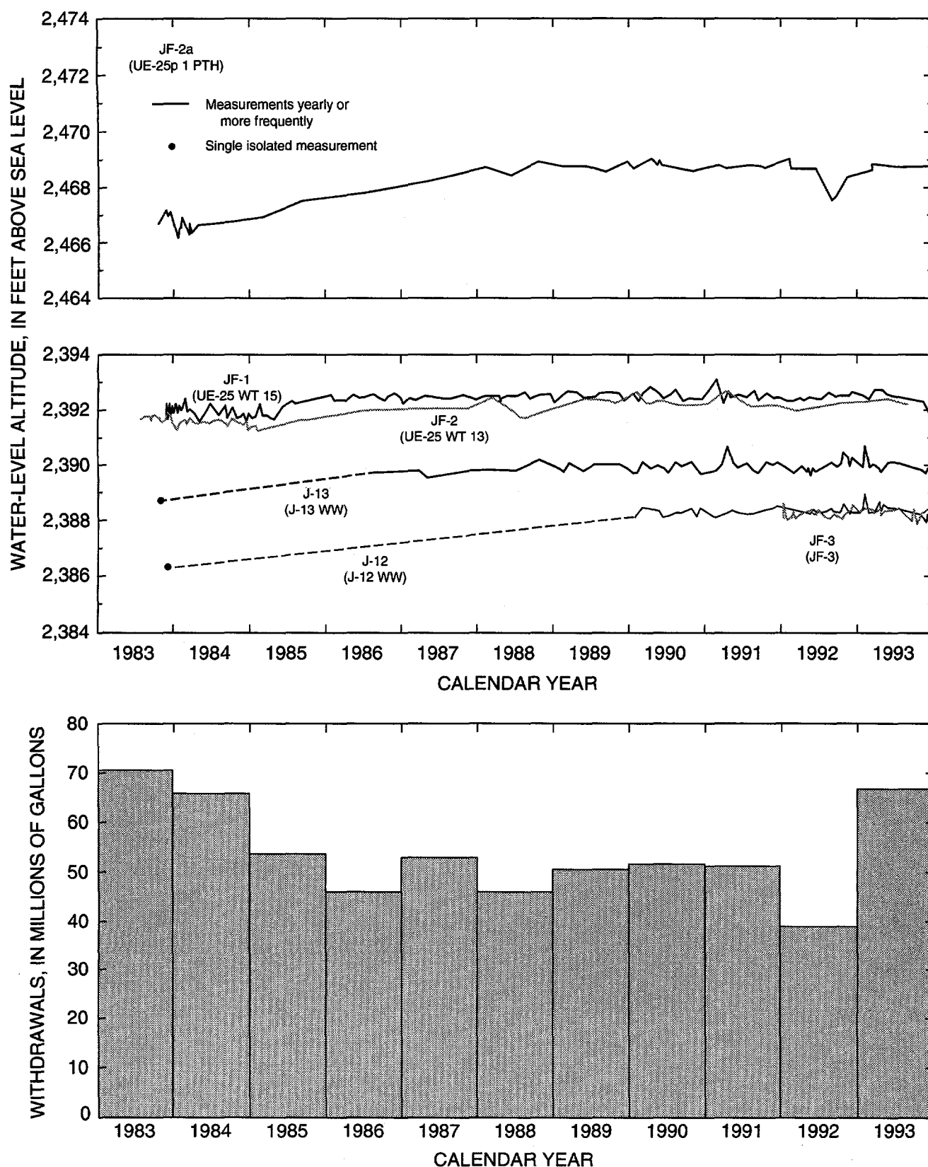
Figure 12. Water-level altitudes in wells JF-1, JF-2, J-13, J-12, JF-3, and JF-2a, 1983 through 1993. Lines connect discrete water-level altitudes listed in table 2 of La Camera and Westenburg (1994) and table 5 in this report, and are dashed where no measurements were available for consecutive calendar years. Data that may represent transient conditions at a site have been excluded (see section titled "Presentation of Ground-Water Data"). A single measurement in JF-2a (November 7, 1983) has been excluded, as that measurement may represent transient conditions at the site. Estimated ground-water withdrawals from Jackass Flats, 1983 through 1993. Bar height equals sum of withdrawals from water-supply wells J-12 and J-13.
