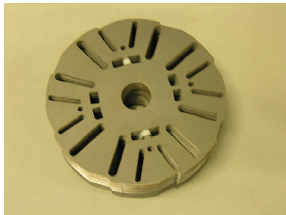
Figure 16. Rotor punching.
