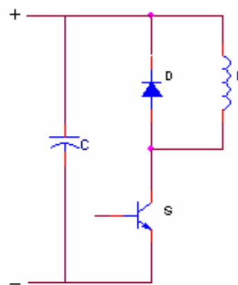
Figure 3. Test circuit for dynamic characterization.
