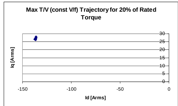
Figure 26. Maximum torque/volt current vector trajectory for SPM1 machine at 20% of rated torque.
