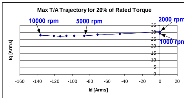
Figure 25. Maximum torque/amp current vector trajectory for SPM1 machine at 20% of rated torque.
