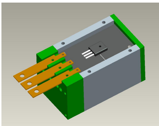
Figure 5. Temperature-controlled box used for high-temperature testing.
