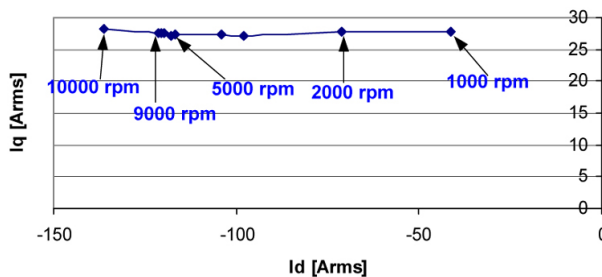
Figure 31. Current vector trajectory for SPM1 machine to deliver maximum partial-load efficiency at 20% of rated torque.
