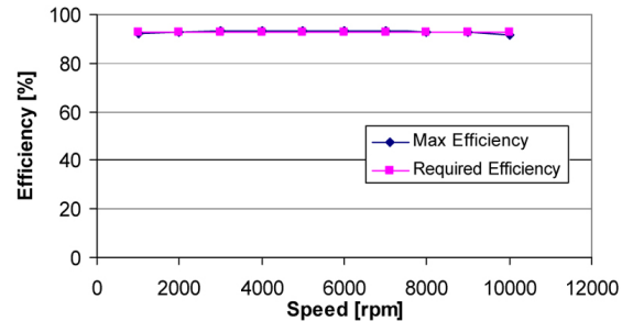
Figure 32. Predicted efficiency of SPM1 machine at 20% of rated torque for maximum partial-load efficiency, plus specified minimum efficiency line.
