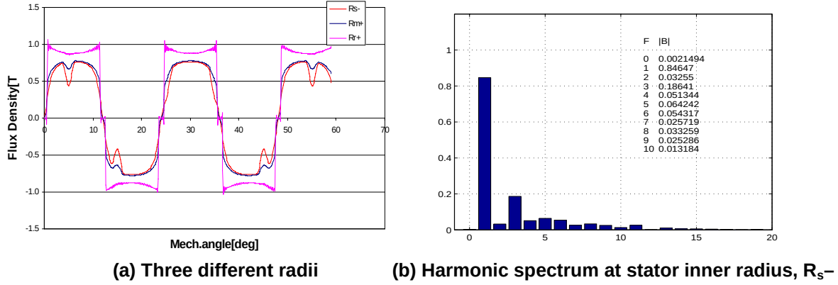
Figure 19. Analytical predictions of the spatial air-gap flux density distribution for a slotted version of the SPM1 machine for a rotor angular position of 5 mechanical degrees.
