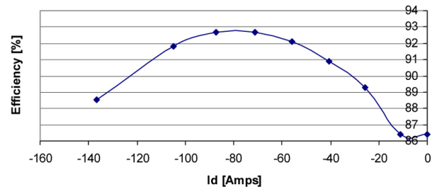
Figure 30. Variation of SPM1 efficiency at 2000 rpm as a function of i_d with i_q adjusted to hold the torque constant at 20% of rated torque.
