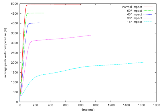
Figure 1. Peak temperatures for various impact angles.
