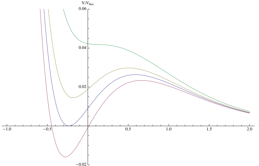
Figure 1: The potential V(\hat{\tau})/V_{\text{flux}} with (\bar{m}_P = 1) B_3 = 1/4 , B_0 = 1/4 , B_4 = 3/8 , B_{O_6} = 2 , and \rho satisfying \partial V/\partial \rho = 0 . From bottom to top, the curves correspond to the following choices of c : 2.183 (anti-de Sitter), 2.205 (Minkowski), 2.227 (de Sitter), and 2.280 (inflection), respectively.
