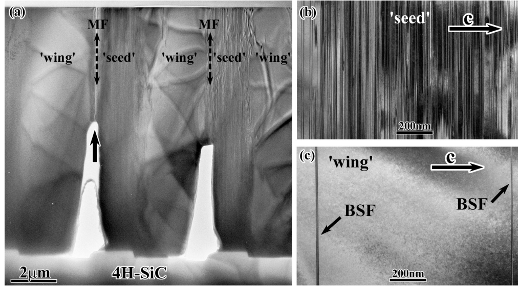
Figure 9. (a) Cross-sectional TEM image of a coalesced a-plane pendeo-epitaxial GaN layer grown on (1120) 4H-SiC substrate. Cracks (marked by arrow) are often observed at meeting fronts (MF) of two adjacent 'wings'. Distribution of basal stacking faults in the 'seed' (b) and in the 'wing' areas (c) is shown with higher magnification. Note decrease of basal stacking fault densities in the 'seed' area in comparison to the 'wing' area.
