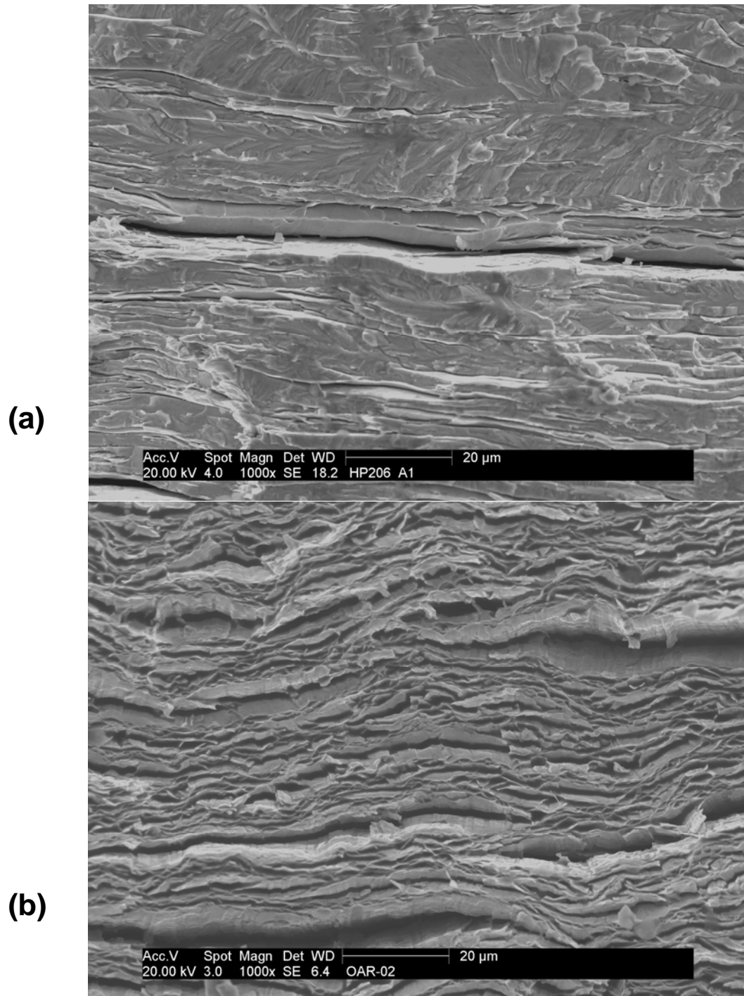
Figure 2. SEM Fractography from the fracture surface of a non-irradiated LAW tensile specimens tested at a temperature near the DBTT: (a) unalloyed HP-LCAC molybdenum tested at -150^{\circ}\text{C} , and (b) LAW ODS molybdenum tested at -150^{\circ}\text{C} .
