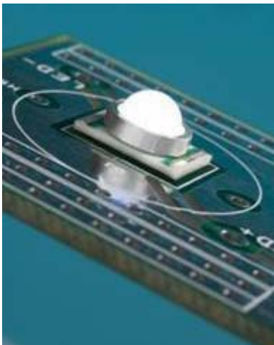
Figure 13: White-emitting 7090 XLamp built with latest generation blue LED chip and yellow phosphor. Up to 94 lumens at 86 lumens per watt was achieved at a drive current of 350 mA.
