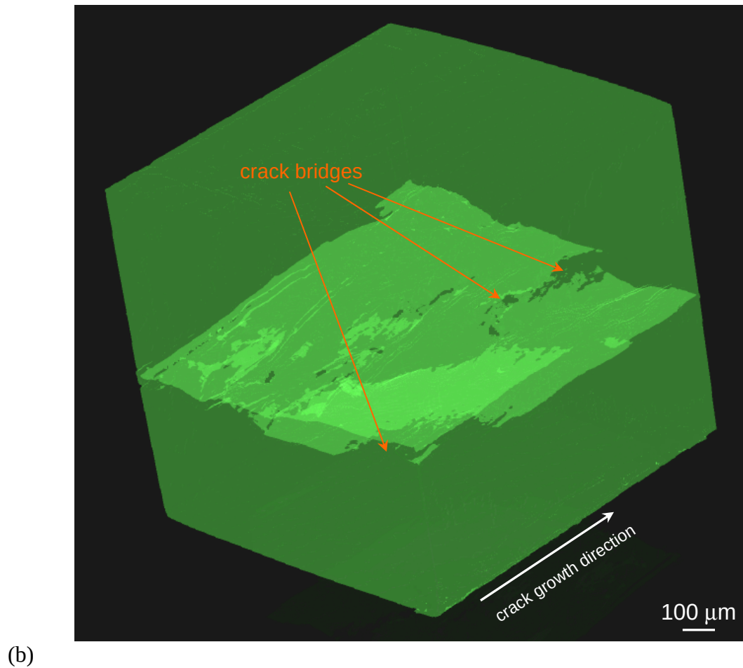
Figure 4: (a) An optical micrograph showing the development of crack bridging in dentin dehydrated using whisky. Microcracks (“daughter cracks”), initiated primarily at tubules, form ahead of the main crack (“mother crack”); their inability to link perfectly with the main crack leads to regions of uncracked material which spans the crack. Such “uncracked ligaments” carry load that would otherwise be used to drive the crack, and thereby act to tough the dentin. (b) A three-dimensional x-ray tomography reconstruction of a section of the crack in (a), showing the three-dimensional nature of the uncracked-ligament bridging. The nominal direction of crack growth is indicated in both cases.
