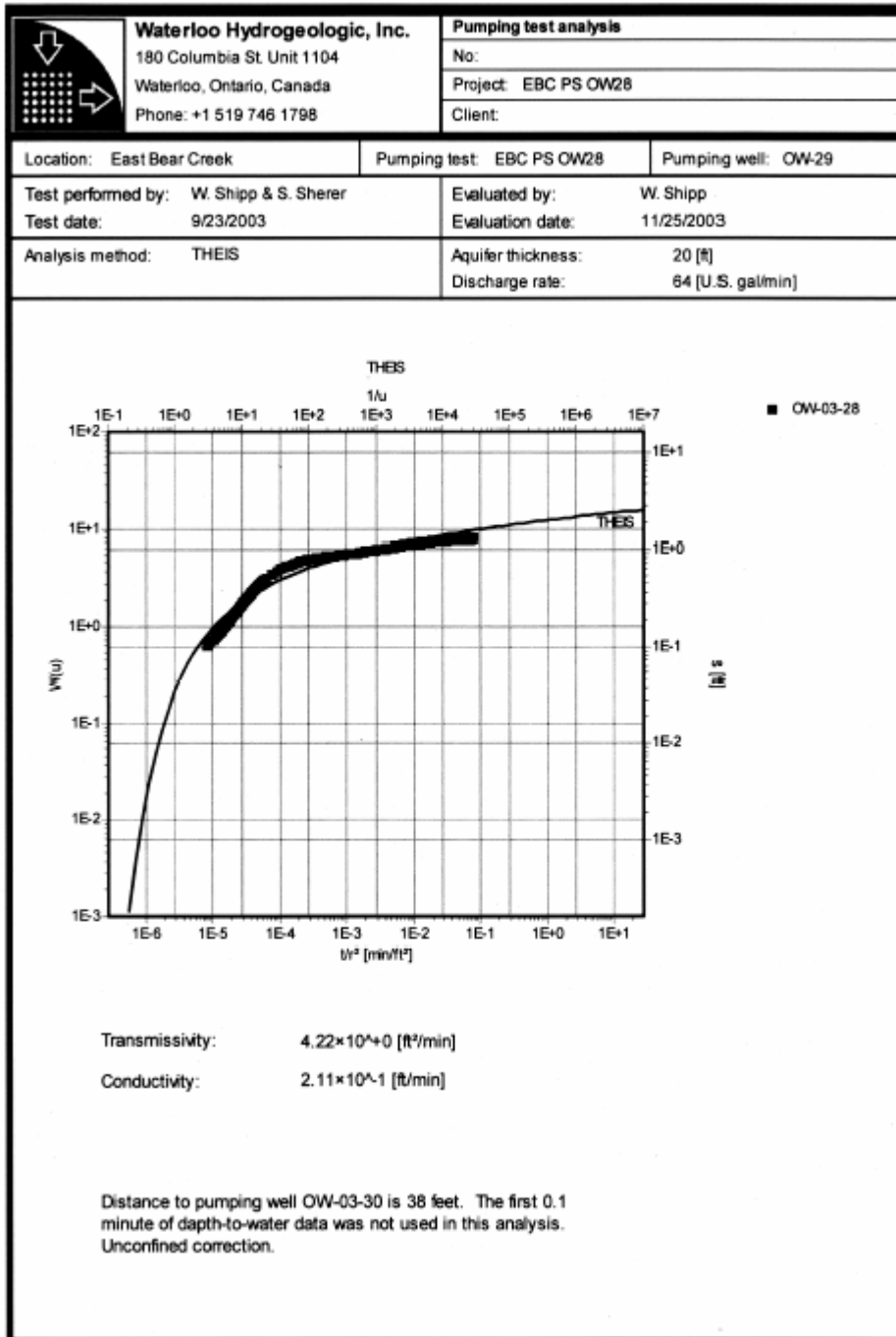
Figure A5. Theis analysis from pump test data from observation well OW-03-28 during pumping test at well OW-29
