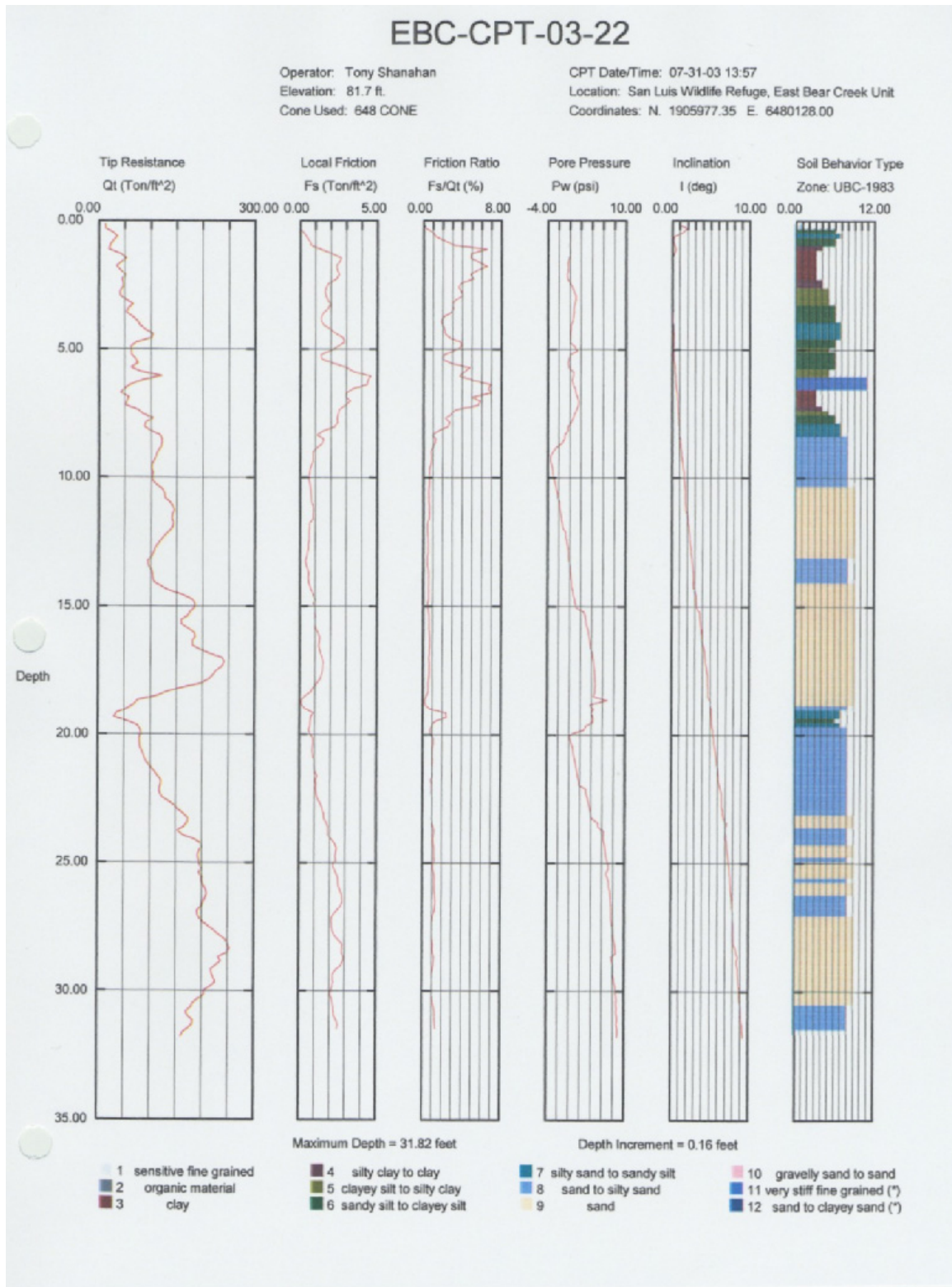
Figure 16. CPT Log CPT-03-22 in the East Bear Creek Unit of the San Luis NWR Complex.
