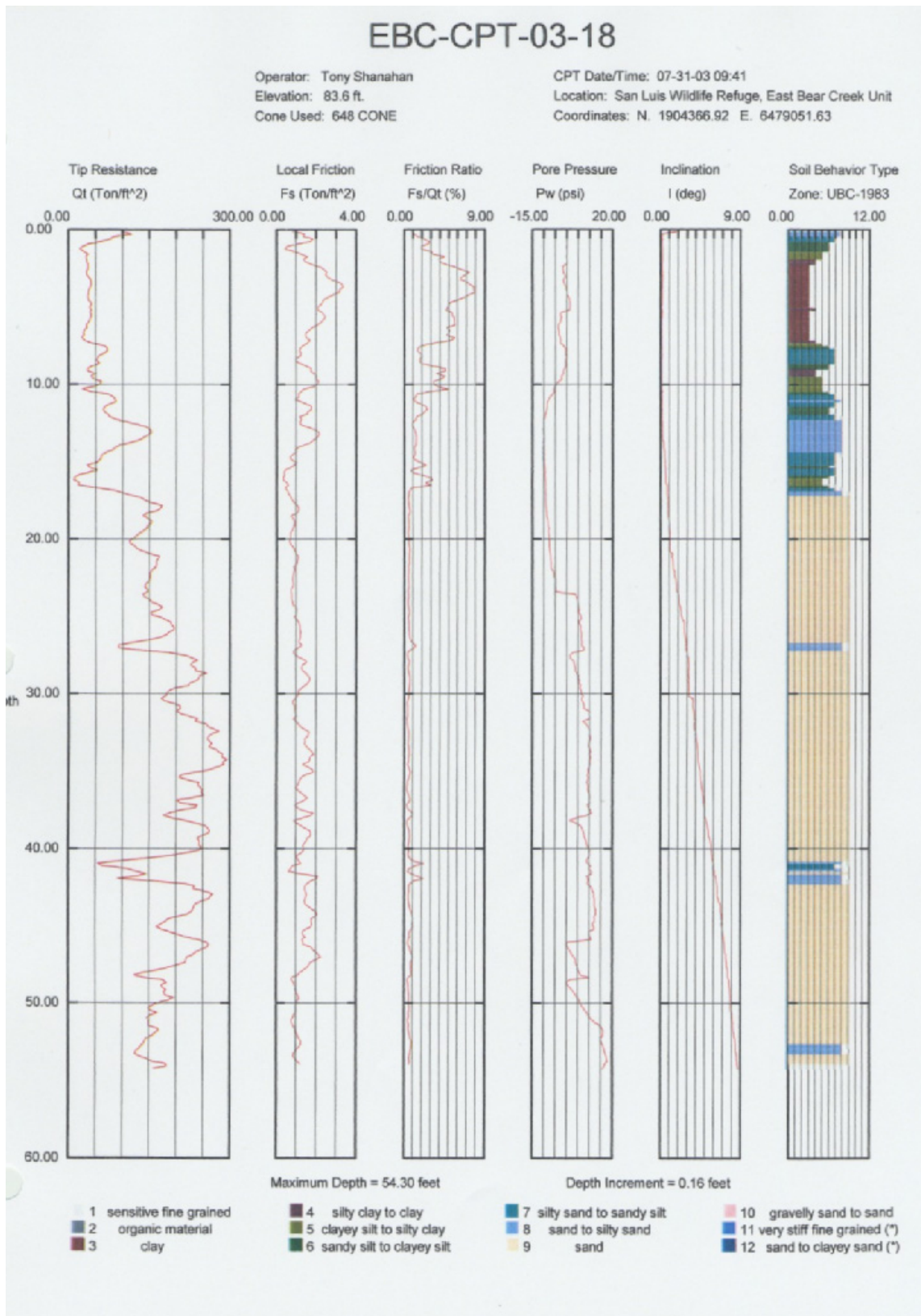
Figure 12. CPT Log CPT-03-18 in the East Bear Creek Unit of the San Luis NWR Complex
