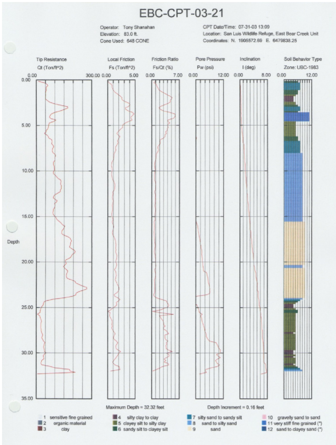
Figure 15. CPT Log CPT-03-21 in the East Bear Creek Unit of the San Luis NWR Complex
