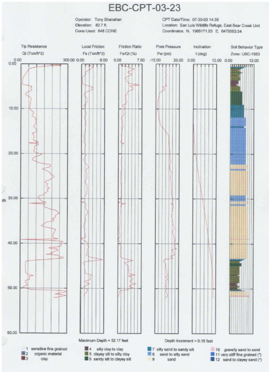
Figure 17. CPT Log CPT-03-23 in the East Bear Creek Unit of the San Luis NWR Complex.
