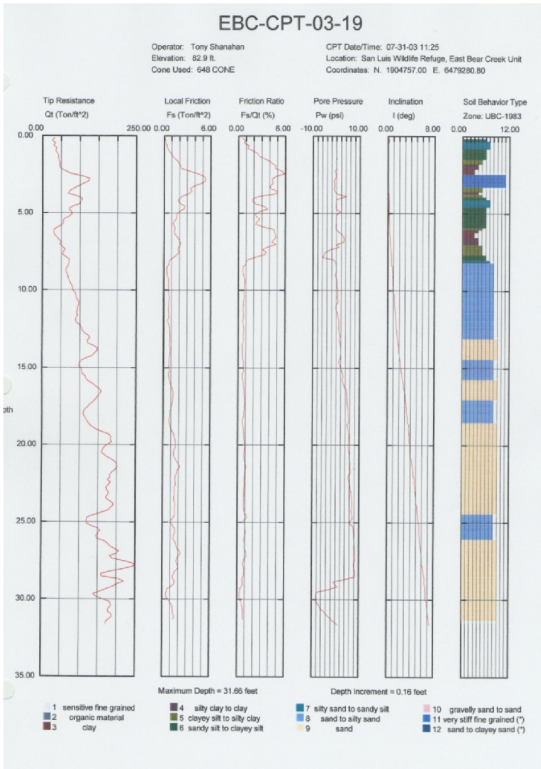
Figure 13. CPT Log CPT-03-19 in the East Bear Creek Unit of the San Luis NWR Complex
