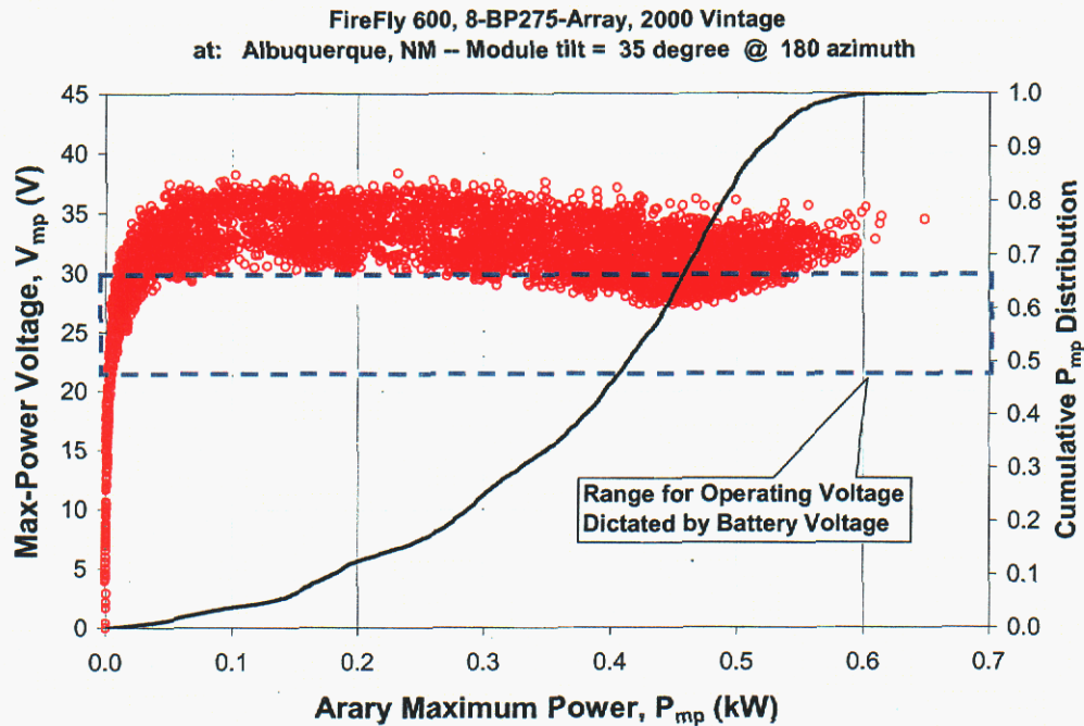
Figure 7a. Scatter plot of hourly values for array V_{mp} as a function of array P_{mp} for year long operation in Albuquerque, with array oriented at a latitude tilt-angle. Array operating voltage will be constrained by battery voltage within the range shown (21.6 to 30 Vdc). The cumulative distribution curve indicates the fraction of the annual energy available as a function of array P_{mp} .
