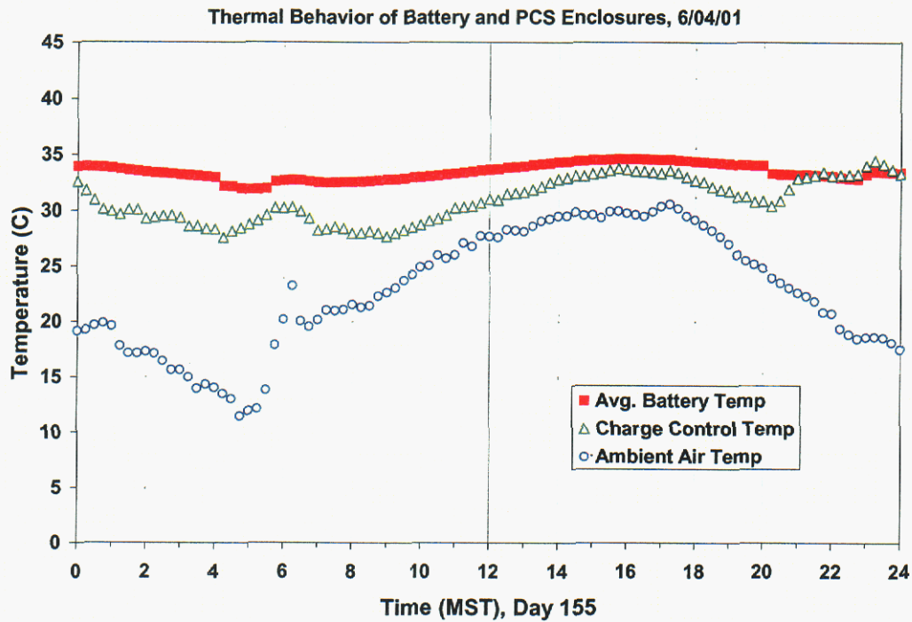
Figure 22. Temperature measurements recorded for battery, charge-controller fin, and ambient temperature during ‘recovery’ from low-voltage-disconnect condition. Lid closed on battery enclosure with battery at about 50% SOC.
