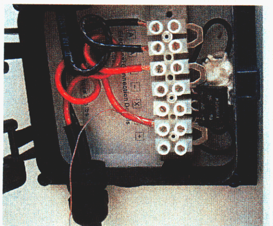
Figure 14. Photo of BP275 module junction box showing wiring, bypass diode, and thermocouple attached to lower wire near terminal lug.
