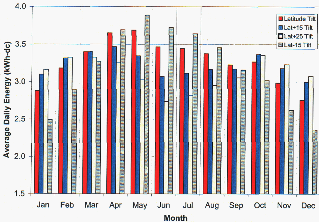
Figure 5. Calculated dc energy available (kWh/d) from the FireFly™ 600 array of BP Solar BP275 modules when located in Albuquerque, pointed south, and oriented at different array tilt-angles.
