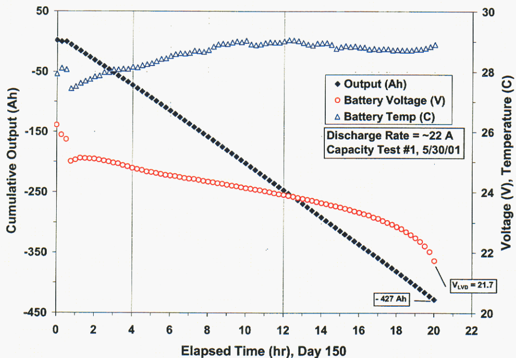
Figure 28. First measurement of 'usable' battery capacity performed during system test procedure. The V_{LVD} setpoint was controlled by the Trace DR2424 inverter.
