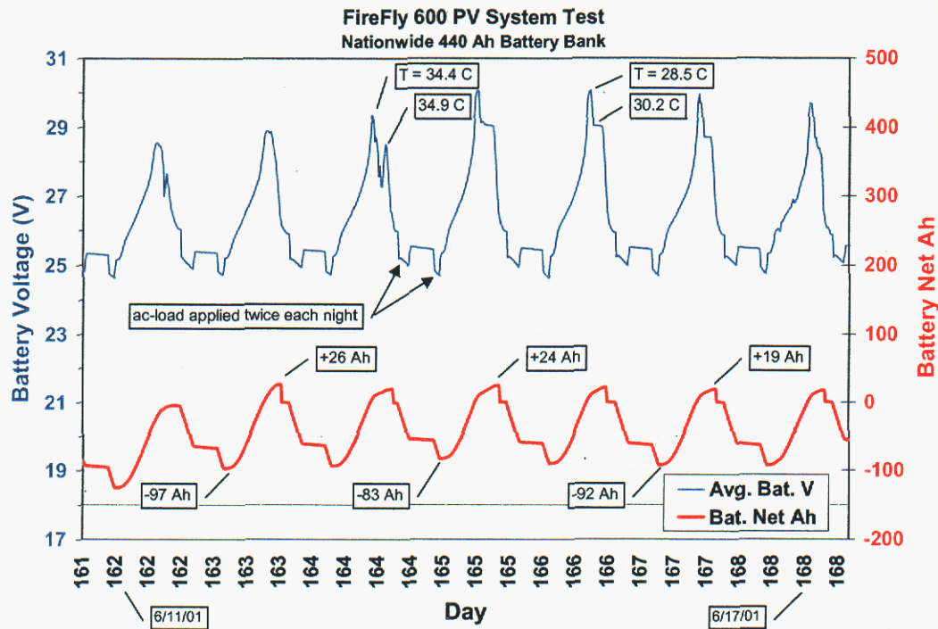
Figure 38. Battery voltage and net amp-hour flow into and out of battery bank during the daily 'cycling' at the end of the first 'recovery' test.
