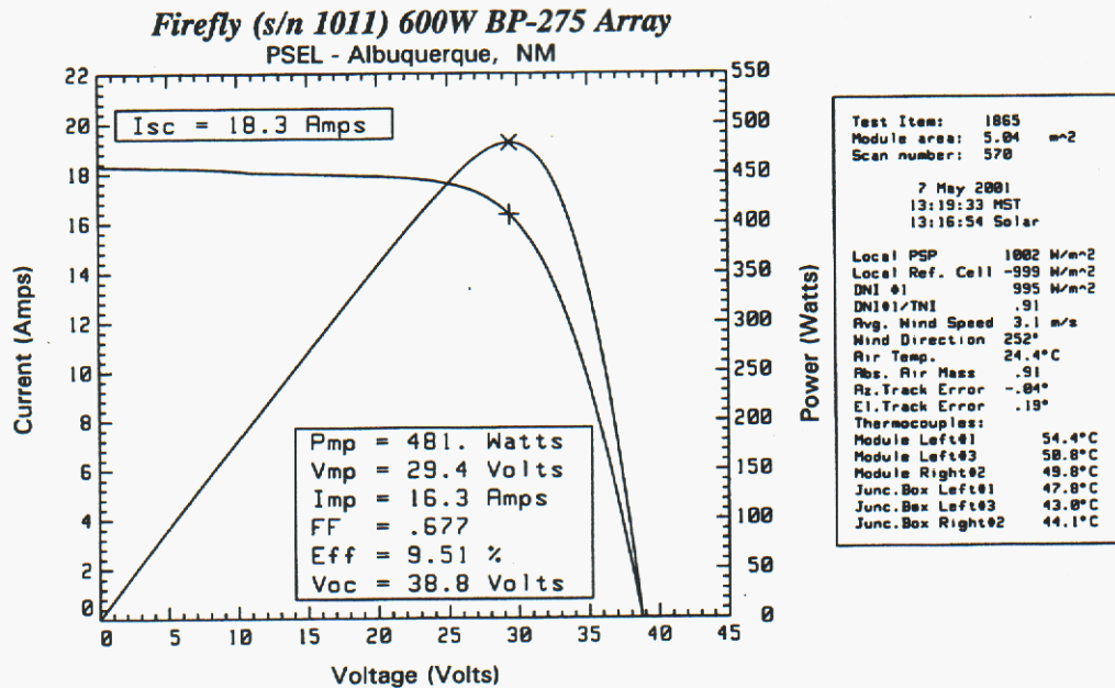
Figure 3a. A typical current-voltage (I-V) curve measurement at 1002 W/m 2 solar irradiance and 52°C module temperature for eight BP Solar BP275 c-Si modules, array pointed south and oriented at a latitude tilt-angle (35 deg).
