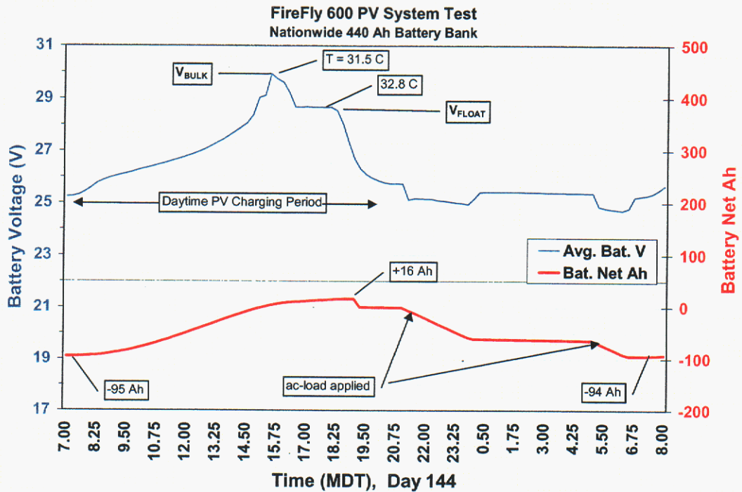
Figure 36. Example of a daily 'cycle' illustrating the 3-stage charging process (bulk, 1-hr absorption, float) controlled by the Trace C40 charge controller. The effect of applying the ac load at two different times during the night is shown.
