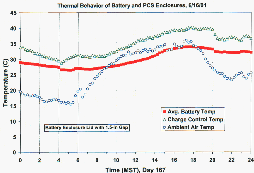
Figure 24. Temperature measurements recorded for battery, charge-controller fin, and ambient temperature during typical ‘cycling’ condition. Lid on battery enclosure was raised for ventilation with battery at a full state-of-charge.
