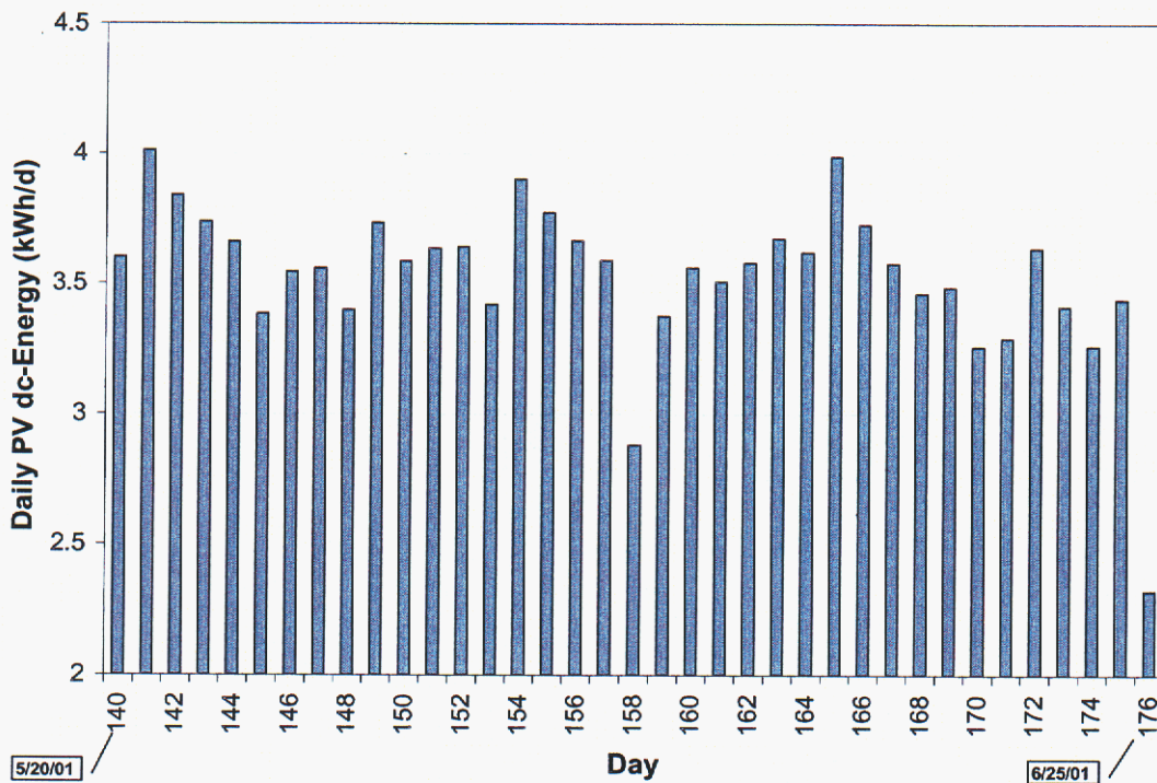
Figure 34. Calculated daily energy available at P_{mp} from the FireFly™ 600 array during the system performance test period, based on empirical array performance model.
