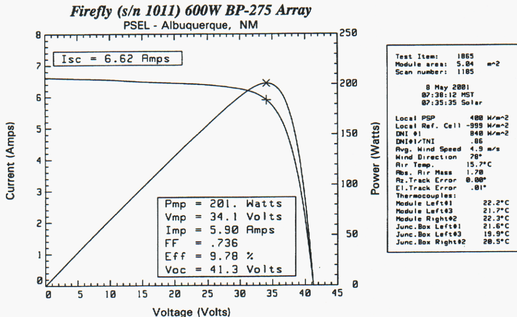
Figure 3b: Typical current-voltage (I-V) curve measurement at 400 W/m 2 solar irradiance and 22°C module temperature for eight BP Solar BP275 c-Si modules, array pointed south and oriented at a latitude tilt-angle (35 deg).
