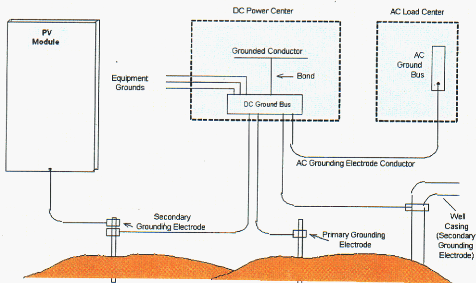
Figure 1. Grounding Electrodes
