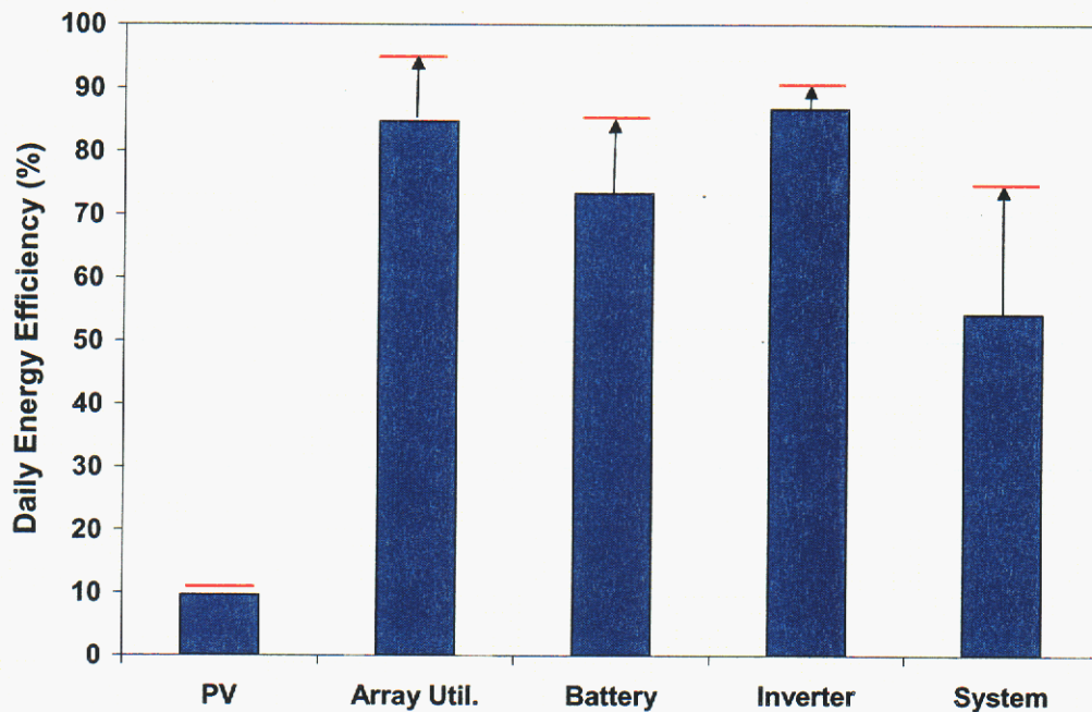
Figure 42. Daily energy efficiency measurements for the FireFly™ 600 components and system during the 30-day test period in June in Albuquerque, using a 'conservative' ac load. Arrows indicate range for potential improvement through system optimization.
