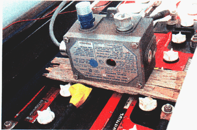
Figure 19. General Monitors hydrogen concentration sensor positioned above batteries in the FireFly™ 600 battery enclosure.
