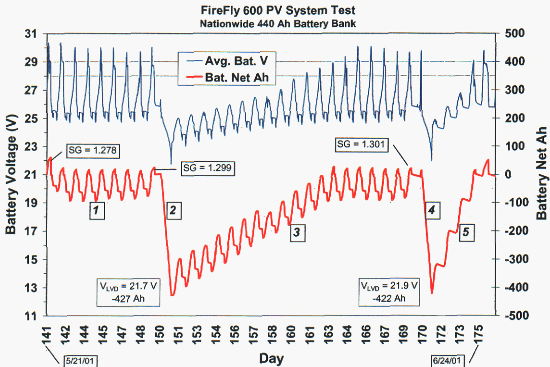
Figure 32. Battery voltage and net amp-hours during the five steps of the system test procedure: (1) initial cycling, (2) battery capacity test, (3) first recovery, (4) battery capacity test, and (5) second recovery.
