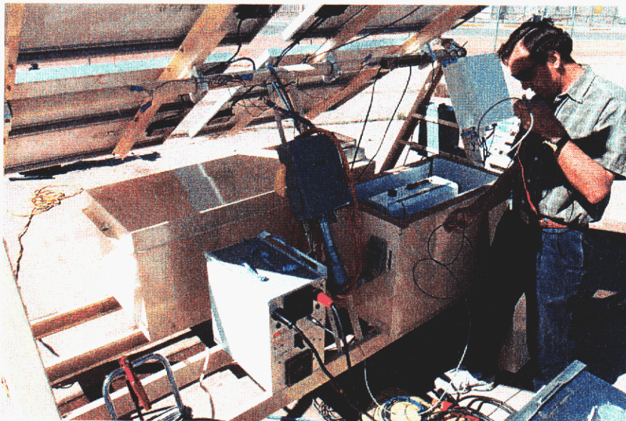
Figure 16. FireFly™ 600 photovoltaic off-grid system during performance testing at Sandia.
