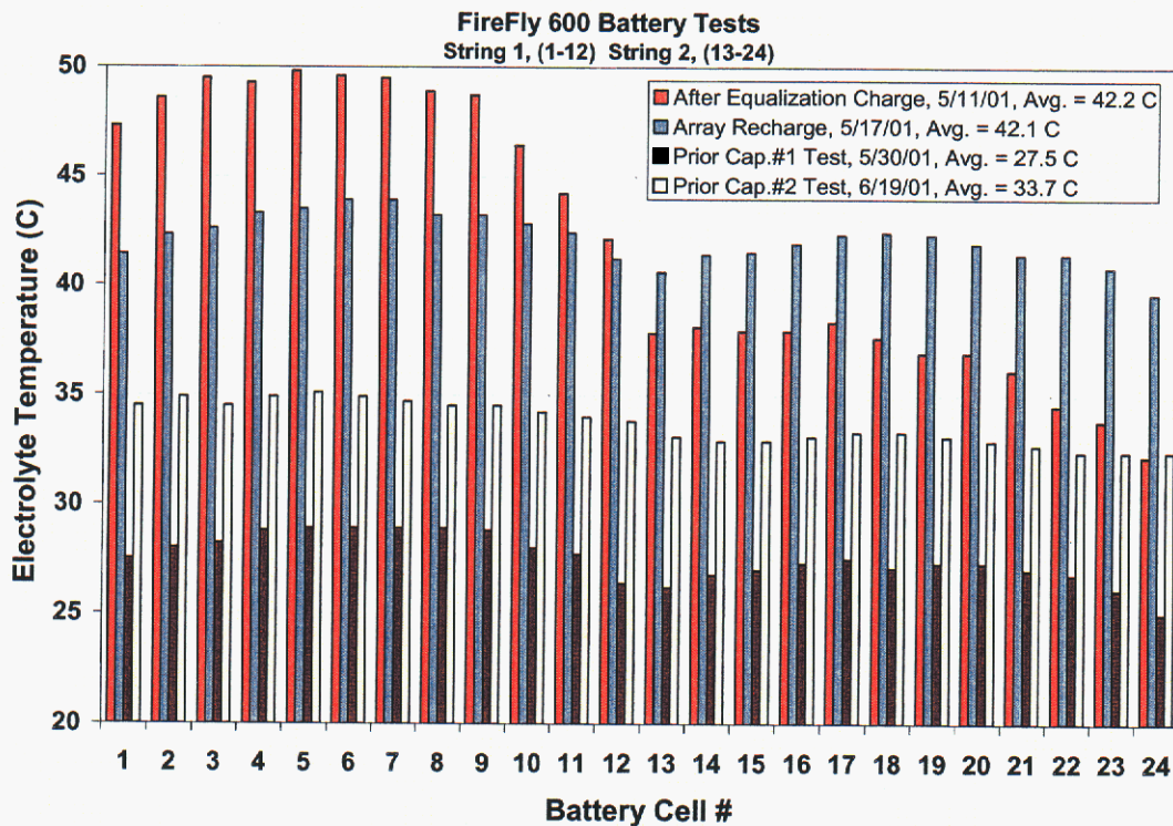
Figure 26. Electrolyte temperature measurements for individual cells in the battery bank recorded at different times in the system test sequence.
