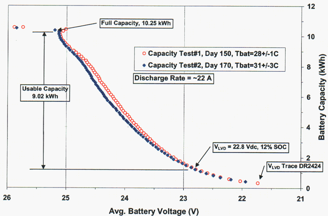
Figure 30. Measured battery capacity in units of kWh versus average battery voltage. The recommended V_{LVD} and the value actually used by Trace DR2424 inverter are indicated.
