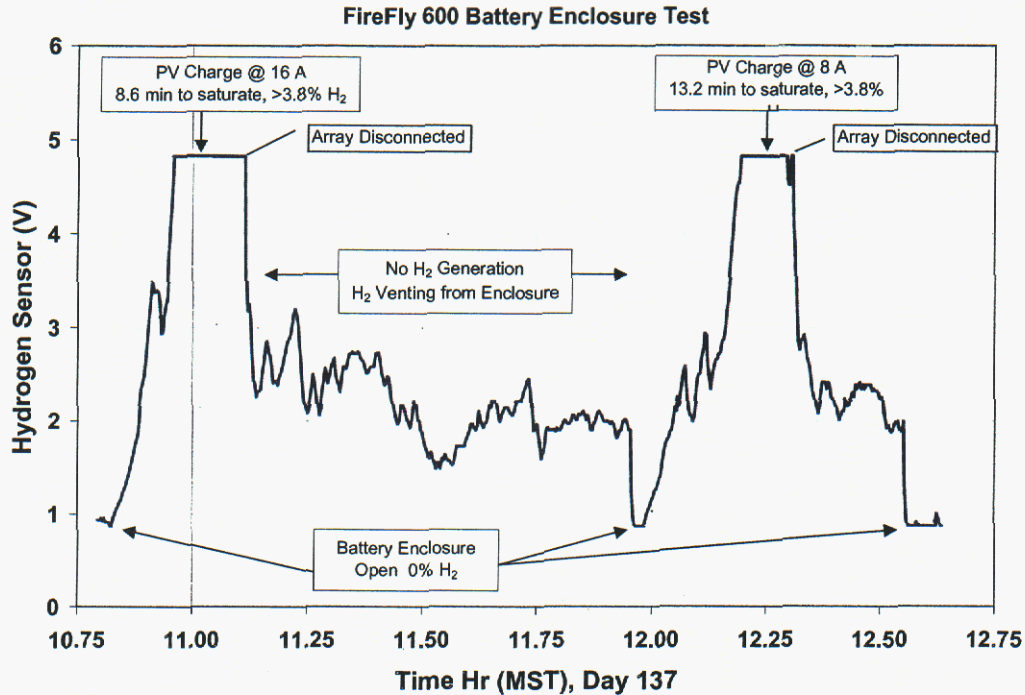
Figure 20. Hydrogen concentration measurement inside the FireFly™ 600 battery enclosure, near full state-of-charge with battery temperature about 35 °C. Note: A hydrogen sensor voltage of 4.8 V corresponded to a hydrogen concentration of 3.8%, and 0.9 V corresponds to 0% hydrogen.
