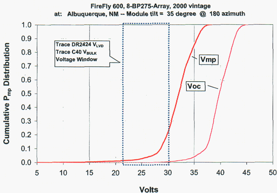
Figure 7b. Cumulative distribution of annual energy available from FireFly 600 array related to the array's maximum-power voltage ( V_{mp} ) and open-circuit voltage ( V_{oc} ). The system "voltage window" defining the range for actual operating voltages is also shown. (Albuquerque, NM)
