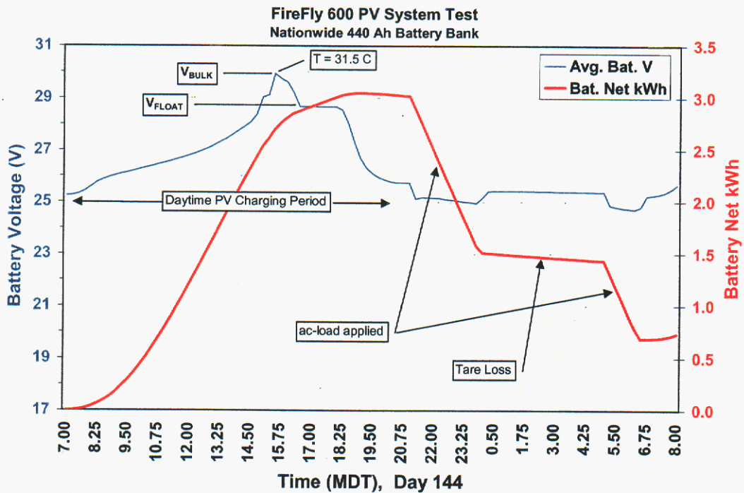
Figure 37. Example of a daily 'cycle' illustrating the 3-stage charging process controlled by the Trace C40 charge controller. Energy balance (kWh) indicated that 30% more energy was put into battery than was withdrawn.
