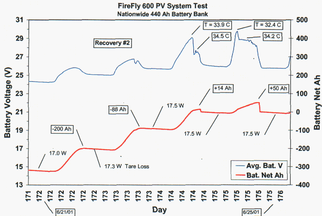
Figure 40. Battery voltage and net amp-hour flow into and out of battery bank during the second 'recovery' test without ac load applied to the system.
