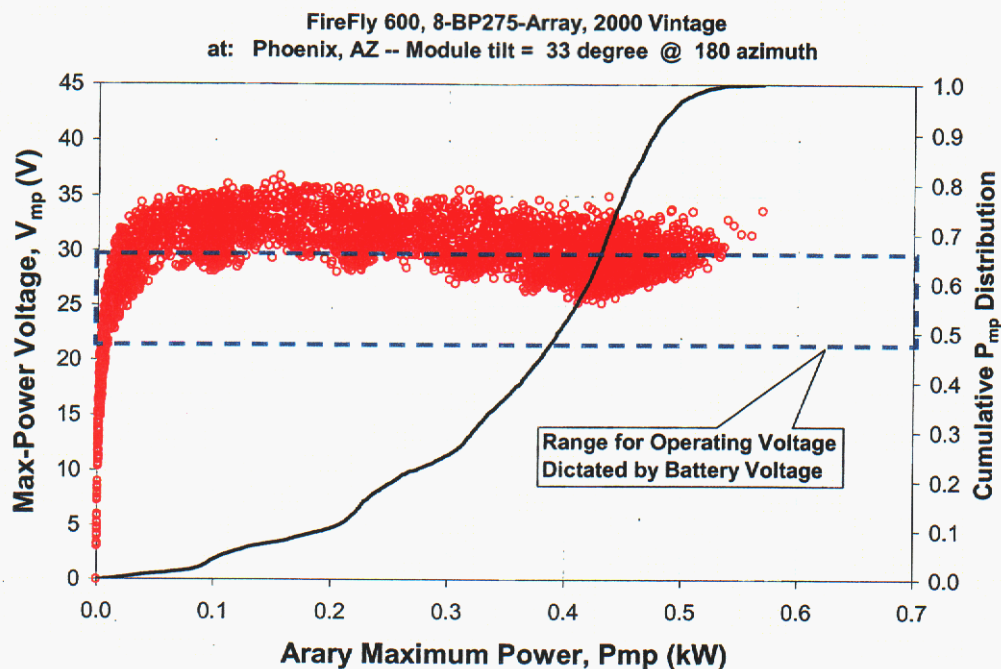
Figure 8a. Scatter plot of hourly values for array V_{mp} as a function of array P_{mp} for year long operation, with array oriented at a latitude tilt-angle. The system “voltage window” defining the range for actual operating voltages is also shown. (Phoenix, AZ)
