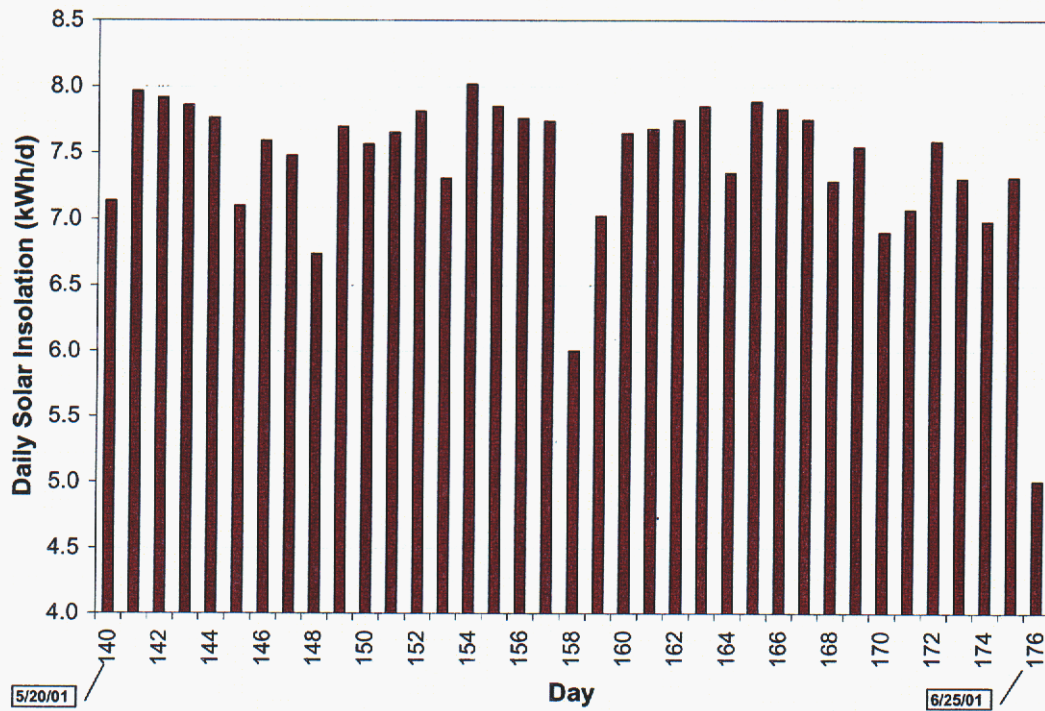
Figure 33. Measured daily solar energy (insolation) in the plane-of-array during the system performance tests for the FireFly™ 600 system.
