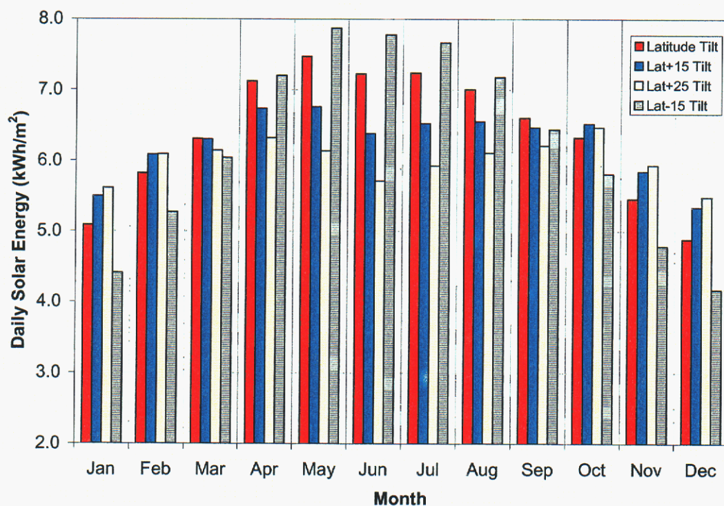
Figure 4. Calculated daily-average solar resource ( \text{kWh/m}^2 ) available to the FireFly™ 600 array when located in Albuquerque, pointed south, and oriented at different array tilt-angles. (TMY2 solar resource from NSRDB)
