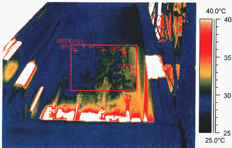
Figure 27. Thermal infrared (IR) image showing temperature distribution between string #1 (right) and string #2 following battery recharge using the PV array. White regions across the image are sunlight shining between the halves of the array.
