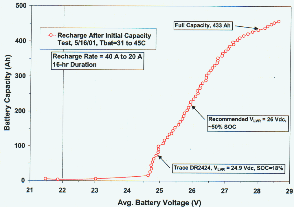
Figure 31. Battery capacity versus battery voltage, measured while recharging from a low-voltage-disconnect condition. A recommended V_{LVR} and the value actually used by the Trace DR2424 inverter are indicated.
