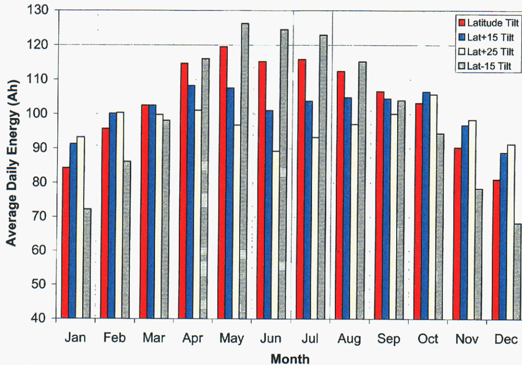
Figure 6. Calculated daily dc amp-hours available from the FireFly™ 600 array of BP Solar BP275 modules when located in Albuquerque, pointed south, and oriented at different array tilt-angles.
