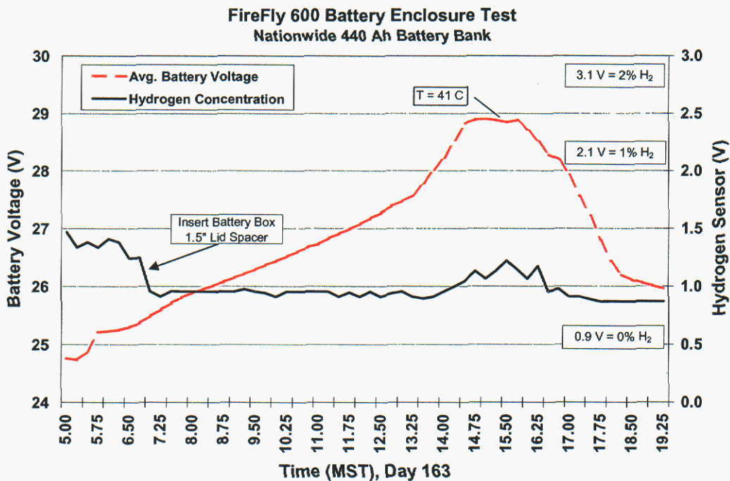
Figure 21. Measurement of hydrogen concentration with lid on battery box raised to allow ventilation around the perimeter. The result was negligible hydrogen concentration even at elevated battery temperature.
