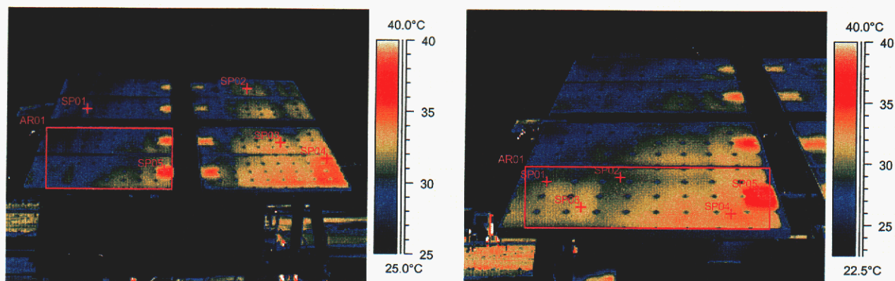
Figure 13. Temperature distribution in FireFly™ 600 array during typical operating conditions on sunny day with wind speed less than 3 m/s.
