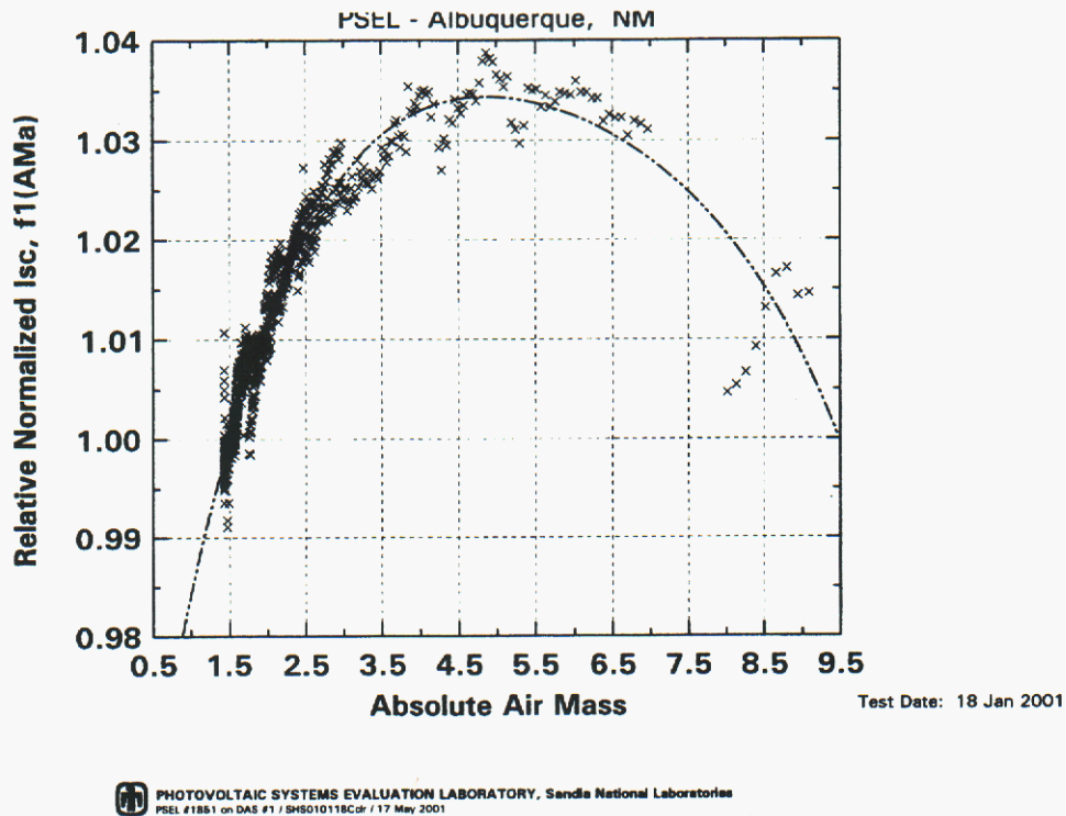
Figure 9. Empirically determined relationship for BP Solar BP275 module showing solar spectral influence on module short-circuit current ( I_{sc} ), related to absolute air mass.
