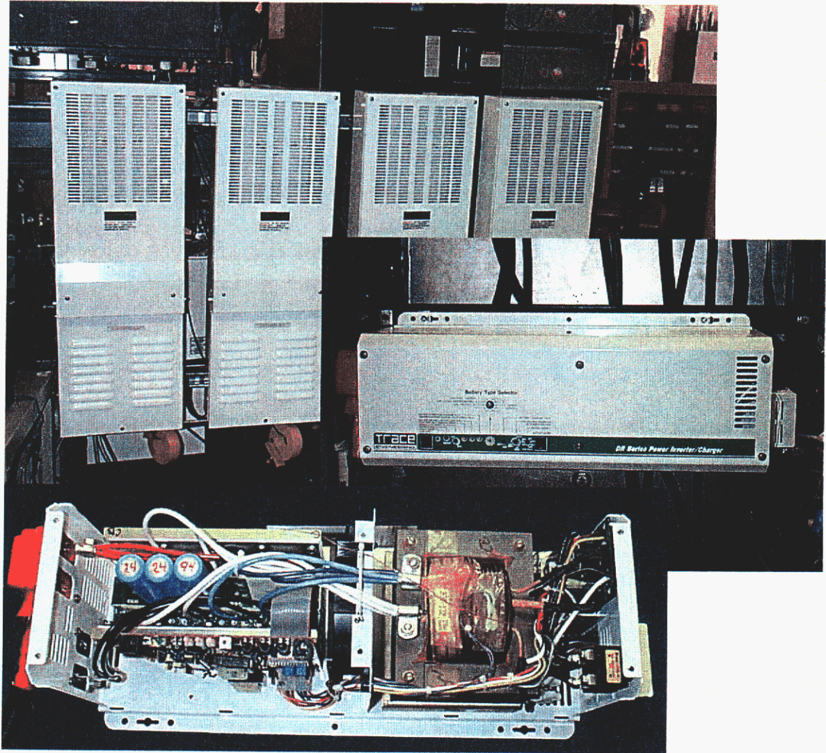
Photos of inverters being evaluated in Sandia's inverter testing laboratory.
