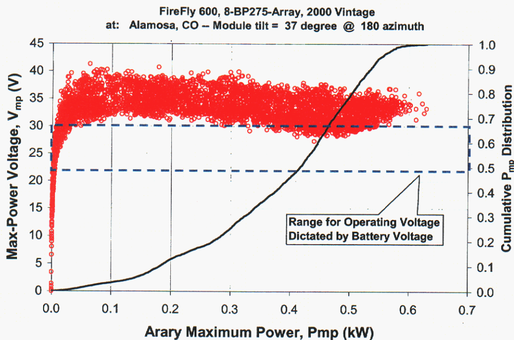
Figure 8b. Scatter plot of hourly values for array V_{mp} as a function of array P_{mp} for year long operation, with array oriented at a latitude tilt-angle. The system “voltage window” defining the range for actual operating voltages is also shown. (Alamosa, CO)
