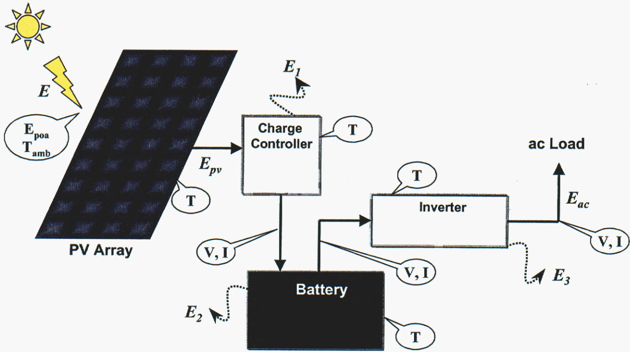
Figure 17. Schematic of an off-grid photovoltaic system indicating the flow of energy from the photovoltaic array to an ac load, including energy losses. Callout ovals indicate the measurements made during the system test procedure (irradiance, temperature, voltage, current).
