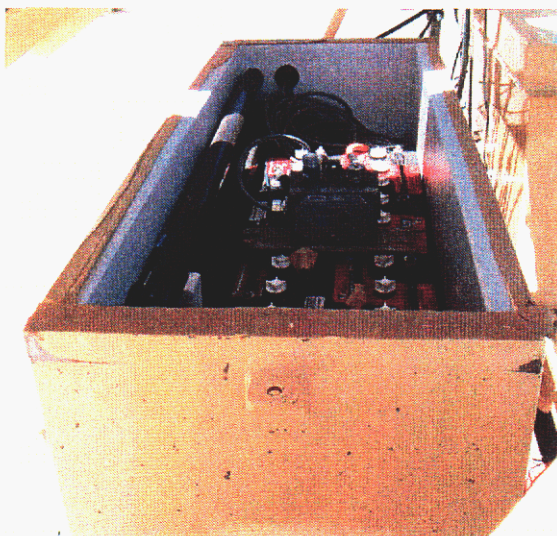
Figure 1. Photos of FireFly™ 600 photovoltaic off-grid system, insulated battery box with lid removed, insulated box containing Trace DR2424 inverter and Trace C40 charge controller, and Trace Meter used for monitoring battery state-of-charge.
