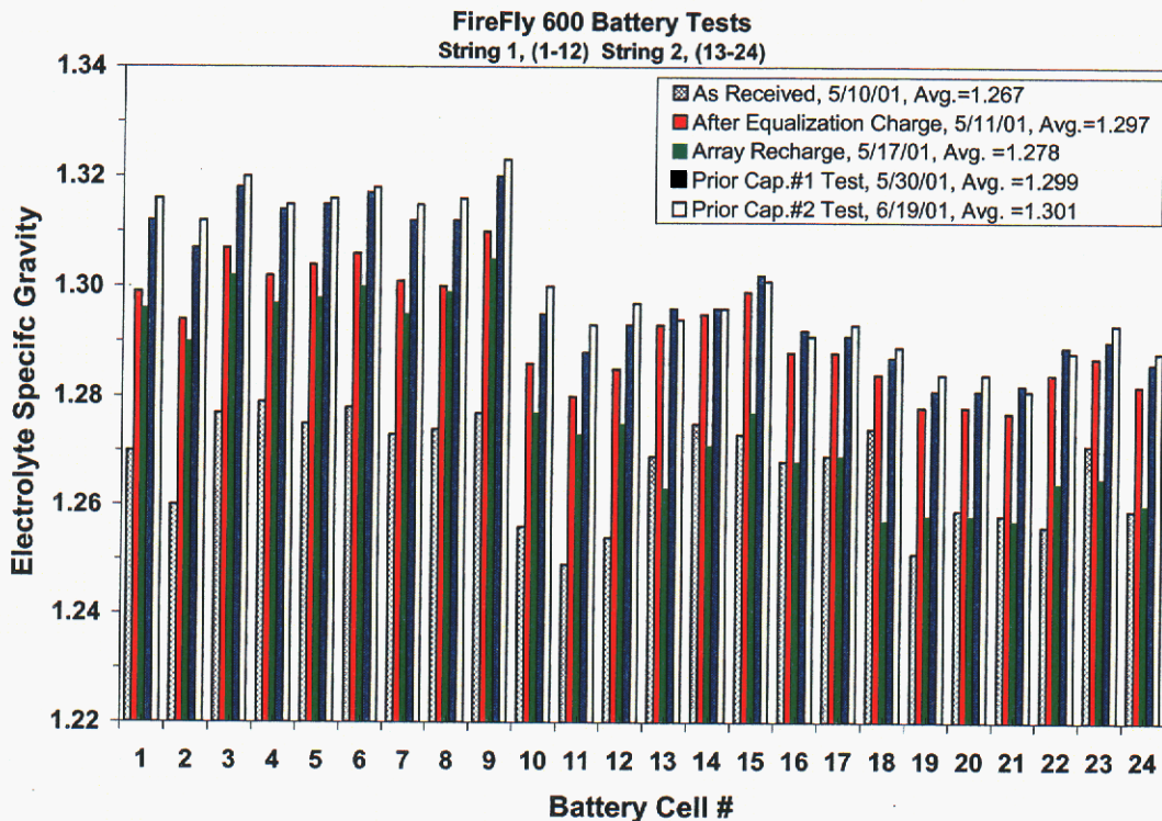
Figure 25. Electrolyte specific gravity measurements for individual cells in the battery bank recorded at different times in the system test sequence.
