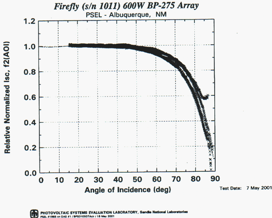
Figure 10. Empirically determined relationship showing solar angle-of-incidence influence on short-circuit current ( I_{sc} ) for the FireFly™ 600 array. A generic curve fit for modules with glass front surfaces is also shown.
