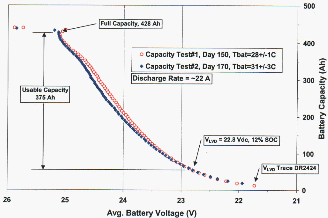
Figure 29. Measured battery capacity in units of Ah versus average battery voltage. The recommended V_{LVD} and the value actually used by Trace DR2424 inverter are indicated.
