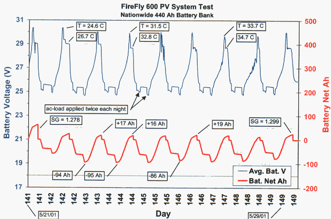
Figure 35. Battery voltage and net amp-hour flow into and out of battery bank during the initial daily 'cycling' phase of the test procedure. A variety of operating parameters are highlighted.
