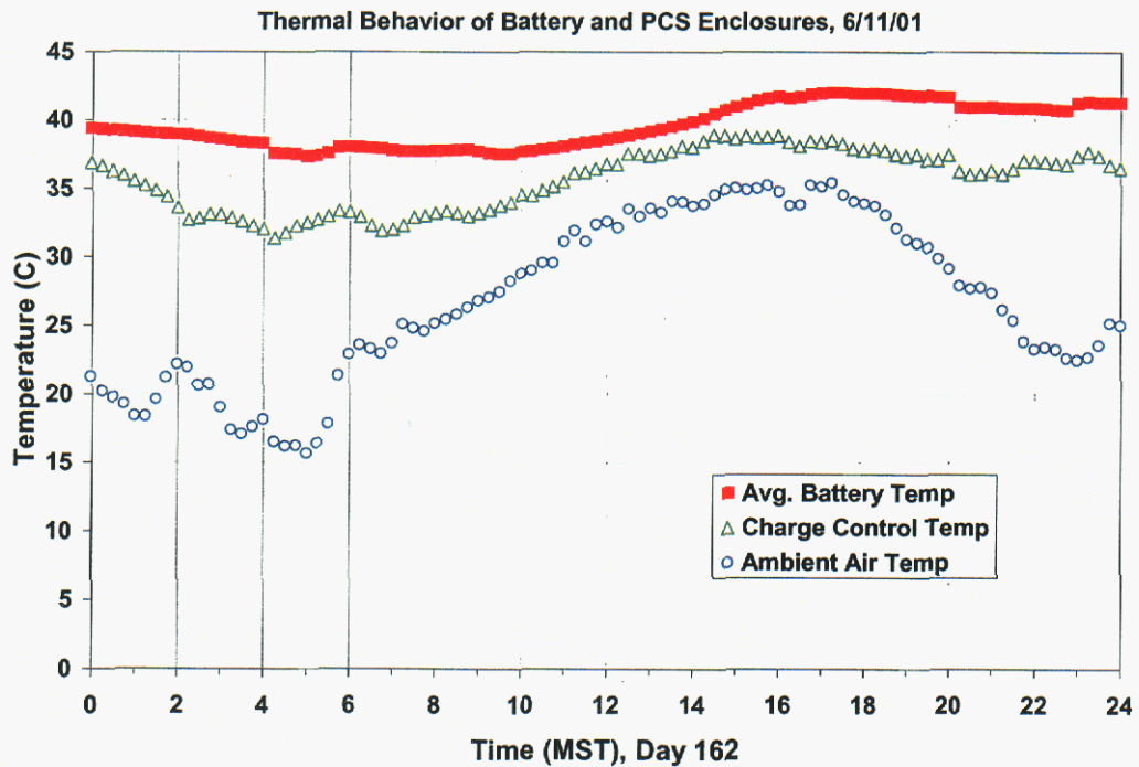
Figure 23. Temperature measurements recorded for battery, charge-controller fin, and ambient temperature during ‘recovery’ from low-voltage-disconnect condition. Lid closed on battery enclosure with battery approaching a full state-of-charge.
