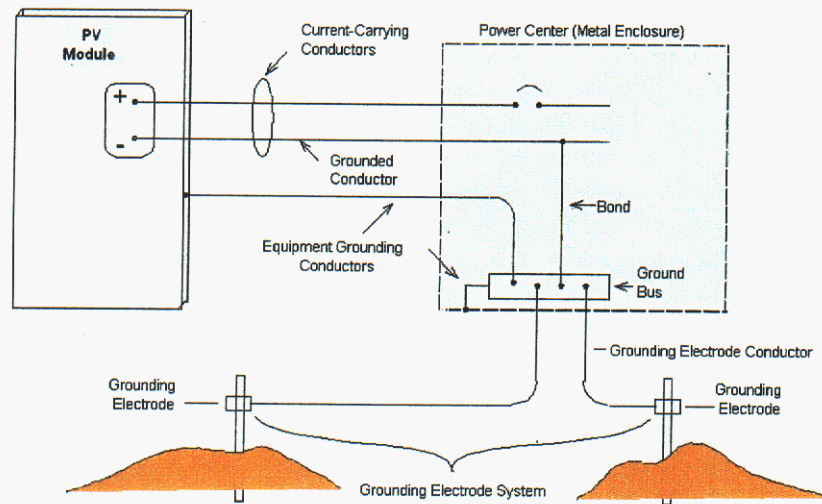
Figure 1. Grounding Electrodes
