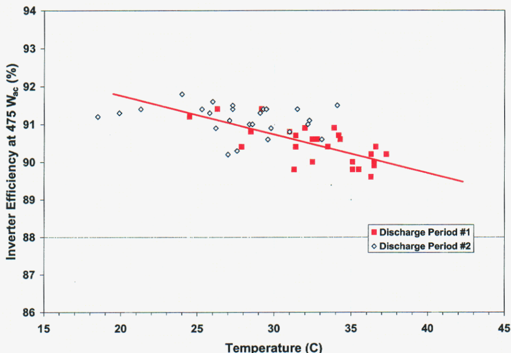
Figure 41. Instantaneous efficiency measured for Trace DR2424 inverter at 475-Wac output for a range of air temperature inside the insulated enclosure used to house the inverter.
