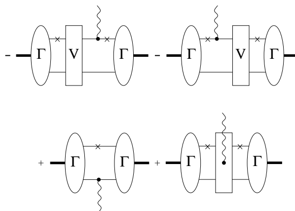
Figure 18: The original Gross effective current.
