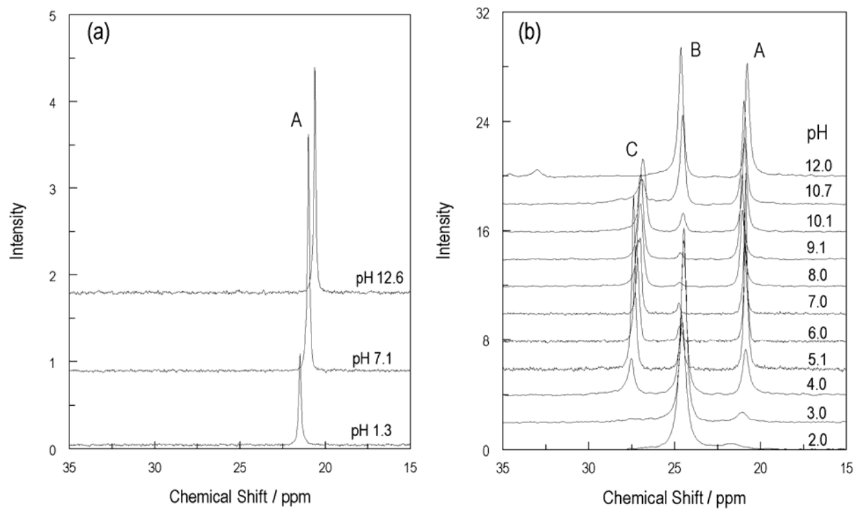
Figure 5. ^{31}\text{P}\{-^1\text{H}\} NMR spectra. (a) 40.0 mM HEDPA. (b) 10.12 mM U(VI), 20.0 mM HEDPA, \text{pH}_{\text{obs}} = 2 to 12.
