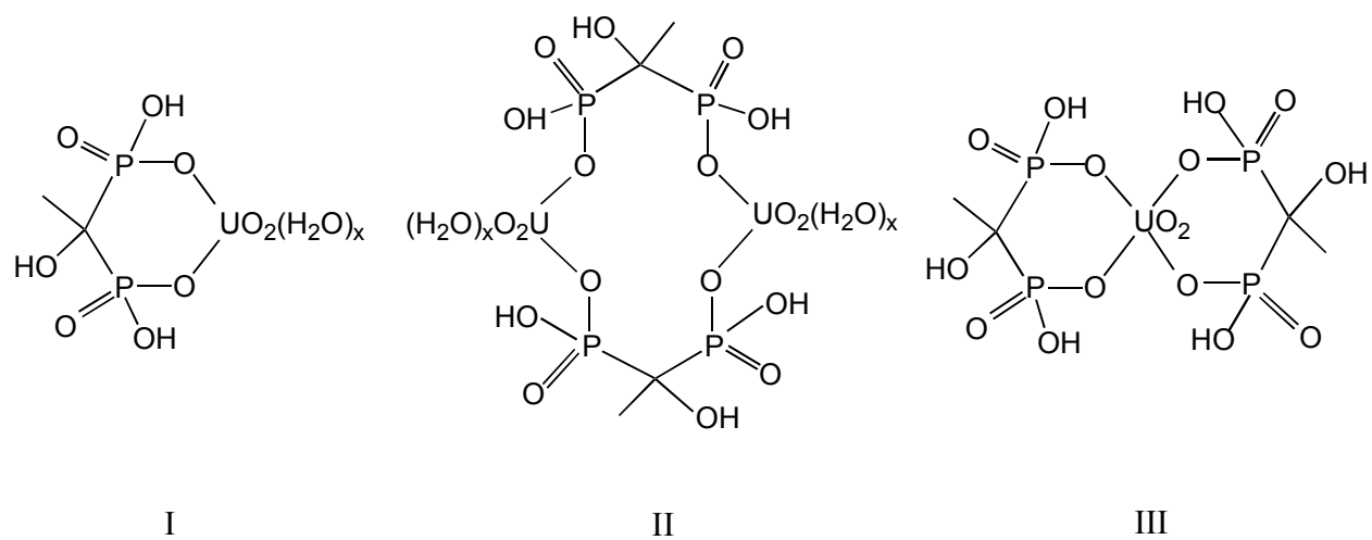
Figure 6. Proposed structures of U(VI)-HEDPA complexes. (I) a 1:1 complex, \text{UO}_2\text{H}_2\text{L} [10]; (II) a 2:2 complex, (\text{UO}_2)_2(\text{H}_2\text{L})_2 ; (III) a 1:2 complex, \text{UO}_2(\text{H}_2\text{L})_2 [10].
