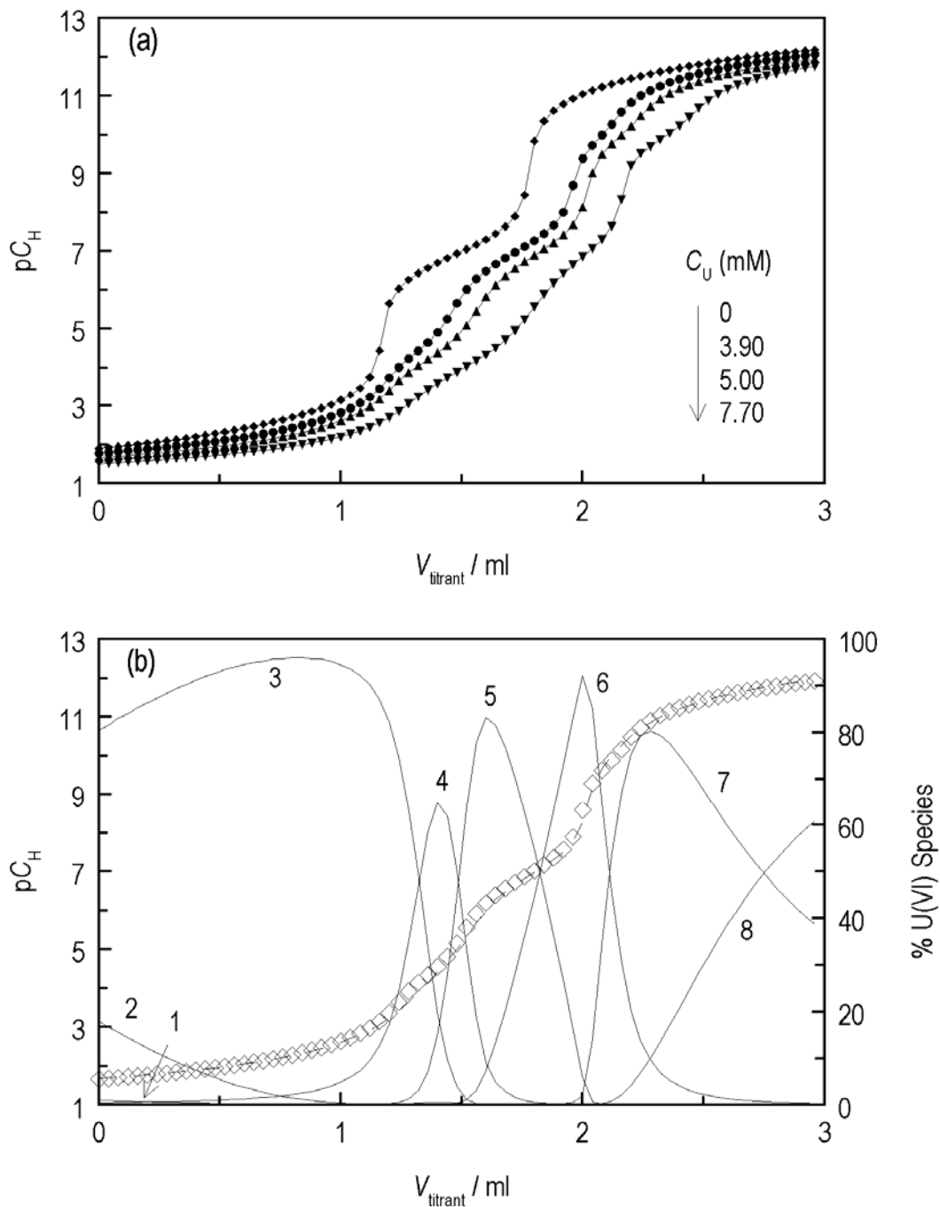
Figure 1. Potentiometric titration of U(VI)-HEDPA complexation, I = 1.0 \text{ M } (\text{CH}_3)_4\text{NCl} , t = 25^\circ\text{C} . V^0 = 40.0 \text{ mL} , titrant: 1.014 \text{ M } (\text{CH}_3)_4\text{NOH} . (a) C_{\text{HEDPA}}^0 = 15.20 \text{ mM} ; C_{\text{H}}^0 = 60 - 65 \text{ mM} ; C_{\text{U}}^0 = 0 - 7.70 \text{ mM} . (b) C_{\text{HEDPA}}^0 = 15.20 \text{ mM} ; C_{\text{H}}^0 = 61.8 \text{ mM} ; C_{\text{U}}^0 = 3.90 \text{ mM} . \diamond - experimental pC_H , left y-axis; dashed line - calculated pC_H , left y-axis; solid lines - percentages of U(VI) species, right y-axis, 1: \text{UO}_2^{2+} , 2: \text{UO}_2\text{H}_3\text{L}^+ , 3: \text{UO}_2\text{H}_4\text{L}_2^{2-} , 4: \text{UO}_2\text{H}_3\text{L}_2^{3-} , 5: \text{UO}_2\text{H}_2\text{L}_2^{4-} , 6: \text{UO}_2\text{HL}_2^{5-} , 7: \text{UO}_2\text{L}_2^{6-} , 8: \text{UO}_2(\text{OH})\text{L}_2^{7-} .
