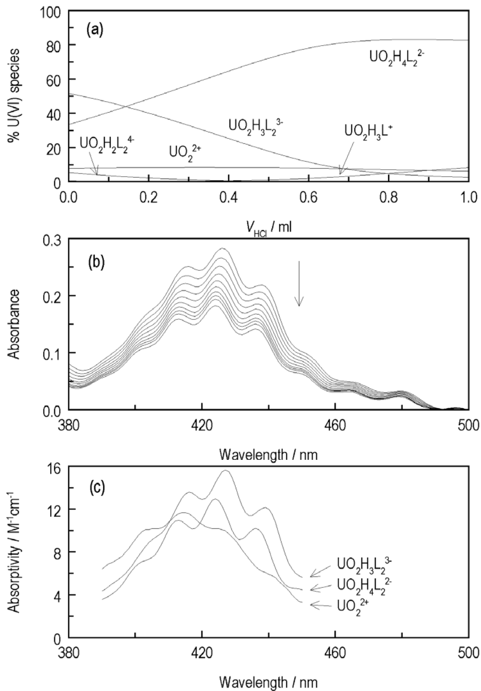
Figure 2. Spectrophotometric titrations, I = 1.0 \text{ M } (\text{CH}_3)_4\text{NCl} , t = 25^\circ\text{C} . Initial solution: 2.5 ml, C_{\text{U}} = 0.020 \text{ M} , C_{\text{HEDPA}} = 0.0367 \text{ M} , C_{\text{H}} = 0.0592 \text{ M} ; titrant: 0.0499 \text{ M HCl} . (a) Speciation of U(VI) in the titration calculated by the stability constants obtained by potentiometry (Table 2). (b) Absorption spectra (20 additions of 50 \mu\text{l} titrant per addition, the number of spectra is reduced for clarity). (c) Calculated molar absorptivities of \text{UO}_2^{2+} , \text{UO}_2\text{H}_4\text{L}_2^{2-} and \text{UO}_2\text{H}_3\text{L}_2^{3-} .
