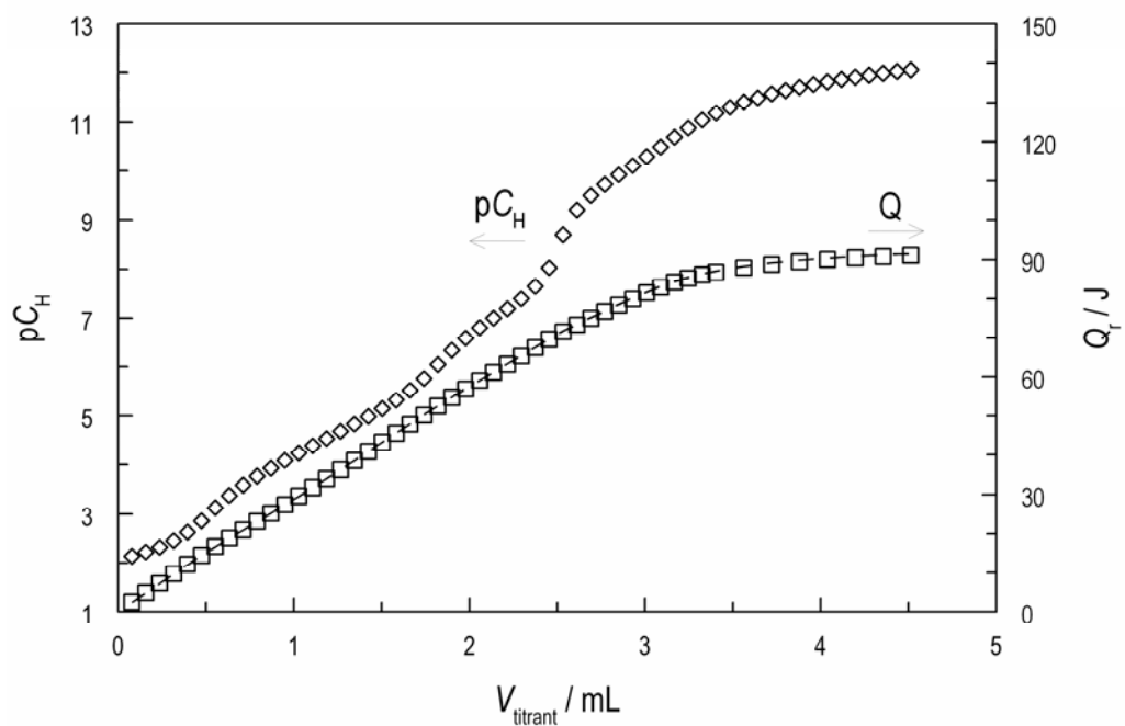
Figure 3. Calorimetric titration of U(VI)-HEDPA complexation ( I = 1.0 \text{ M } (\text{CH}_3)_4\text{NCl} , t = 25^\circ\text{C} ). Cup: 20.0 \text{ mL} , C_{\text{H}} = 81.21 \text{ mM} , C_{\text{U}} = 16.72 \text{ mM} , C_{\text{HEDPA}} = 34.26 \text{ mM} ; titrant: 0.508 \text{ M } (\text{CH}_3)_4\text{NOH} . Symbols: \diamond - -pC_{\text{H}} , \square - experimental heat of reaction ( Q_{\text{r}} ) in joule, dashed line – calculated heat of reaction.
