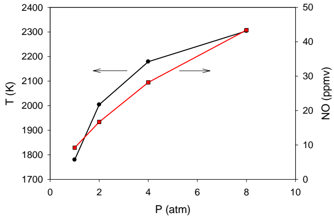
Figure 9: Peak flame temperature and NO concentration calculated with OPPDIF for 40% nitrogen dilution, and strain rate= 7000 \text{ s}^{-1} .
