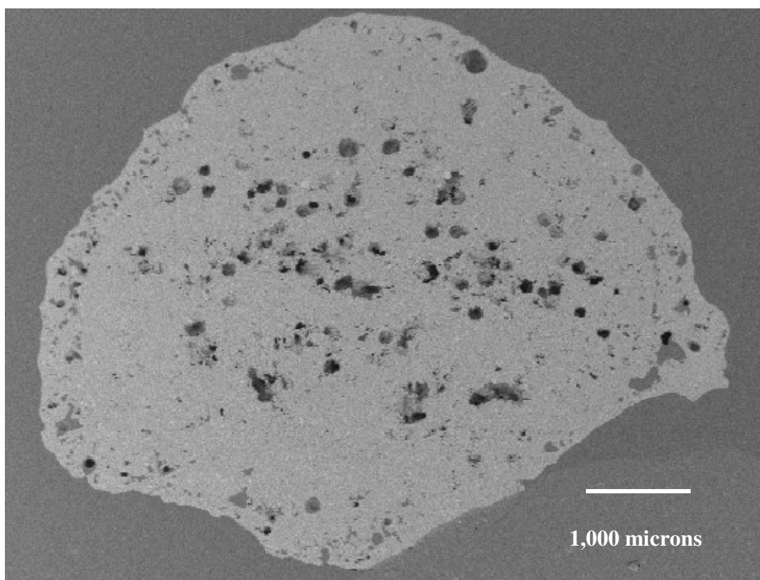
Figure 13: Backscatter electron image of used sintered bonded alumina micro-porous filter media. Figure 14 contains EDS analyses made at equi-distance locations across the center from left to right.
