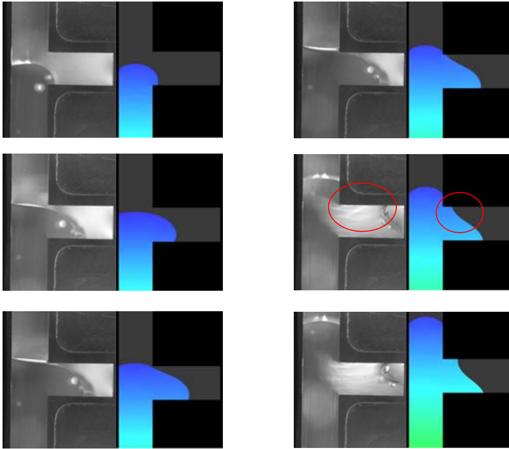
Figure 23. Representative frames from ARIA simulations (right side of each column) and visual observations (left side of each column) of the flow in Geometry 2 with H_f/H=2 (Figure 5). Experiment used the curing system and the simulation is for the elastomer only. Circled region indicates the difference between 3D and 2D as discussed in the text. Color gradations indicate pressure.
