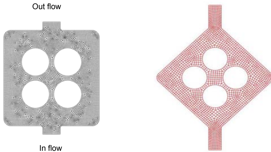
Figure 4. Typical mesh for a 2D representation of Geometries 2A and 2B.
