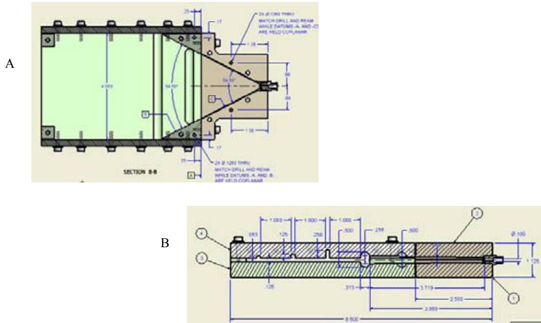
Figure 18. Two views of the apparatus used to test Geometry 2 with dimensions in inches. A. The triangular area on the right acts as a distributor. B. Region 3 is aluminum, and 4 is polycarbonate.
