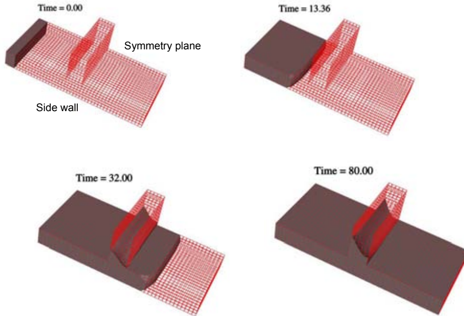
Figure 25. ARIA 3D simulation results of notch problem.
