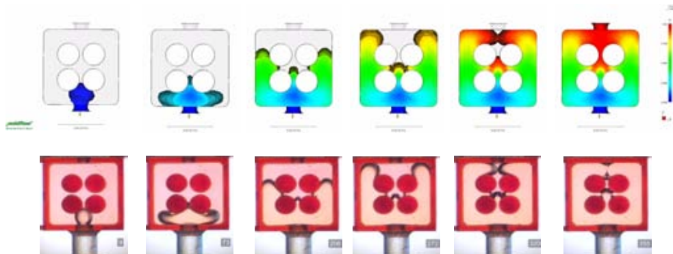
Figure 41. MOLDFLOW results compared to the experiment (Figures 33 and 36). Colors represent time to reach that point. Red areas would be the last to fill and could represent void locations.
