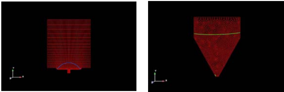
Figure 19. Flattening of flow front with a change in distributor shape predicted in a 2D GOMA calculation.
