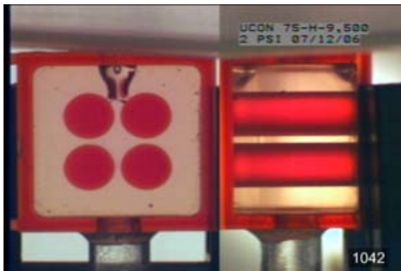
Figure 37. 3D ARIA calculation correctly shows bubbles left at exit near walls. Left, views of the experiment (left from front, right from side) as liquid knit lines meet and as liquid begins to leave the top. Right, corresponding frames from simulation.
