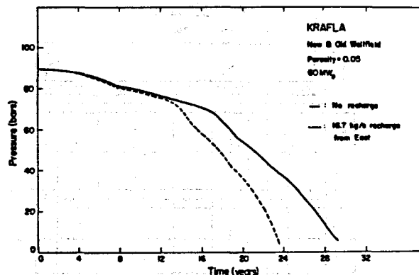
Figure 6. Pressure decline versus time in the Krafla wellfield for a power production of 60 MW e .
