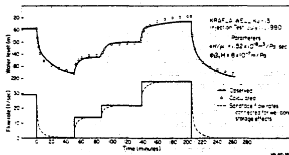
Figure 3. Comparison between observed and calculated water level data for injection test of well KJ-13.
