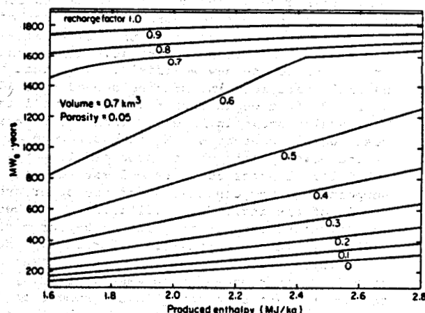
Figure 5. Lumped model-generating capacity of the old wellfield.
