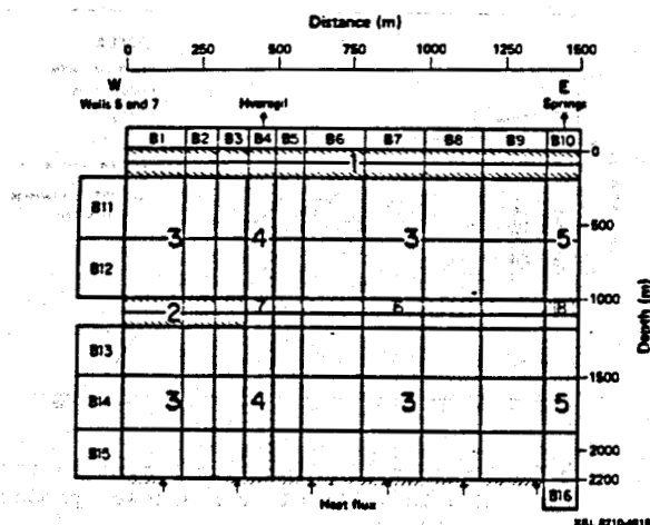
Figure 4. Grid blocks and different reservoir zones used in the natural-state modeling.
