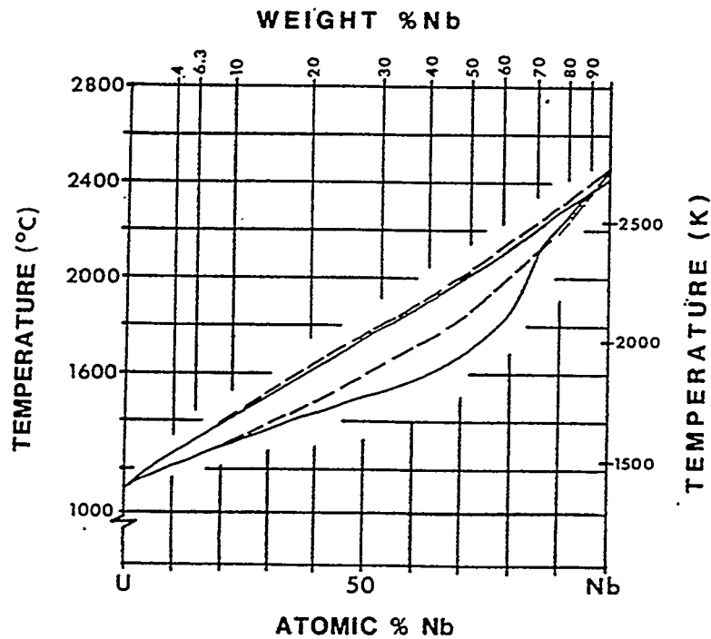
Figure 3: U-Nb binary phase diagram.
