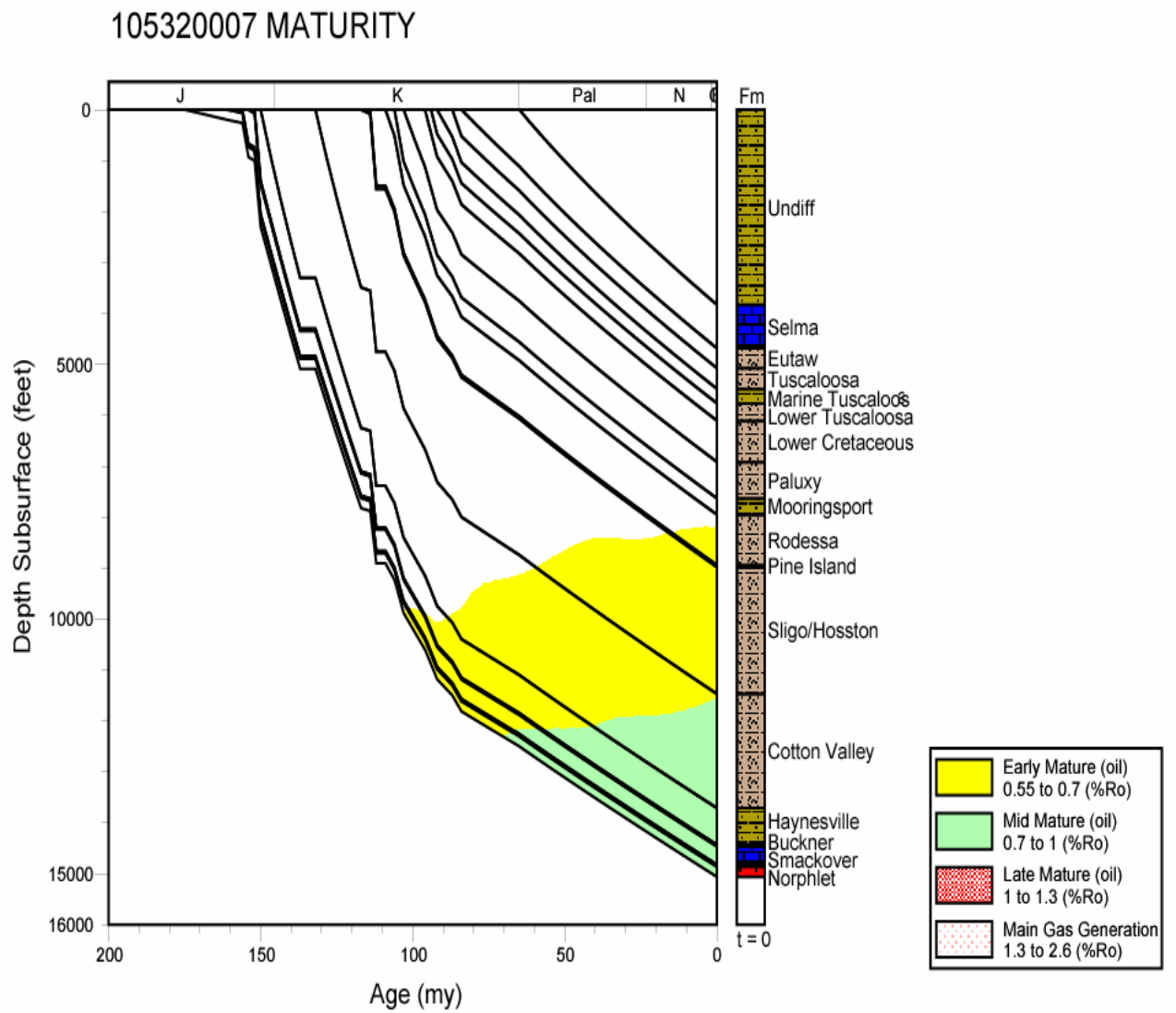
Figure 83. Conecuh Subbasin, thermal maturation history profile.
