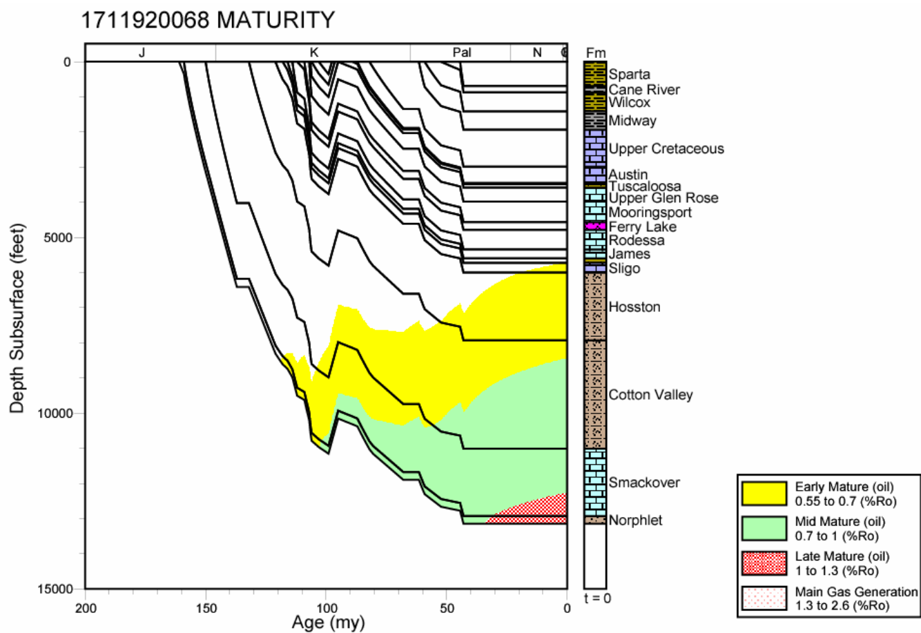
Figure 60. Updip North Louisiana Salt Basin, thermal maturation history profile, modified from Mancini et al. (2006).
