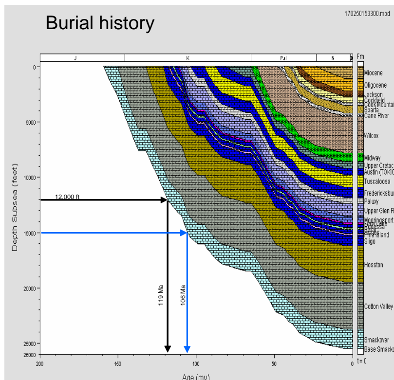
Figure 90. Modeling of top of Smackover burial By R. Barnaby.
