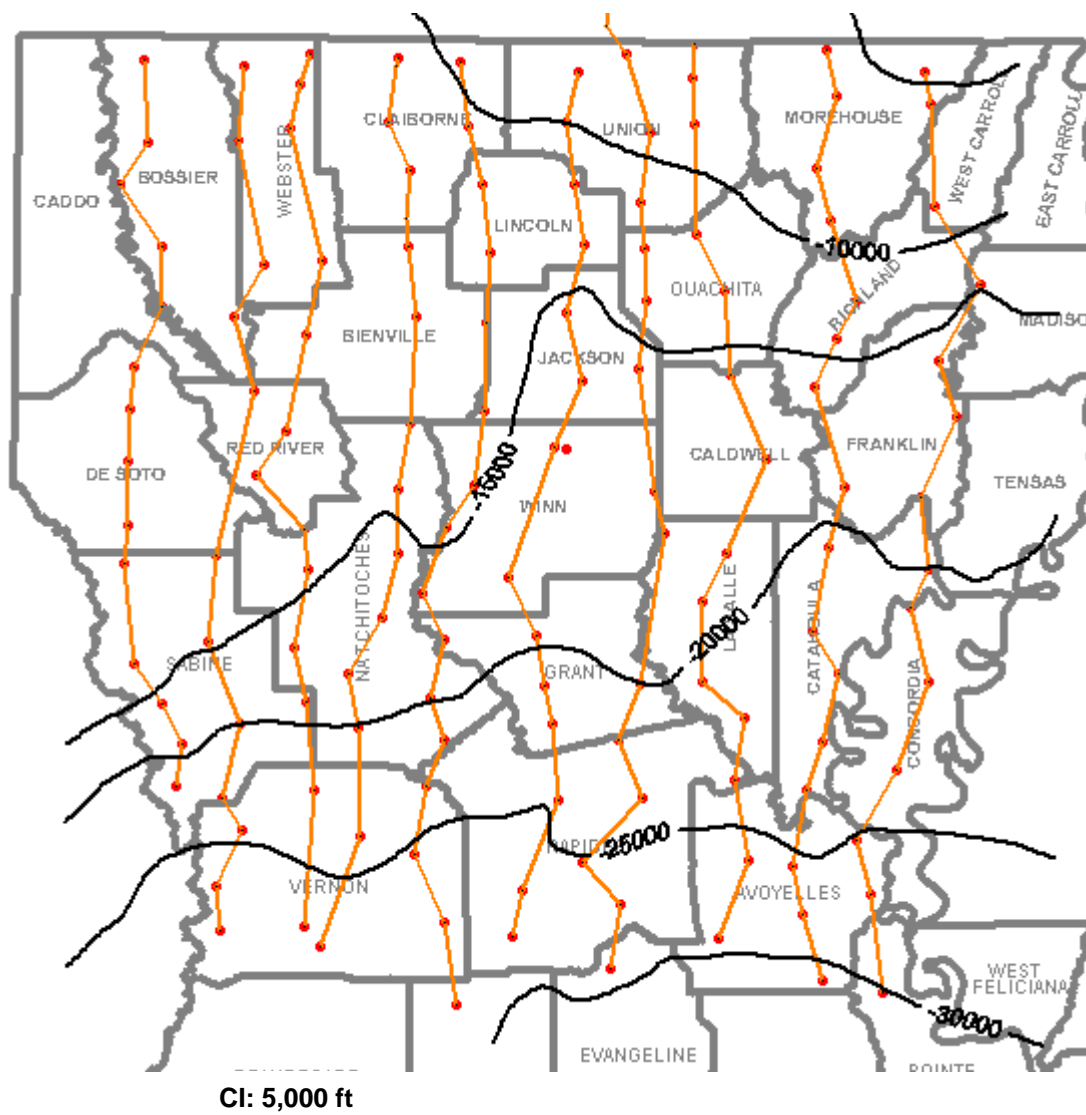
Figure 91. Depth of top of Smackover at present day. By R. Barnaby.
