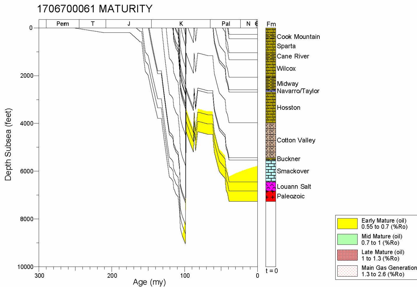
Figure 57. Monroe Uplift, North Louisiana Salt Basin, thermal maturation history profile, modified from Mancini et al. (2006).
