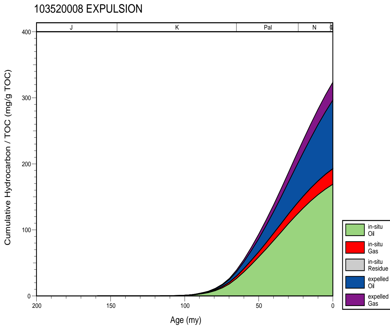
Figure 84. Conecuh Subbasin, hydrocarbon expulsion plot.
