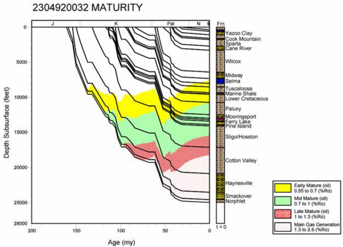
Figure 74. Downdip Mississippi Interior Salt Basin, thermal maturation history profile, modified from Mancini et al. (2003).
