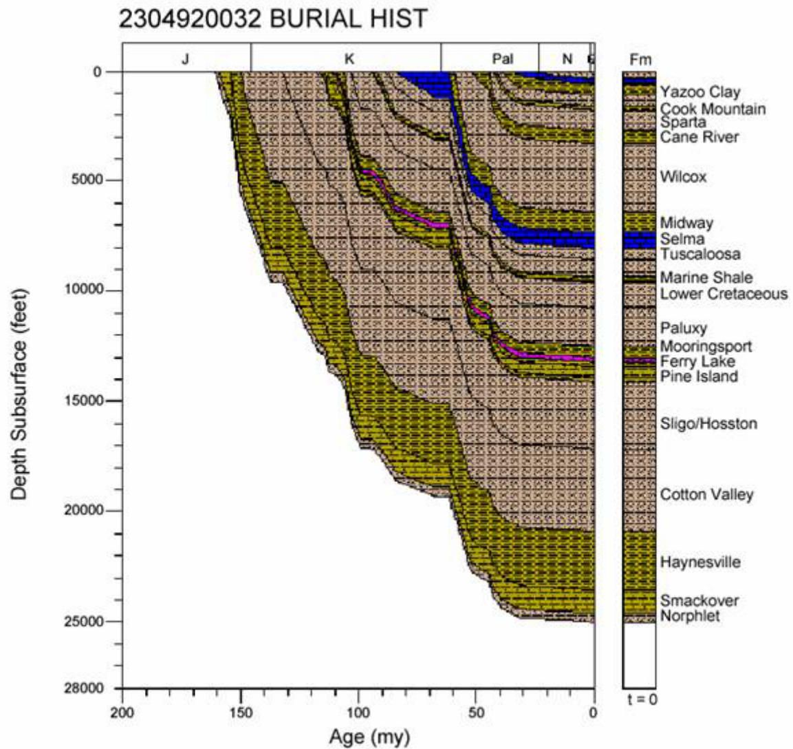
Figure 73. Downdip Mississippi Interior Salt Basin, burial history profile, modified from Mancini et al. (2003).
