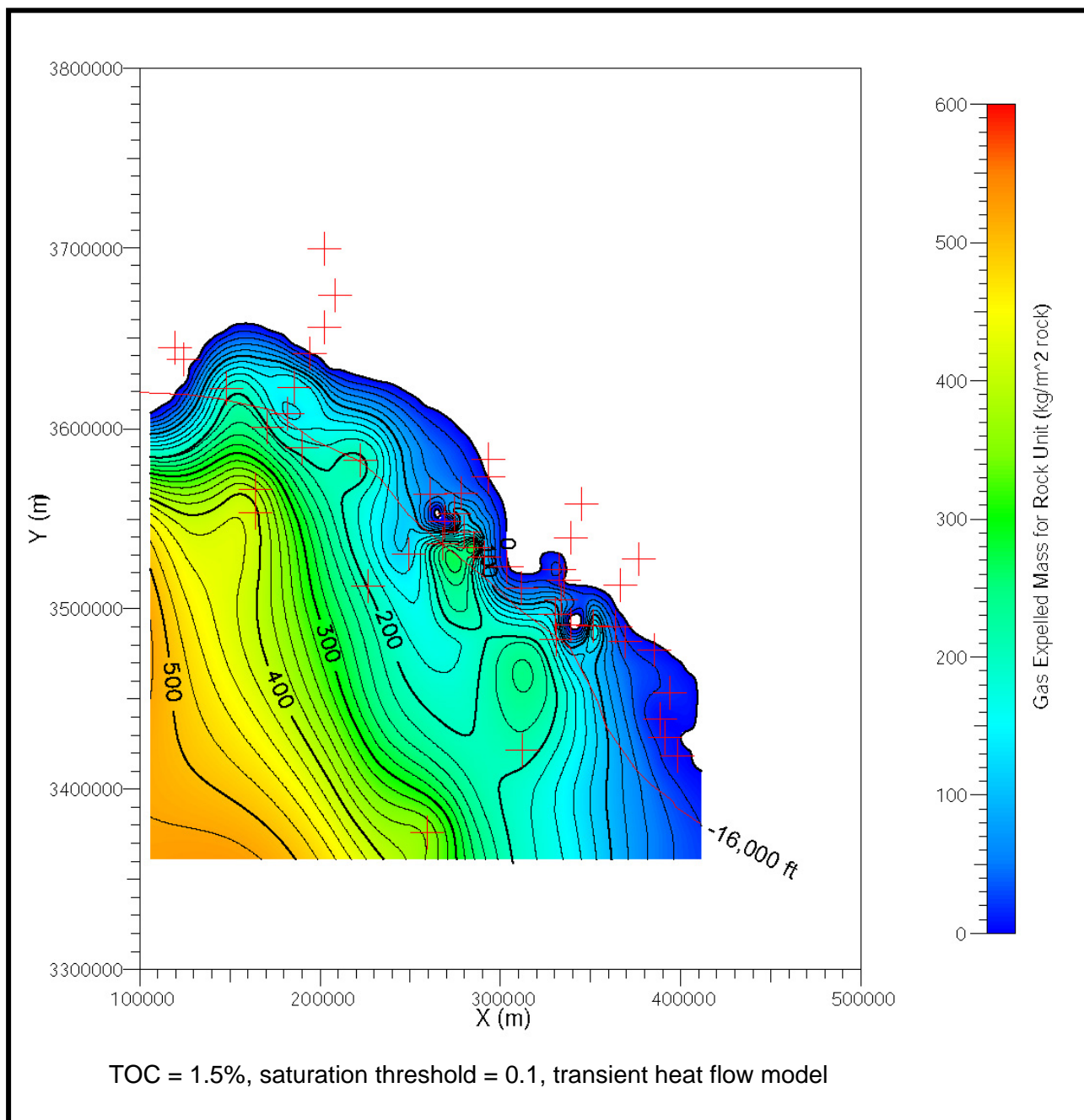
Figure 103. Platte River software model of total expelled gas from the Smackover in the Mississippi Interior Salt Basin. By P. Li.
