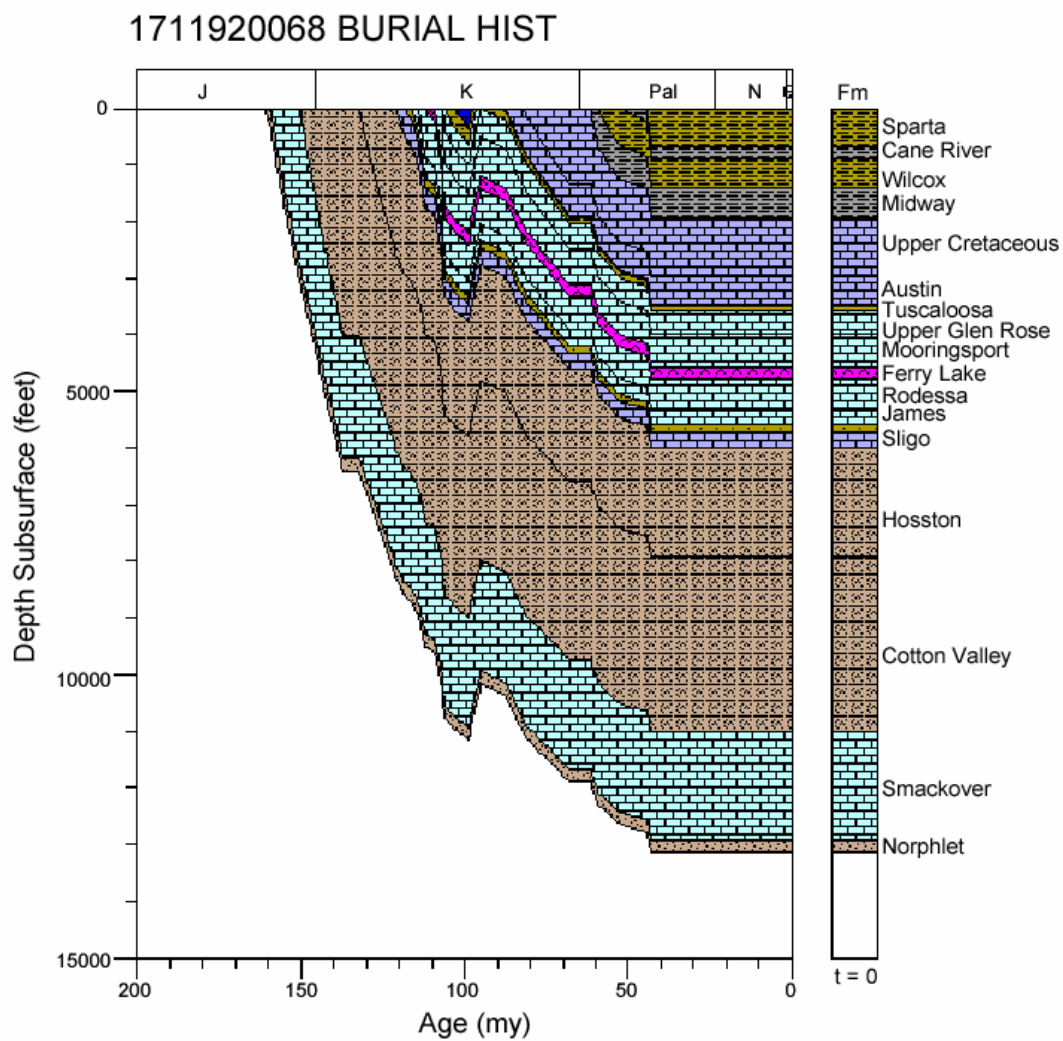
Figure 59. Updip North Louisiana Salt Basin, burial history profile, modified from Mancini et al. (2006).
