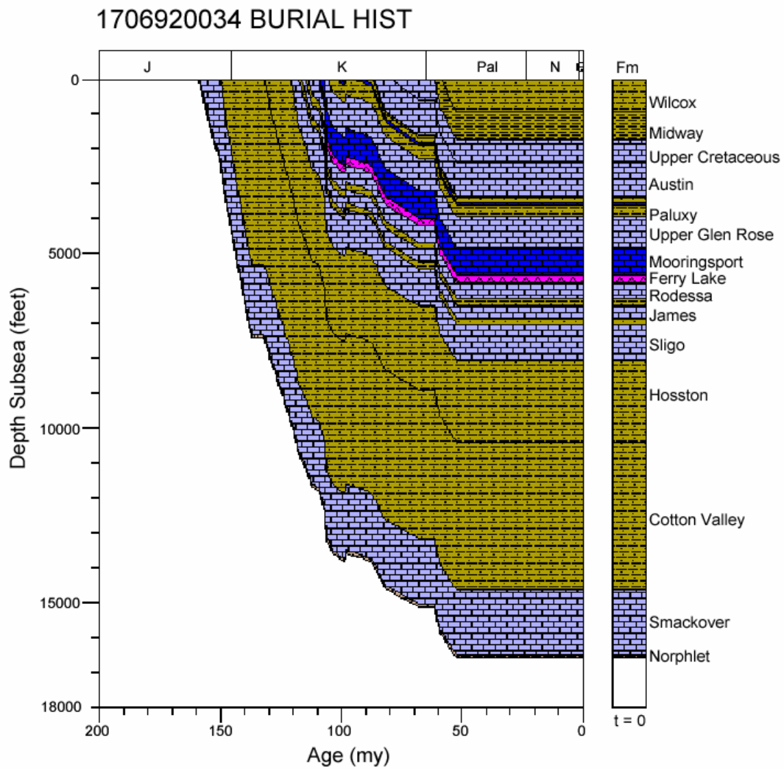
Figure 62. Dwindip North Louisiana Salt Basin, burial history profile, modified from Mancini et al. (2006).
