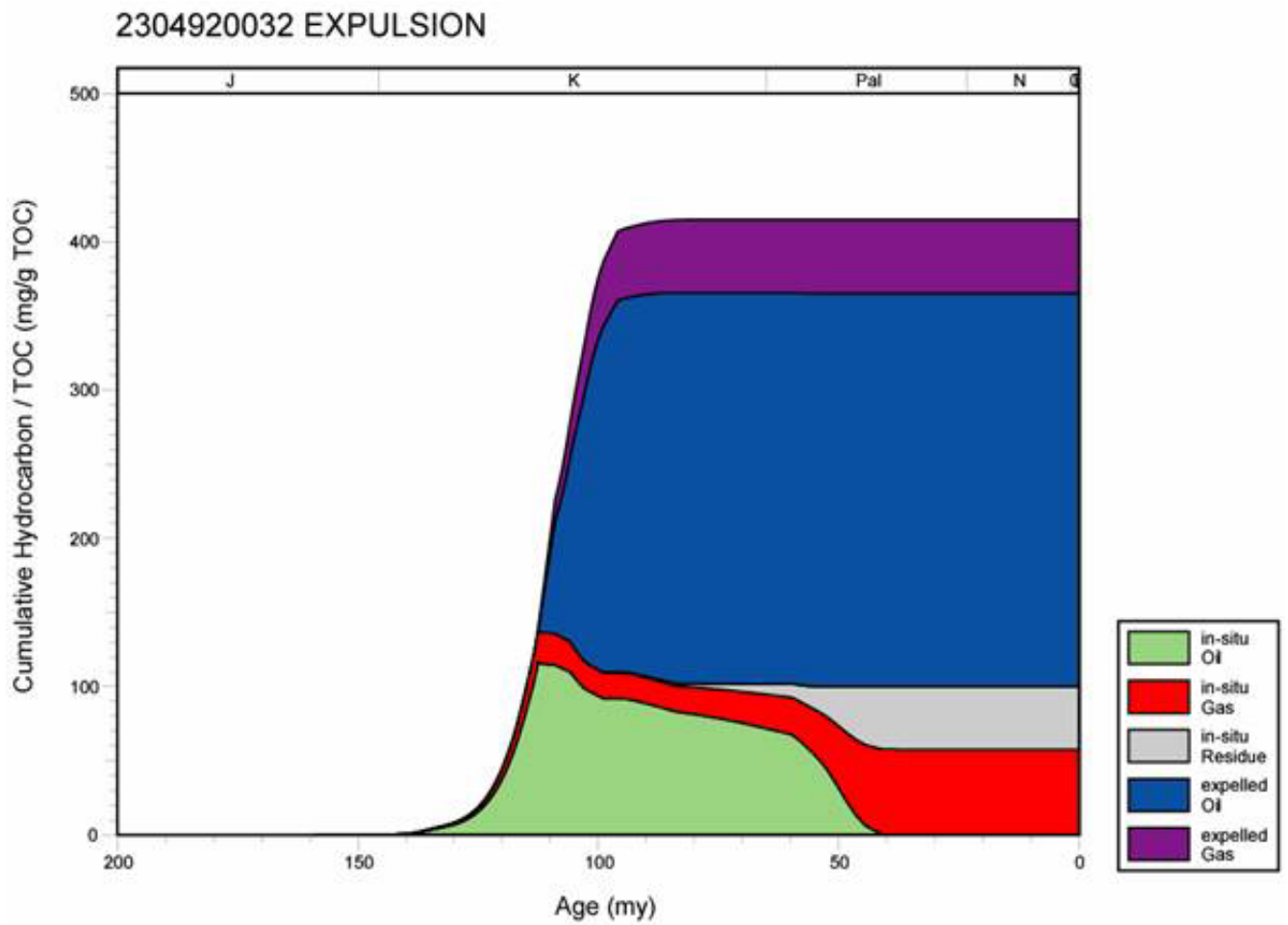
Figure 75. Dwindip Mississippi Interior Salt Basin, hydrocarbon expulsion plot, modified from Mancini et al. (2003).
