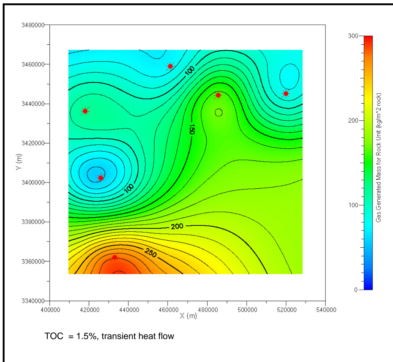
Figure 98. Platte River software model of total generated gas from the Smackover in the Conecuh Subbasin. By P. Li.
