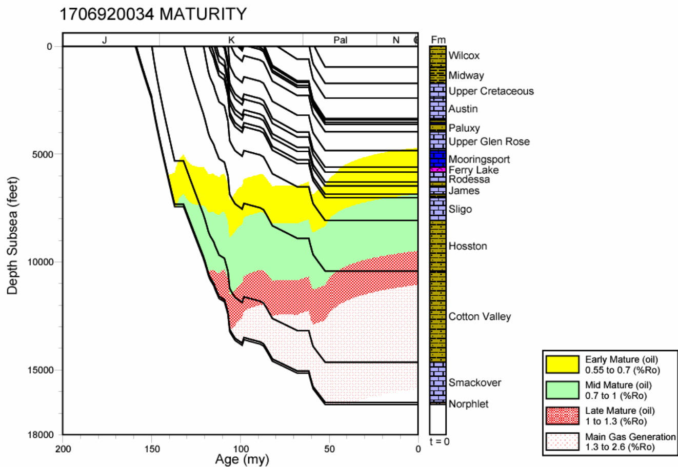
Figure 63. Downdip North Louisiana Salt Basin, thermal maturation history profile, modified from Mancini et al. (2006).
