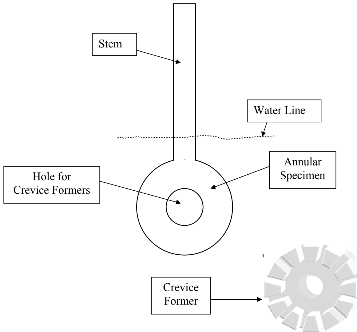
FIGURE 1 – Multiple Crevice Assembly (MCA) Specimen and Crevice Former (CF).
