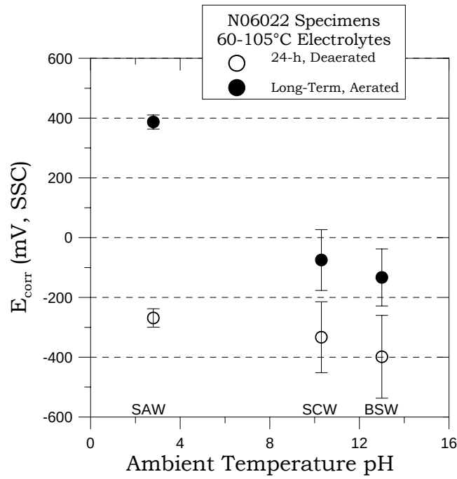
FIGURE 2 – Corrosion potential ( E_{\text{corr}} ) for Alloy 22 in multi-ionic electrolytes
