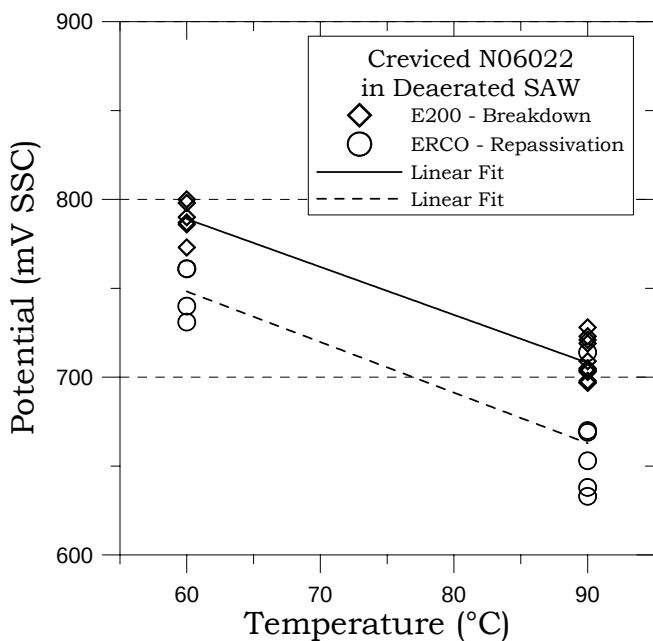
FIGURE 11 – Breakdown and repassivation potentials for Alloy 22 in SAW solution. None of the specimens suffered crevice corrosion
