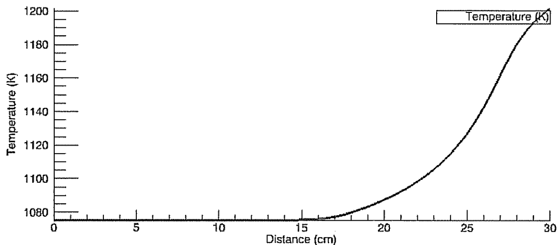
Figure 5.12. Temperature corresponding to the case in Figure 11 as a function of distance
