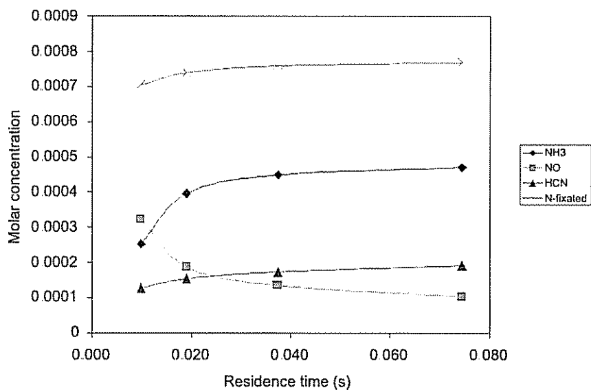
Figure 7.25. Molar concentration of fixated nitrogen.
