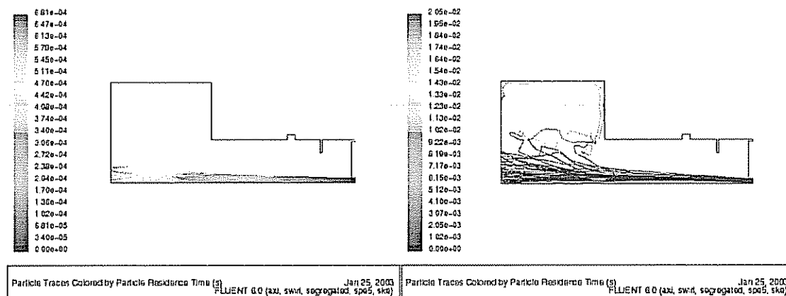
Figure 7.17. Stochastic paths for initial radial velocities of (a) 0 m/s, and (b) 10 m/s
