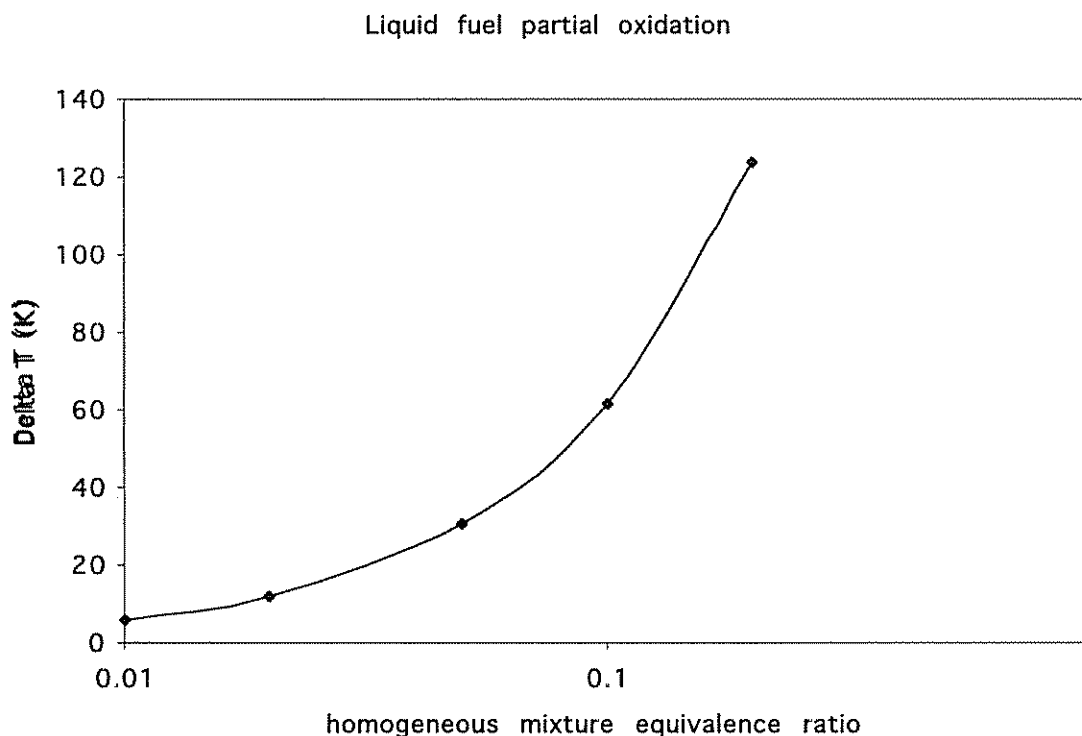
Figure 6.1 Temperature excursion of the gaseous charge to the cylinder as a function of the equivalence ratio of the air/reformate fuel mixture.
