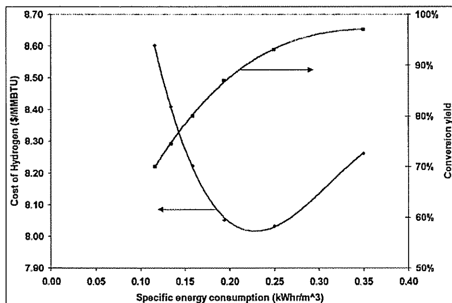
Figure 9 Methane yield and cost of hydrogen as a function of the specific energy, for 571 m³=h plant capacity
