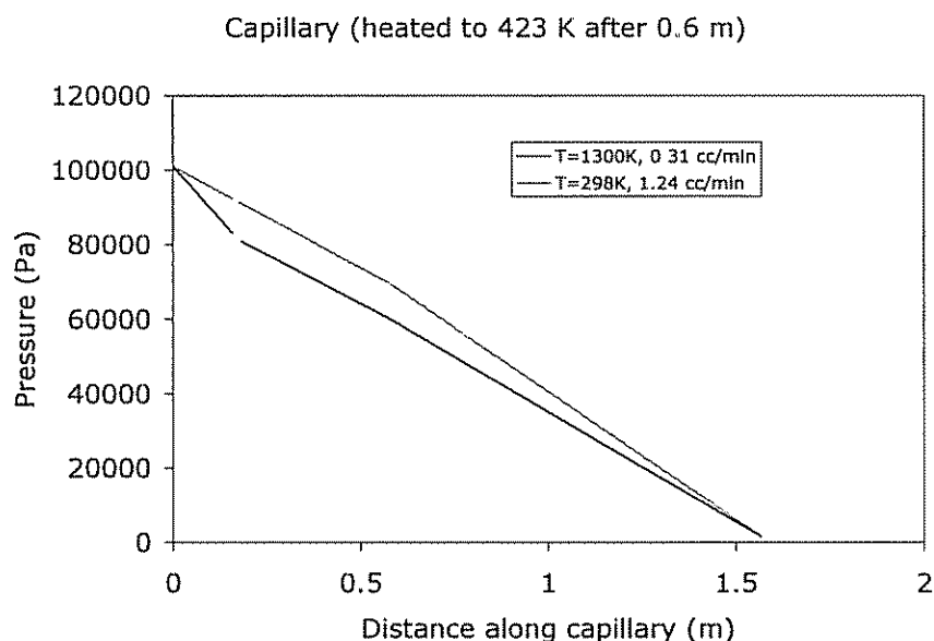
Figure 2.9. Pressure drop as a function of the distance along the capillary
