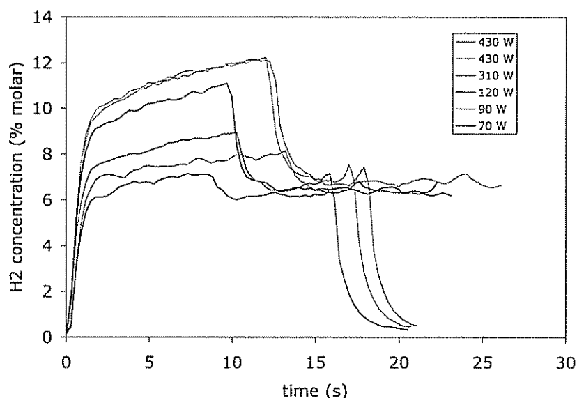
Figure 9.4. H_2 concentration for O/C \sim 2.2 for several values of power.
