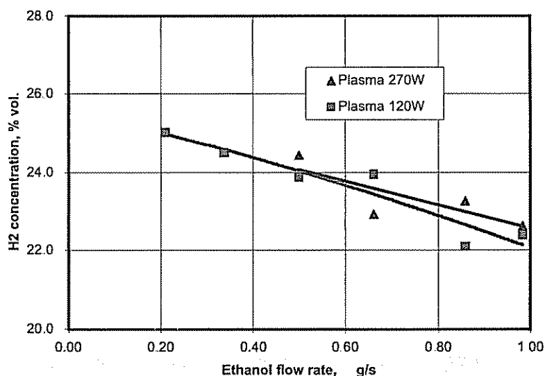
Figure 4.4. Hydrogen concentration in dry gas for ethanol reforming, as a function of flow rates, for O/C \sim 1.2
