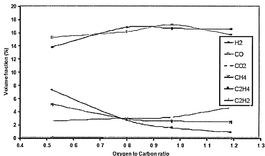
Figure 8.33. Composition of the reformat as a function of oxygen to carbon ratio for diesel fuel.
