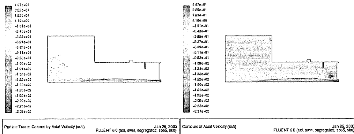
Figure 7.16. Axial velocity (a) of droplets along their path (b) of continuous media
