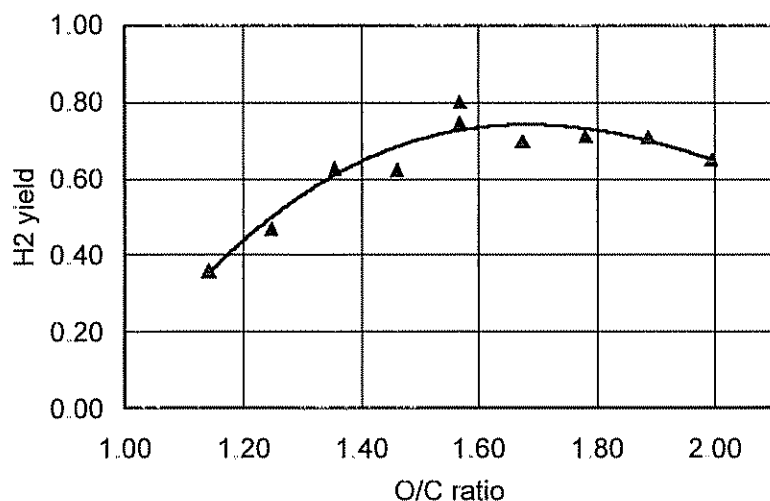
Figure 4. Hydrogen yield for the plasma-catalytic reforming of ethanol vs. O/C ratio
