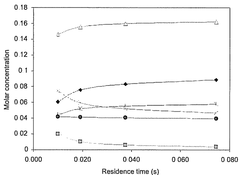
Figure 7.24. Molar concentration of major components as a function of the residence time.
