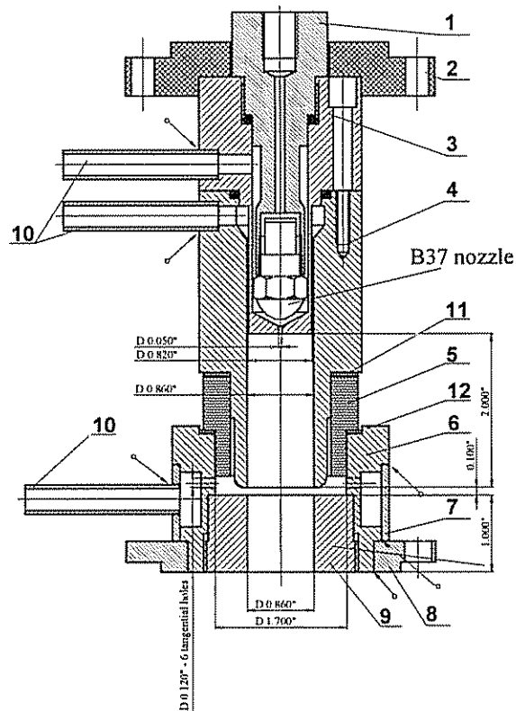
Figure 2. Detailed schematics of plasmatron
