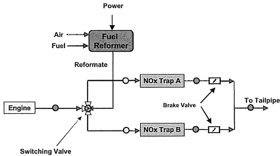
Figure 4.5. Test set-up for hydrogen assisted NO x traps
