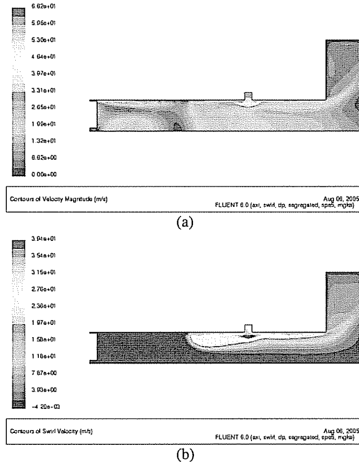
Figure 7.5. Same as Figure 2 but for case of methane through swirl port.
