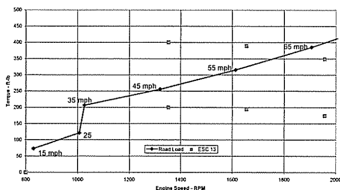
Figure 4.7. Bus Road Load vs ESC 13 mode
