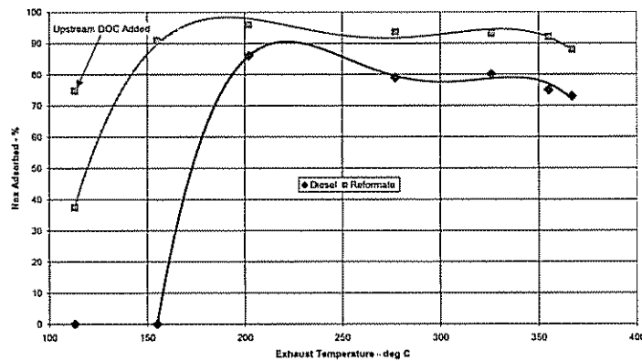
Figure 4.8. NO x adsorption comparison. Bus Road Load, at same fuel penalty (reformate vs diesel)
