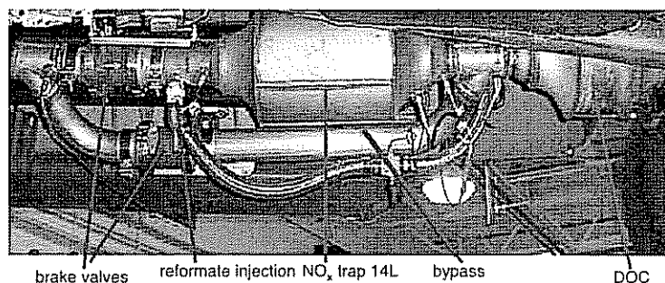
Figure 4.13. F250 hydrogen assisted \text{NO}_x trap installation
