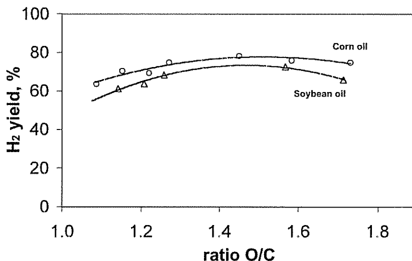
Figure 4.3. Hydrogen yield as a function of the \text{O/C} ratio, for corn and soybean oils
