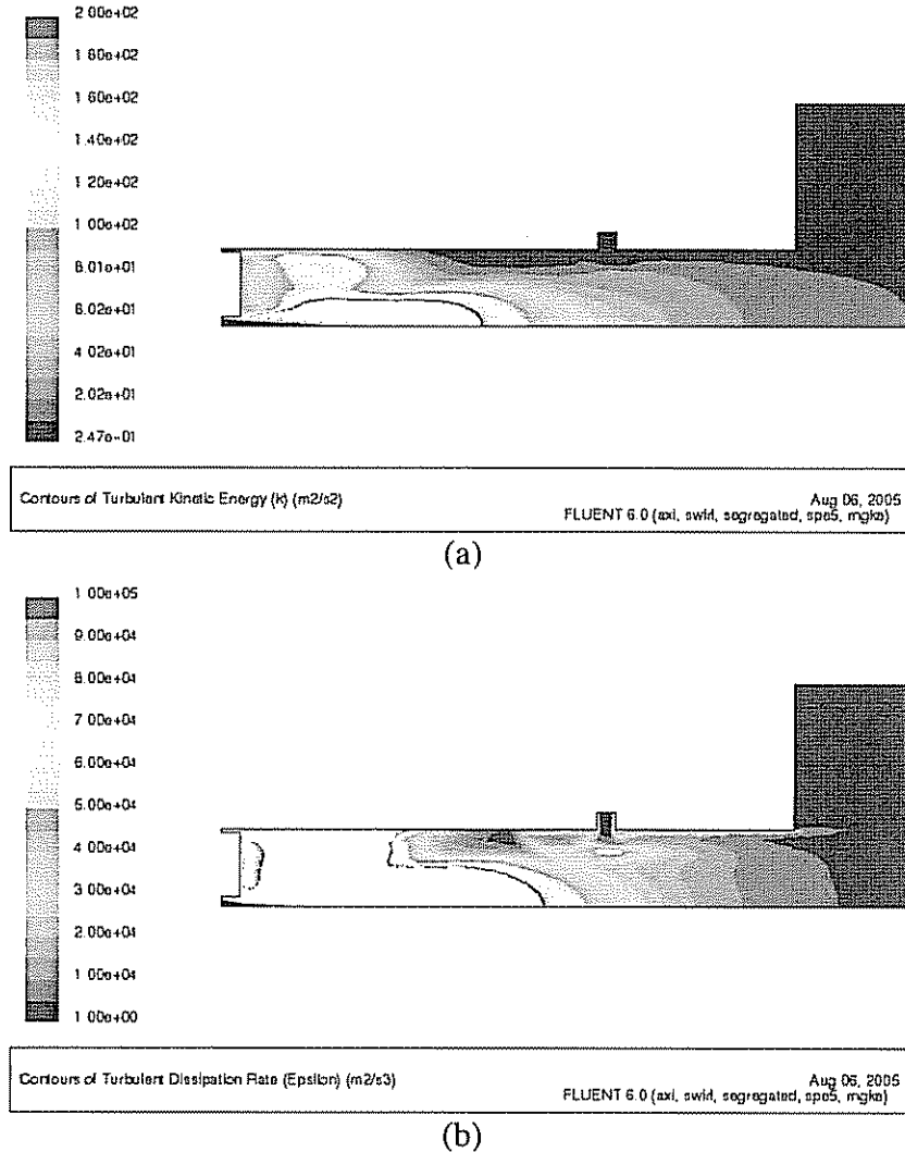
Figure 7.2. Contours of constant (a) k , turbulent kinetic energy; (b) \epsilon , dissipation rate
