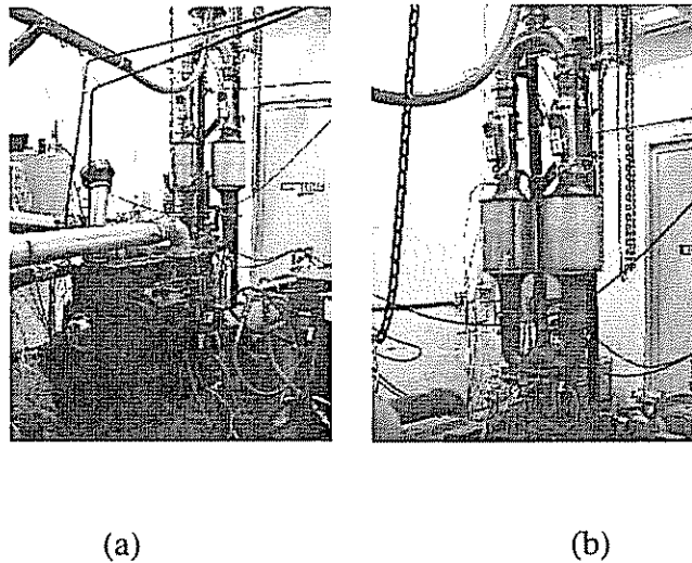
Figure 4.6. Test cell installation of hydrogen assisted NO x traps: a) Cummins engine; b) dual leg (14 liter/leg) traps and switching valve
