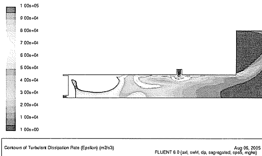
Figure 7.6. Same as Figure 7.2 but for methane injected through the swirl port.
