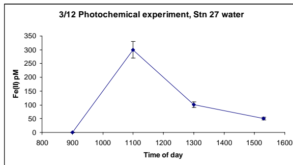
Figure 4. Shipboard study of the photo-production of Fe(II) in oligotrophic Drake passage waters.
