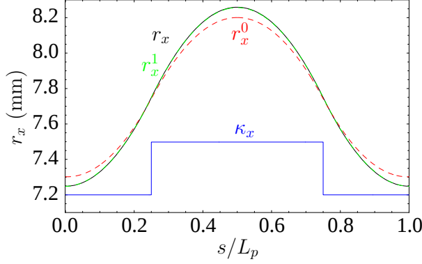
FIG. 4: (Color) Converged matched envelope solution (black) r_x = r_y for solenoidal focusing and the first (seed) second iterations r_x^0 (red) and r_x^1 (green). System parameters are L_p = 0.5 m, \eta = 0.5 , \sigma_0 = 80^\circ , \varepsilon = 50 mm-mrad, and \sigma/\sigma_0 = 0.3 .
