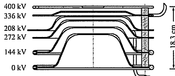
Figure 1. Side view of the electrodes used in the Full Gradient Experiment. Electric Field between the 2 nd and 3 rd cup was 100 kV/cm.
