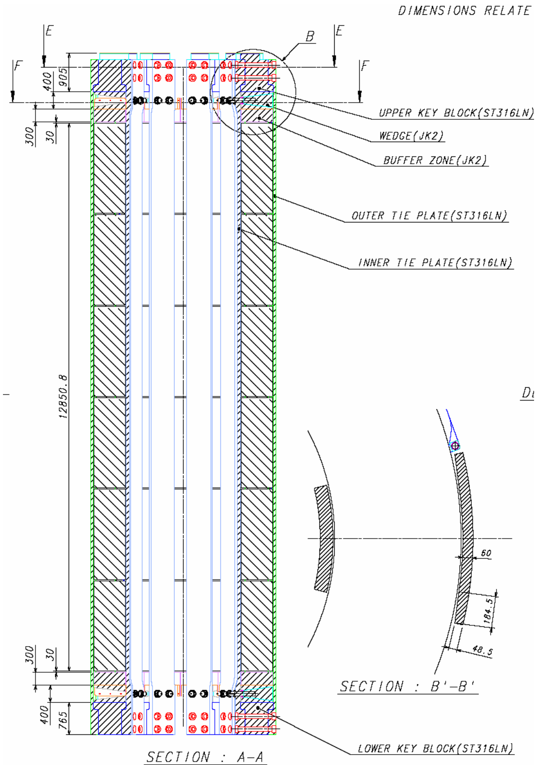
Fig. 1. Prestress structure
