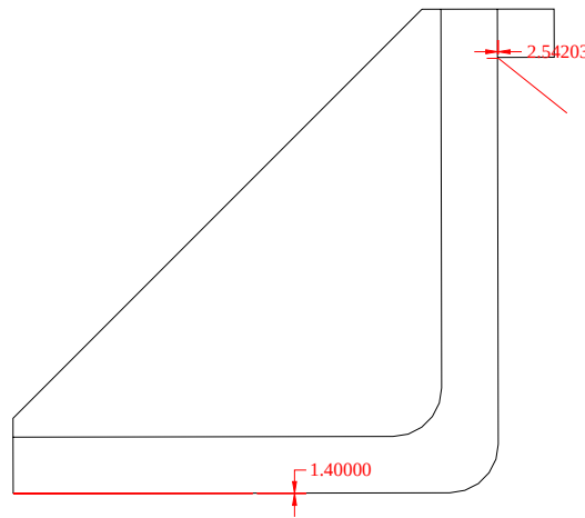
Fig. 3.1.4 mm DZ displacement of the bracket at the foundation causes 2.5 mm DR displacement at the top of the bracket.
