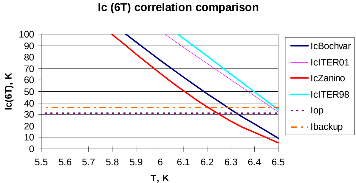
Fig. 1. j_c(T) correlations for NbTi at 6 T
