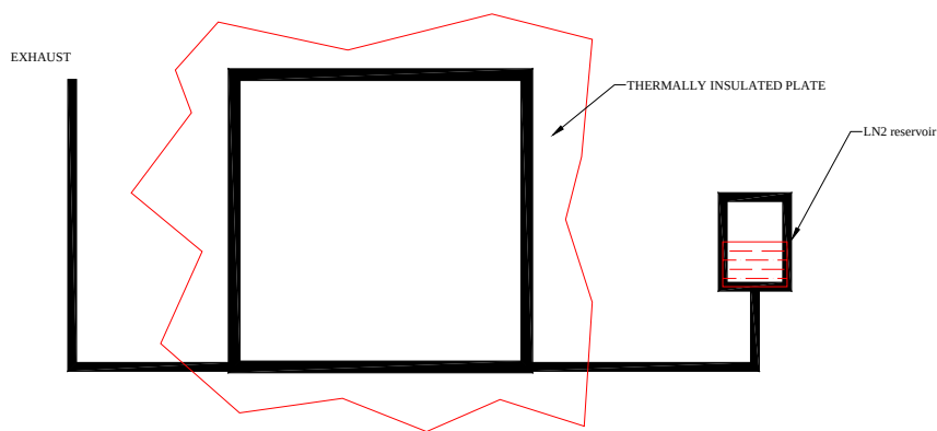
Fig. 5. Test arrangement
