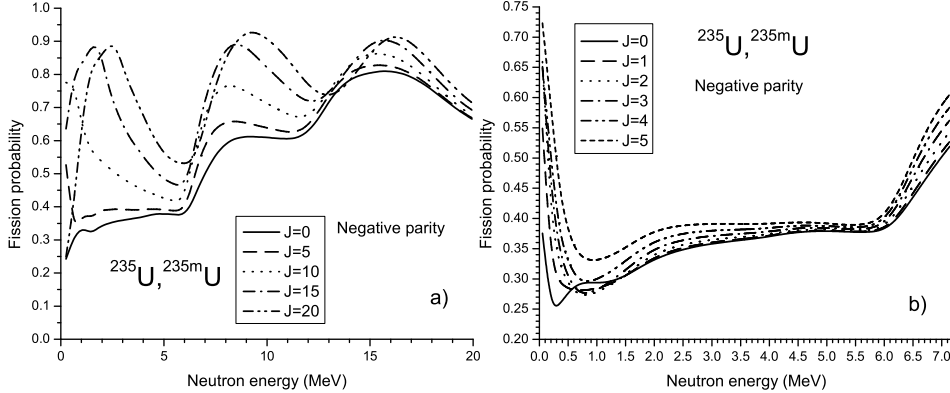
Figure 2: Calculated branching ratios G_{fission}^{CN}(E_{ex}, J, \pi) for fission of ^{236}\text{U} (following n + ^{235}\text{U} ). a) Results are shown for negative parity states with total angular momenta J = 0, 5, 10, 15, 20 in the compound nucleus ^{236}\text{U}^* . b) Results for negative parity states with small total angular momenta, J = 0, 1, 2, 3, 4, 5 .
