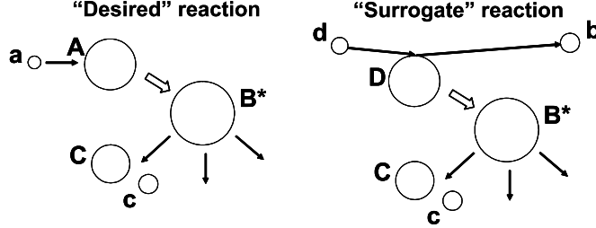
Figure 1: Surrogate reaction mechanism. The first step of the desired reaction, a + A \rightarrow B^* \rightarrow c + C , is replaced by an alternative (“Surrogate”) reaction, d + D \rightarrow b + B^* , that populates the same compound nucleus, B^* . The subsequent decay of the compound nucleus into the relevant channel, B^* \rightarrow c + C , is measured and used to extract the desired cross section.
