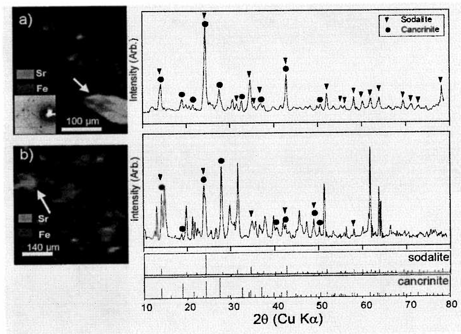
Figure 4. Microfocused synchrotron X-ray fluorescence maps and micro-diffraction patterns of Hanford (WA) soil particles (HC) after reaction for 374 d with caustic synthetic tank waste leachate (top), and the same sample after extraction with acid-ammonium oxalate extraction (bottom). Secondary sodalite and cancrinite that sequestered contaminant Sr formed as products of reaction of leachate with soil minerals. Diffractograms show the persistence of the secondary sodalite and cancrinite phases after extraction treatment, which does not remove sequestered contaminant Sr.
