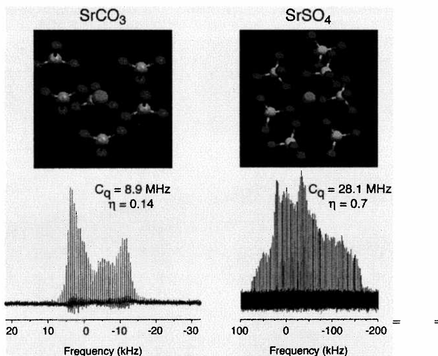
Figure 5. ^{87}\text{Sr} QCPMG NMR signals from two model strontium compounds exhibit the strong dependence of quadrupolar interaction parameters (the quadrupolar coupling constant, C_q , and the quadrupolar asymmetry parameter, \eta ) on the local environment of the strontium cations. In the \text{SrCO}_3 structure, the cation is coordinated by nine oxygen atoms, while in the \text{SrSO}_4 structure the strontium sits in a highly asymmetric site with twelve neighboring oxygen atoms.
